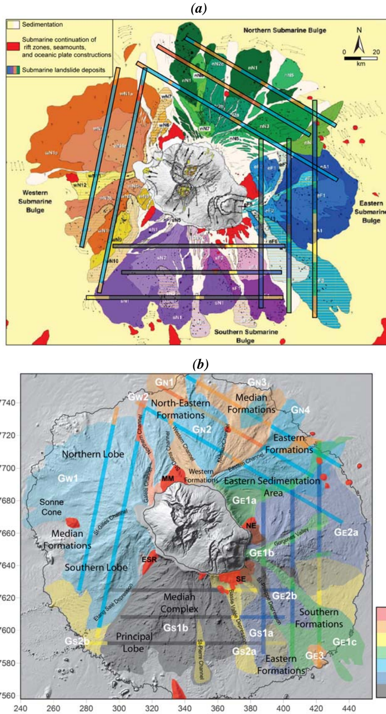
Figure 13: a) Geological map of the submarine flanks of La Réunion, from Oehler et al. (2008); b) Inferred 2D density distribution at the surface of the submarine flanks, based on the modelling along different profiles and the correlations with the geological units defined by Oehler et al. (2008). The labels (e.g. GE) refer to the gravity (G) units of North (N), East (E), South (S) and West (W). The numbers and their letter index (e.g. 1b) specify units and sub-units.
