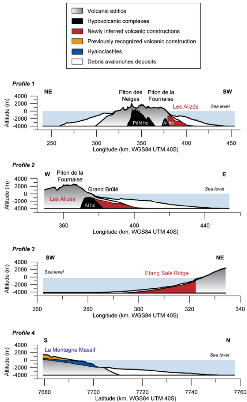
Figure 15: Slices from the 3D model presented in figure 14 along the main structures discussed in the text. The submarine volcanic constructions presented in this study (i.e. Les Alizés volcano, Etang Salé Ridge and La Montagne Massif) are underlined. The hypovolcanic complexes of Les Alizés volcano (Al hc) and Piton des Neiges (PdN hc) are described in a separate paper (Gailler and Lénat, submitted in JVGR).
