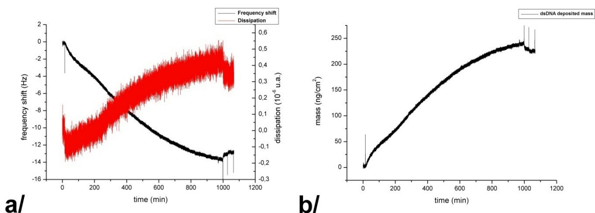
Figure 37 : (a) Frequency shift of QCM crystal and dissipation monitored after injection of double stranded DNA ( \text{NH}_2 - C7T5 hybridizes with \text{A}_5\text{G}_7 ) (b) calculation of mass deposited according to the frequency shift from the Sauerbrey equation.
