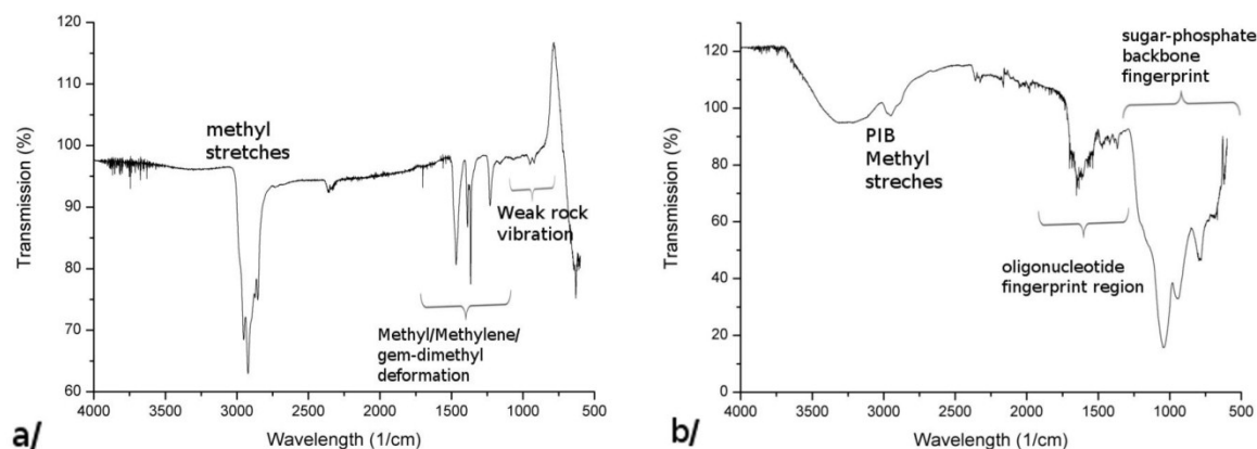
Figure 22: FTIR spectra of (a) Amino-modified PIB and (b) \text{PIB}_{31}\text{-G}_7\text{A}_5 . Both spectra were recorded on air background. Most significant regions are highlighted to provide the fingerprint of the polymer-modified oligonucleotide.
