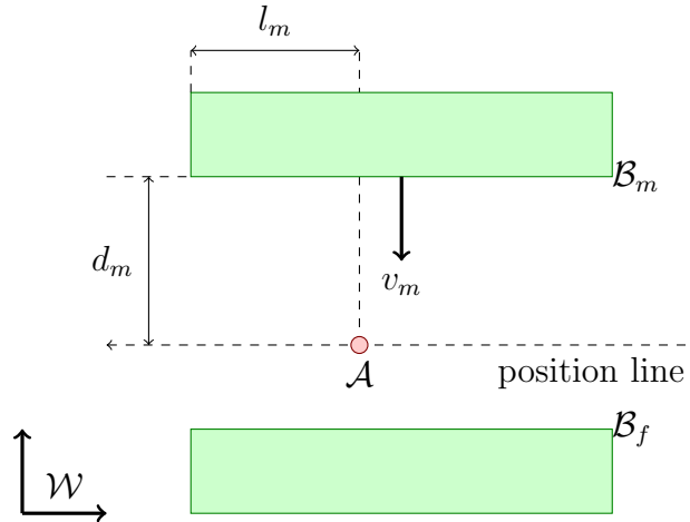
Figure 2.1: Compactor scenario.
