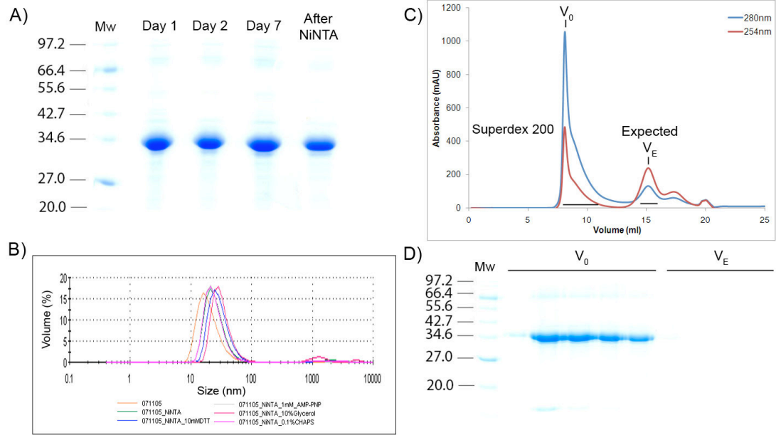
FIGURE 4.13: REFOLDING OF IKKB 1-275.
