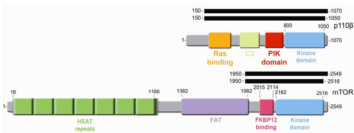
FIGURE 5.4: TRUNCATION LIBRARY ENTRY CONSTRUCTS MAPPED ONTO 110B AND mTOR
