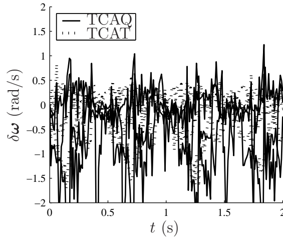
Figure 8.16: Errors on the angular velocity estimates
