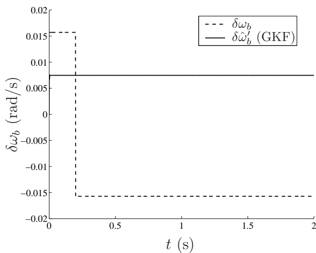
Figure 9.12: Estimates of the bias errors on the angular velocity
