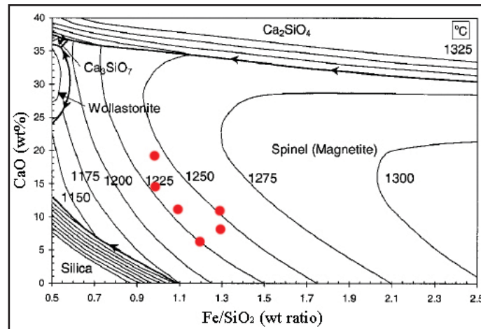
Figure 6.42 - SEM-EDS analyses of slag matrices plotted on a Flogen binary chart for slag system at a 10^{-8} ppO_2 and with 7wt% Al 2 O 3 . Image adapted from Kongoli & Yazawa 2001: Figure 11.
