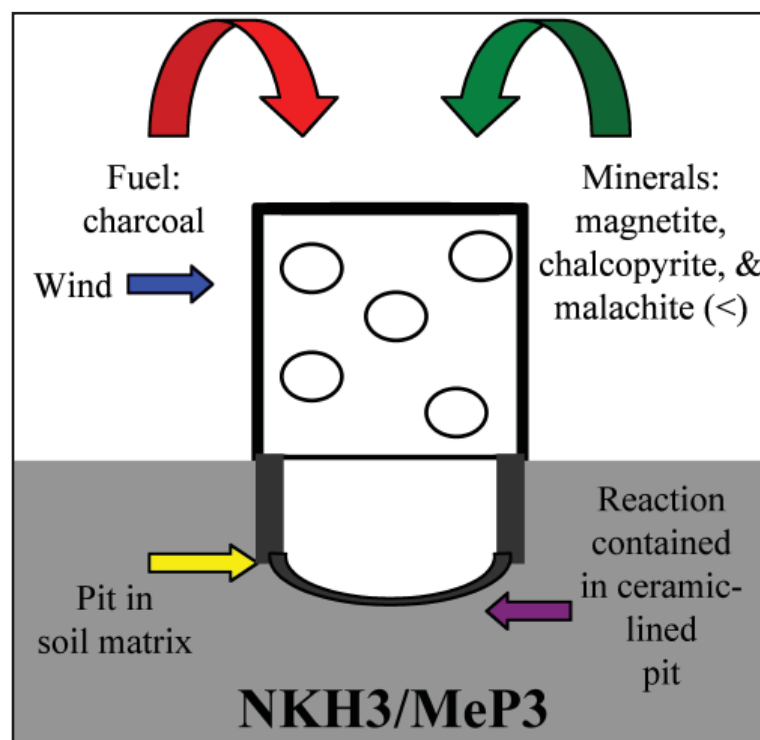
Figure 6.43 - Schematic technological reconstruction for copper smelting technique at later Iron Age Nil Kham Haeng, prior to experimental testing. Image: author.
