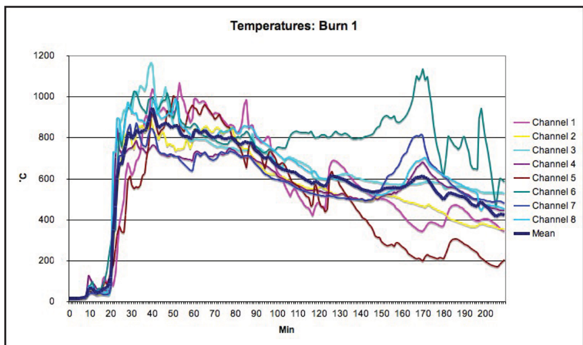
Figure 7.12 - Graph of temperature data for Burn 1. Image: author.
