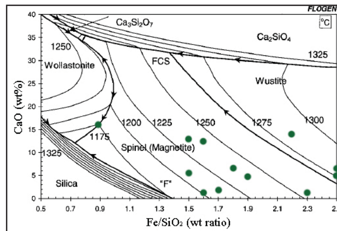
Figure 5.35 - SEM-EDS analyses of olivine phases plotted on a Floggen binary chart for a slag system at a 10^{-8} ppO 2 and with 1wt% MgO. Image adapted from Kongoli & Yazawa 2001: Figure 15.
