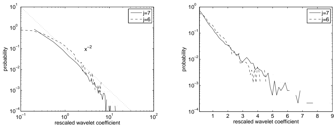
Figure V.4.6: Probability distribution functions of the wavelet coefficients of \omega_z at scales j_{xz} = 6 and 7 estimated by histograms using 50 bins at two different wall distances, y^+ = 30 (left) and y^+ = 153 (right).
