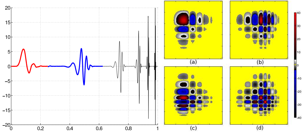
Figure III.1.1: Daubechies 6 wavelet family. Left, bold red: scaling function \varphi at scale j = 5 . Left, bold blue: wavelet \psi at scale j = 5 . Left, thin black, from left to right: wavelets at scales 6, 7, 8 and 9. Right : (a) 2D scaling function \varphi(x_1)\varphi(x_2) . (b) first 2D wavelet \psi(x_1)\varphi(x_2) . (c) second 2D wavelet \varphi(x_1)\psi(x_2) . (d) third 2D wavelet \psi(x_1)\psi(x_2) .
