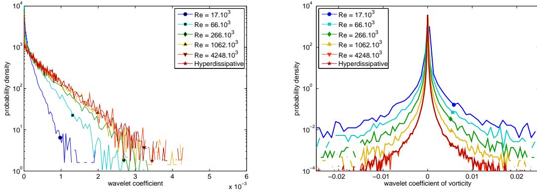
Figure V.3.4: Wavelet coefficients PDFs in the direction \mu = 1 for the reference solutions at t = 50 , for varying Reynolds number. Left: scale-wise PDF at j = 7 . Right: global PDF of wavelet coefficients.
