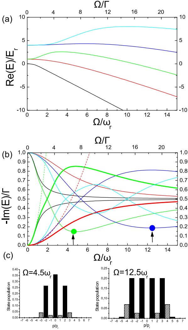
Fig. 7: (Colour on-line) Real (a) and imaginary parts (solid lines) (b) of the eigenvalues of the effective Hamiltonian given by the expression 3, with n_{\text{max}} = 8 and q = 0 , as a function of \Omega . Only the eigenvalues corresponding to eigenstates for which the momentum |p| \leq 2\hbar k at \Omega = 0 are shown. In (b) the dashed red and black lines correspond, respectively, to \Gamma_{\text{off}} and \Gamma'(\delta + \omega_r) , whereas the dash-dotted line corresponds to \Gamma_C in units of \Gamma (see text). At \Omega \approx 4.5\omega_r and \Omega \approx 12.5\omega_r long-lived states appear, pointed out by arrows and coloured circles. The histograms in (c) represent the populations of the relevant momentum states in the ground state (plain bars) and in the excited state (dashed bars).
