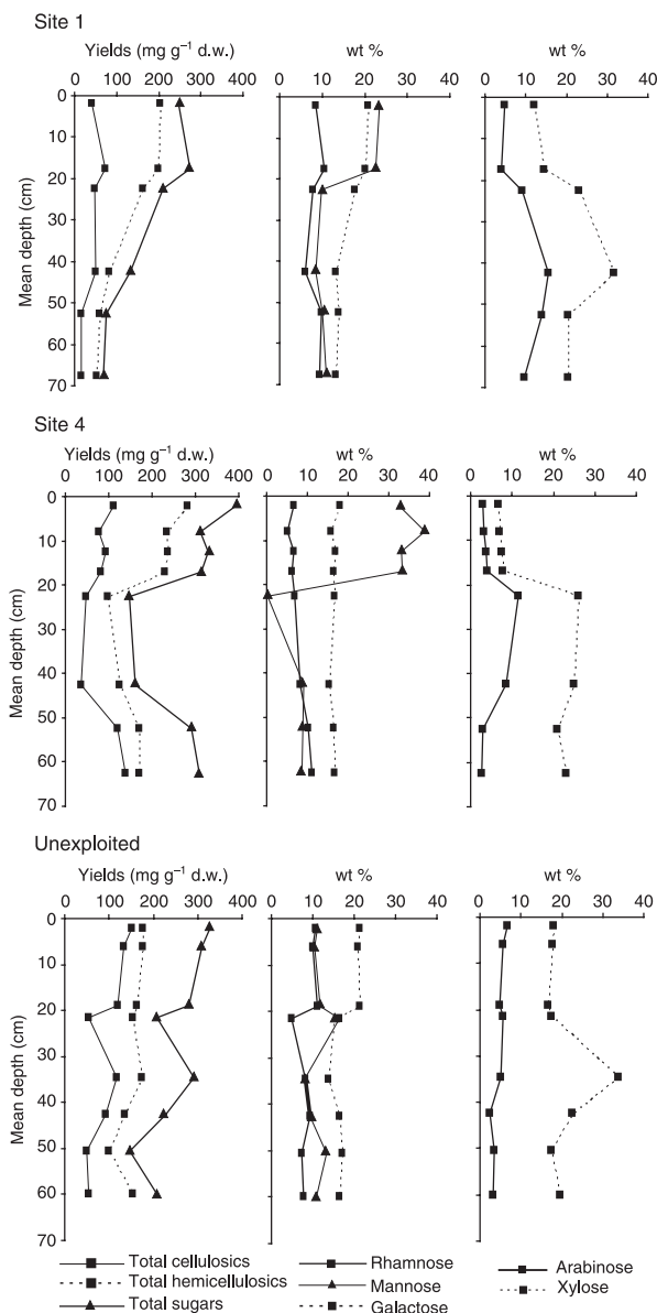
Fig. 5. Depth evolution of total sugar, cellulosics and hemicellulosics yields (mg g -1 ) and concentrations (wt%) of moss and Cyperaceae markers in the recent and advanced regenerating stages (sites 1 and 4) in comparison with the unexploited site.
