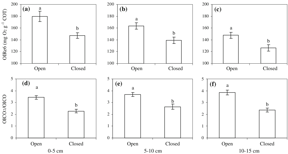
Fig. 4 Rock-Eval 6 oxygen index (OIRe6) and the ratio of the amount of pyrolysed CO 2 to the amount of pyrolysed CO (OICO 2 /OICO) of the uppermost peat (0–15 cm depth) from different vegetation plots (open and closed). The error bars represent one standard error ( n = 8)
