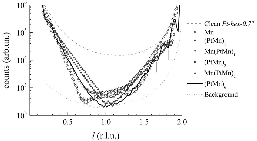
Figure 4.3: Stationary l -scans intensity along (1 1) CTR during Mn and Pt alternate growth at RT on a clean Pt\text{-}hex\text{-}0.7^\circ . The legend indicates each corresponding layer. Note that, hollow symbols represent Mn terminated and filled symbols Pt terminated layers. The final (PtMn)_6 film is plotted in a black solid line, where vertical bars highlight the thickness oscillations period. Yet, we added the measured clean surface and the background along (1.03 \ 1.03) , dash and dot gray lines, respectively, to make clear that the RT deposition yields a rough surface (the intensity in the anti-phase region comes only from the background in the final film).
