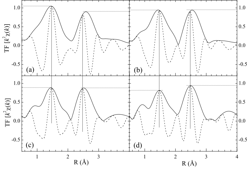
Figure 6.10: FT peaks corresponding to the oxygen and iron nearest neighbors for: (a) X=5.0 nm ( \approx 4 ML), (b) X=5.5 nm ( \approx 3 ML), (c) X=6.0 nm ( \approx 2 ML) and (d) X=6.5 nm ( \approx 1 ML). Solid lines give the moduli, while dashed lines give the real part of the FT.
