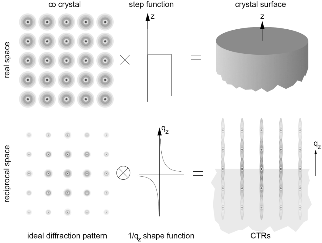
Figure 2.1: Origin of crystal truncation rods, explained qualitatively by the convolution theorem (taken from ref. [85]).
