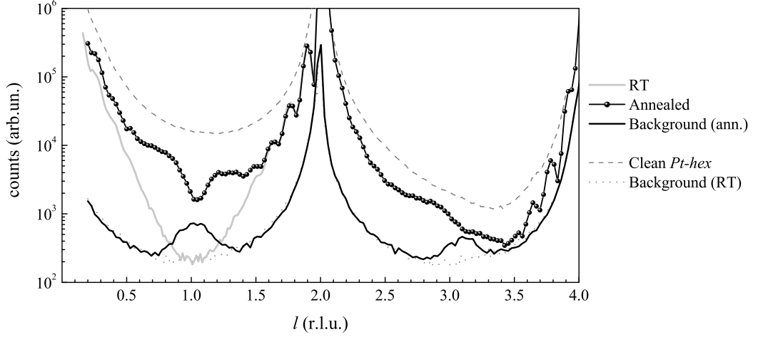
Figure 4.5: X-ray scattering along the (1 1) CTR for the (MnPt) 6 layer as deposited (gray solid line) and after annealing at 770 K (spheres). The offset scans, along (1.03 1.03 l ), evidence a large peak in the background after annealing.
