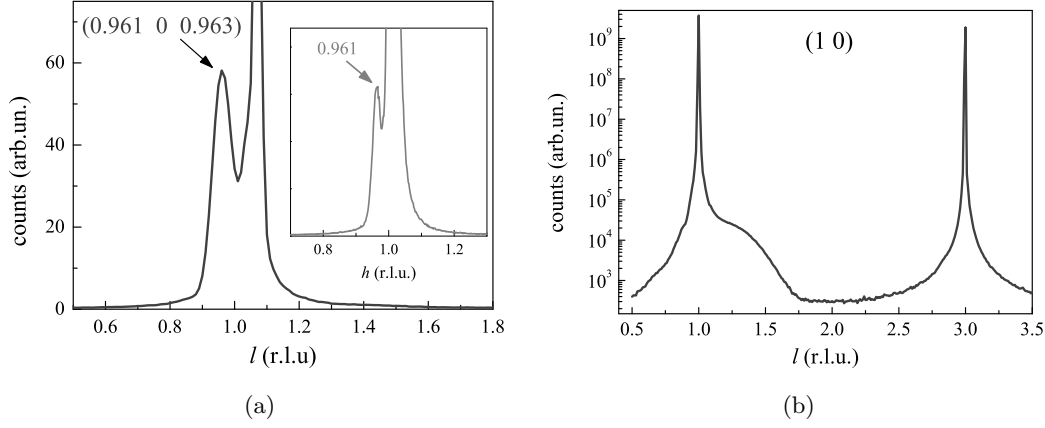
Figure 6.3: (a) l -scan along (0.961\ 0\ l) showing the relaxed CoO diffraction peak. The inset presents the radial scan along (h\ 0\ 0.96) . (b) l -scan along the (1\ 0) CTR, sensible to the pseudomorphic Fe layer on Ag(001), buried under the CoO film.
