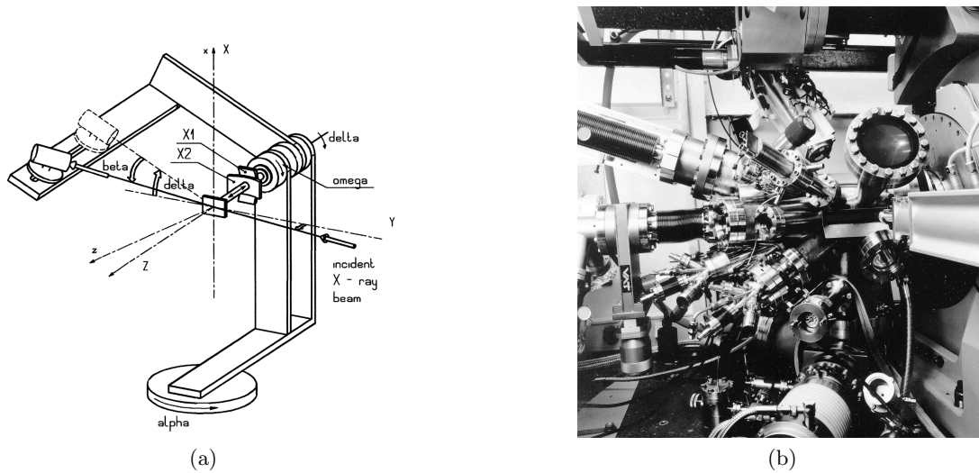
Figure 2.4: (a) Schema of the z-axis diffractometer [99]. (b) Picture of the SUV experimental setup.
