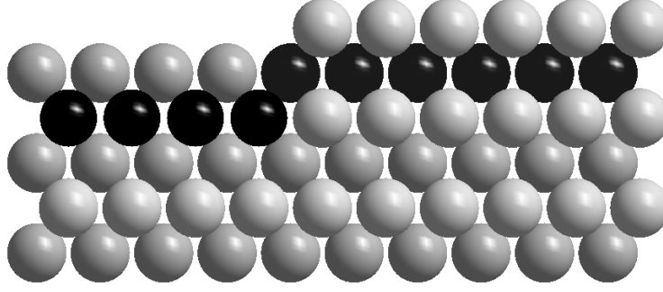
Figure 3.13: Sketch of one Pt ML on Ag(001)
