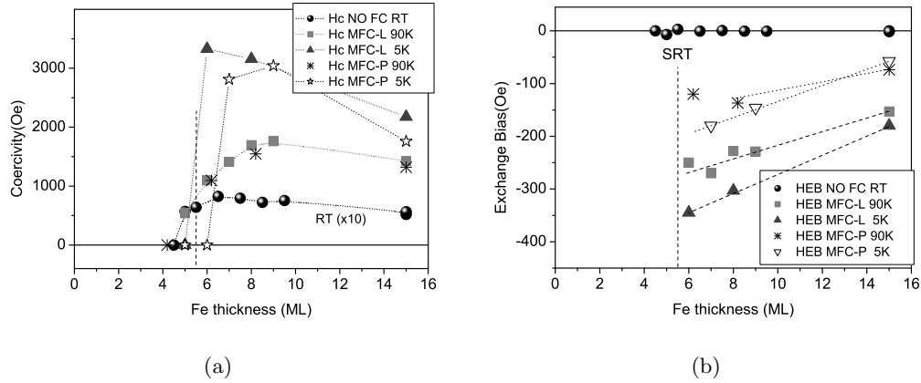
Figure 6.28: (a) Coercivity and (b) exchange bias shift for the CoO/Fe-wedge sample for different temperatures after magnetic field cooling from 315 K to 5 K under 0.55 Tesla.
