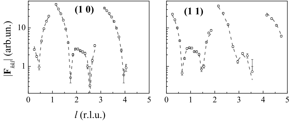
Figure 3.15: Experimental and fitted structure factors for 2 ML Pt/Ag(001) deposited at RT.
