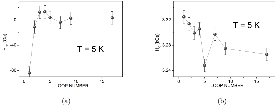
Figure 5.26: Training effect after perpendicular magnetic field cooling for \text{Pt}_6/(\text{MnPt})_8/(\text{FePt})_6/\text{Pt}(001) : (a) exchange bias shift and (b) coercivity as function of the number of loops.
