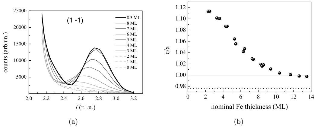
Figure 3.19: (a) Real time evolution of the (1\bar{1}) CTR during the Fe deposition. (b) Tetragonal distortion as function of coverage for two different depositions. Solid line gives the limit of no distortion; dotted line gives the situation where the volume of the unit cell is the same as bulk bcc Fe.
