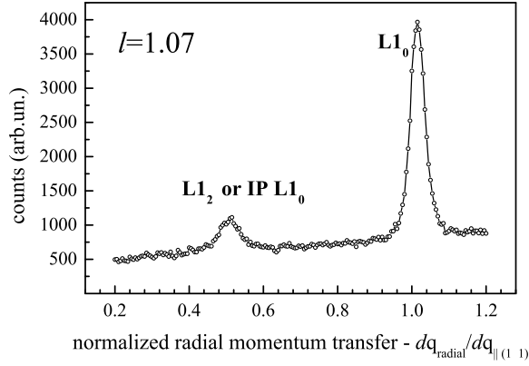
Figure 3.18: (\text{PtMn})_8\text{Pt}_3/\text{Ag}(001) . Radial scan across the (1.015 \ 1.015 \ 1.07) LRO peak.
