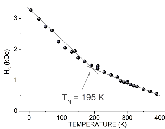
Figure 5.27: Coercivity as function of temperature for the \text{Pt}_6/(\text{MnPt})_8/(\text{FePt})_6/\text{Pt}(001) sample.
