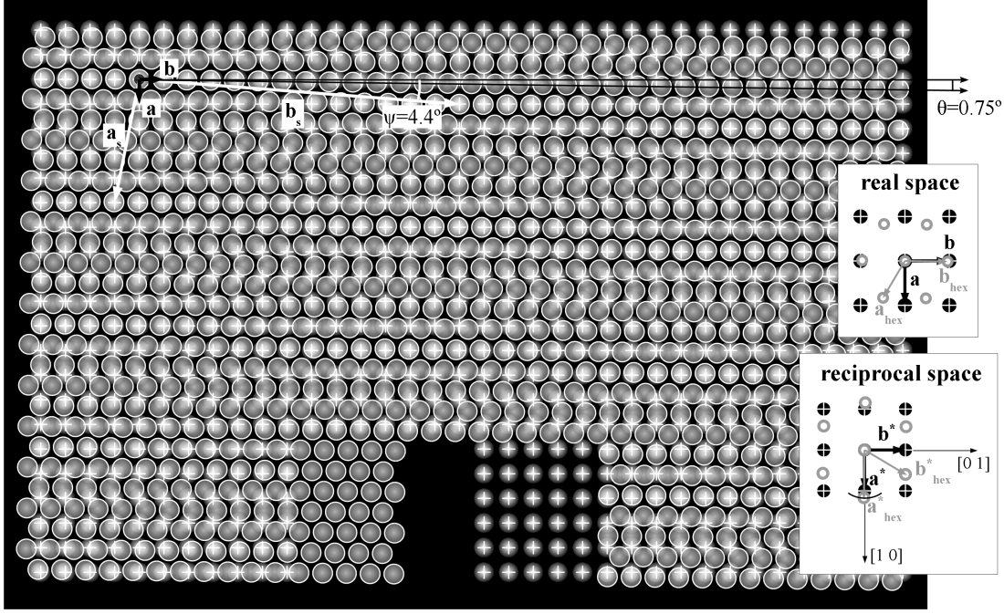
Figure 3.3: Schematic view of the Pt-hex-0.7° phase putting in evidence the \theta = 0.75^\circ rotation angle. White circles represent the top hexagonal layer, while crosses represent the underlying bulk with square symmetry. A possible surface unit cell is given by vectors \mathbf{a}_s and \mathbf{b}_s . In the insets the real and reciprocal spaces surface unit cell vectors are represented for both hexagonal and square layers.
