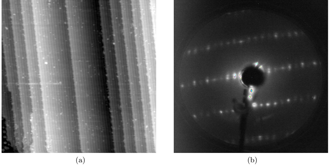
Figure 3.2: a) 100 nm \times 100 nm STM image of a 1°-miscut surface, showing the reconstruction rows aligned with the step edges; b) (5x1) LEED pattern of the same surface, evidencing that only one family of domains are present (beam energy of 169 eV).
