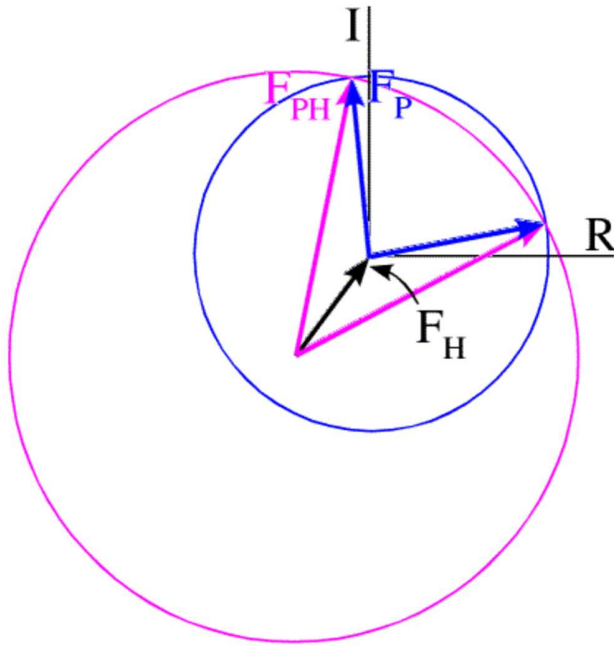
Figure 2.6: The Harker construction for the MIR method. The black vector \vec{F}_{Heavy} , (while having an error bar not represented here) is fully defined in both amplitude (length) and phase (orientation). The blue vector \vec{F}_{Prot} has only its amplitude known (represented as a blue circle centred on the \vec{F}_{Heavy} vector). The purple vector \vec{F}_{Prot+Heavy} representing the derivative dataset has only its amplitude known, therefore represented as the purple circle. The intersections of the two circles represent the two possible phases for \vec{F}_{Prot} and demonstrate the ambiguity of the method.
