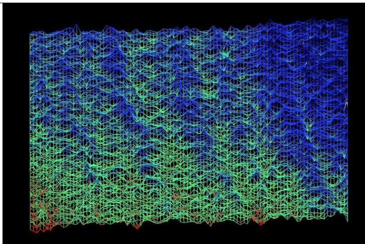
Figure 5.16: 3D views of zoomed regions of the detector. Colour depends on the measured intensity, at low angles the rings are well separated, at high angles several peaks are measured by the same pixels, this is the drawback of using 2D detector instead of high angular resolution instruments.
