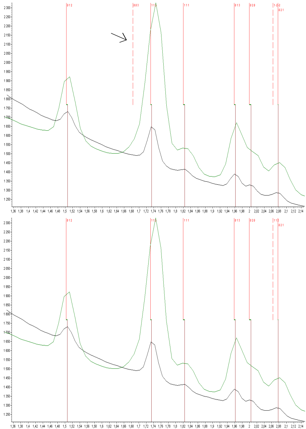
Figure 5.18: This is a zoomed view of 5.17 showing the first 6 peaks used for the indexing, to show the difference between the P3_1 solution and the P6_1 solution. In P3_1 the 003 peak though predicted is not observed. Its presence would exclude the P6_1 for which the extinction condition 00l, l=6n applies. Therefore this absence doesn't allow to exclude P3_1 , but suggest P6_1 .
