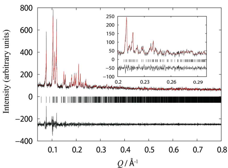
Figure 3.11: LeBail fit of ligand-free urate oxidase crystallised with NaCl and 8 % PEG 8000 ( P2_1 ) (ID31: \lambda = 1.30000(6) Å, 295 K). The black, red, and lower black lines represent the experimental data, calculated pattern, and difference between experimental and calculated profiles respectively. The vertical bars correspond to Bragg reflections compatible with its particular space group. The inset correspond to magnification of the fit in the selected Q range.
