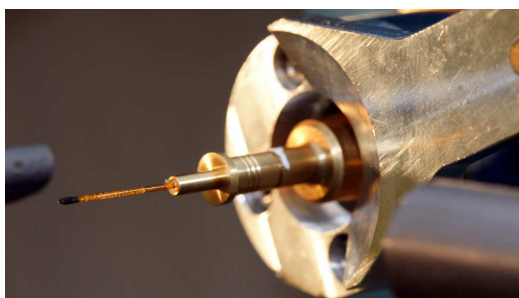
Figure 6.9: The complete setup for a cryocooling experiment (the cryostream is removed for a clearer view). The sample (in white) is centrifuged to the end of a kapton capillary. The capillary is sealed at one end with Sty-cast resin (black), and the capillary is held inside the brass holder with grease. The brass holder is held via a strong magnet on the spinner of the diffractometer.
