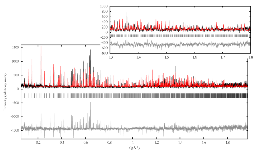
Figure 7.14: 2WUX structure, with prior background subtraction and with solvent scattering not refined.
