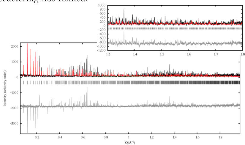
Figure 7.12: 2OH6 structure, with prior background subtraction and with solvent scattering not refined.
