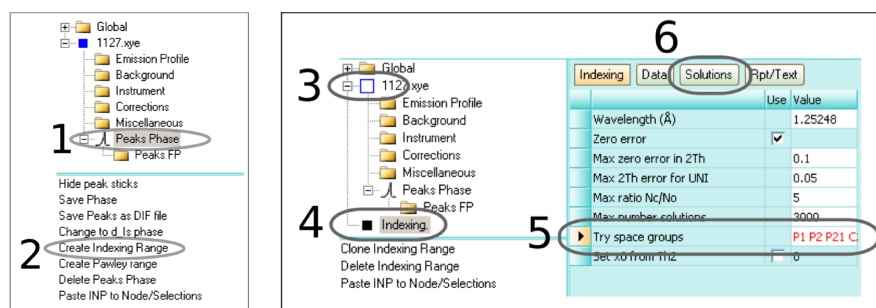
Figure F.2: The peak phase submenu (1) with create indexing range (2), the profile checkbox (3), the indexing menu (4), the try space group option (5) and the solutions menu (6).
