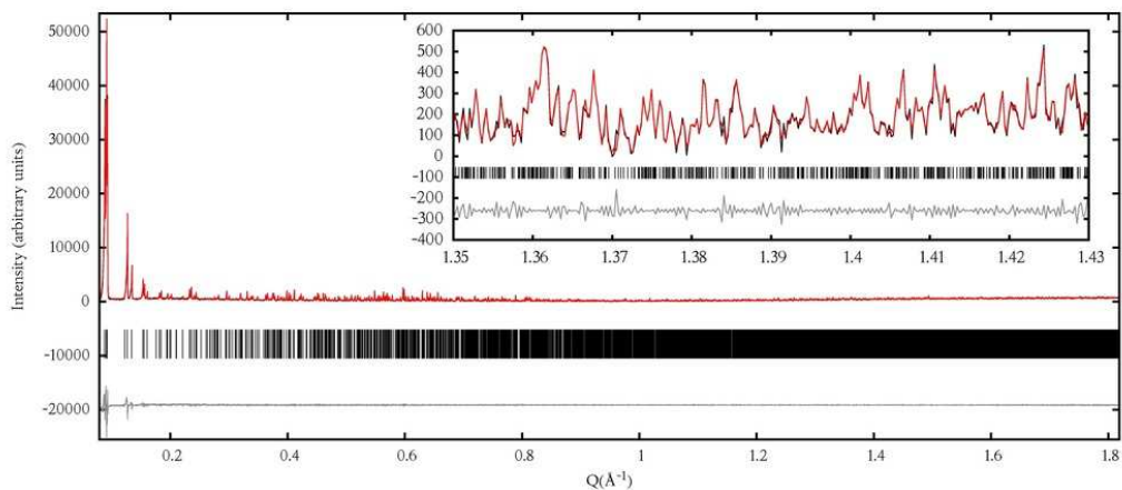
Figure F.3: Pawley fit of Glucose isomerase, I222, a=93.92614 , b=99.54783 , c=102.94948 . Powder pattern collected at ID31 ESRF.
