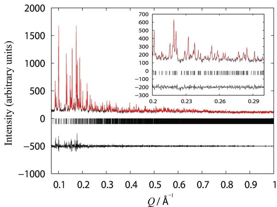
Figure 3.12: LeBail fit of ligand-free urate oxidase crystallised with NaCl and 15 % PEG 8000 ( P2_1 ) (ID31: \lambda = 1.30000(6) Å, 295 K). The black, red, and lower black lines represent the experimental data, calculated pattern, and difference between experimental and calculated profiles respectively. The vertical bars correspond to Bragg reflections compatible with its particular space group. The inset correspond to magnification of the fit in the selected Q range.
