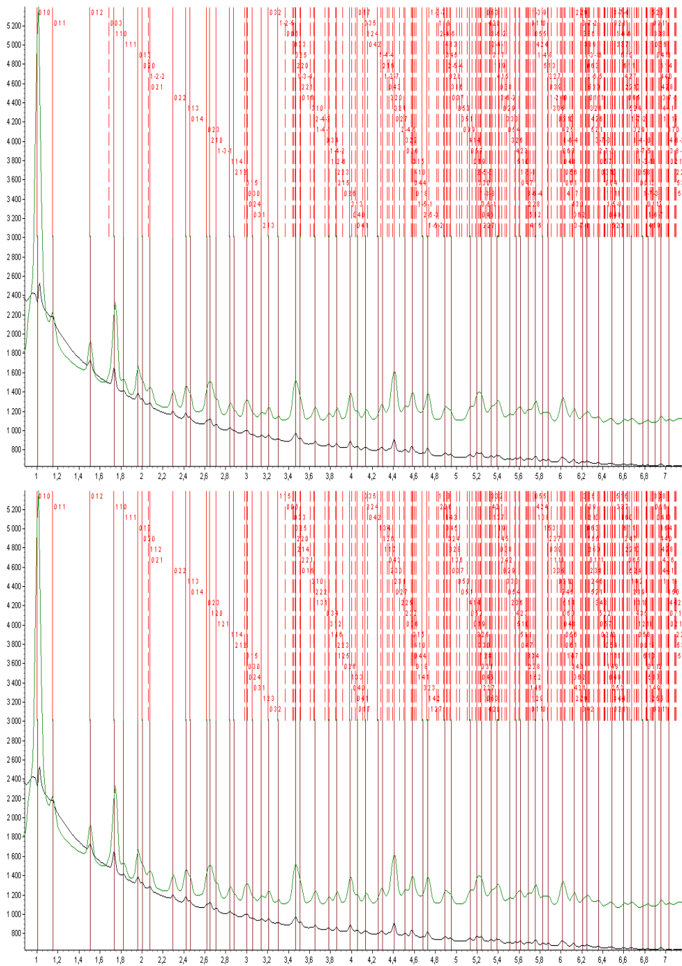
Figure 5.17: Indexing of two patterns collected on ID14-eh1 on a single urchin of mayaro virus with two different detector-sample distance (for the green curve detector distance is 659.180 mm, for the black curve detector distance is 434.485mm). On top is the P3_1 solution as found in previous experiments, below is the P6_1 solution. The upper dark red lines are the positions of the peaks used for the indexing procedure. The lower light red are the computed lines for the solution. The dashed red lines are the theoretical positions of peaks which have not been input for the indexing (unobserved peaks). This is a view of all the peaks used for the indexing.
