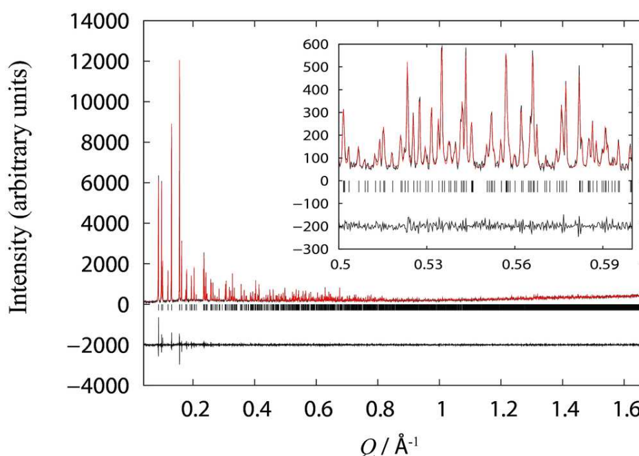
Figure 3.14: LeBail fit of Uox complexed to AZA and crystallised with NaCl ( I 222) (ID31: \lambda = 1.30000(6) Å, 295 K).
