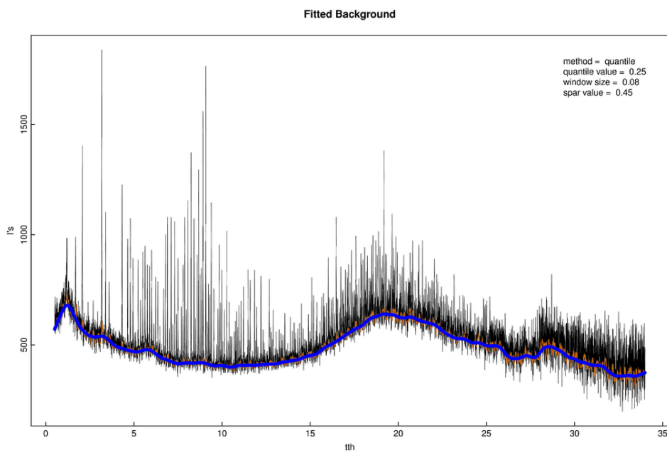
Figure E.2: In orange, the result of the rolling function determined by taking the first quartile in a window of 0.08 degrees around the point. In blue the smoothed function using a smoothing parameter value of 0.45.
