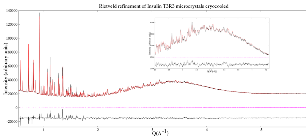
Figure 6.21: Rietveld fit of human insulin T3R3 cryocooled at 5K using a Liquid-helium-cooled cryostat. The fit was obtained after refining the room temperature powder crystal structure 1FUB with GSAS.
