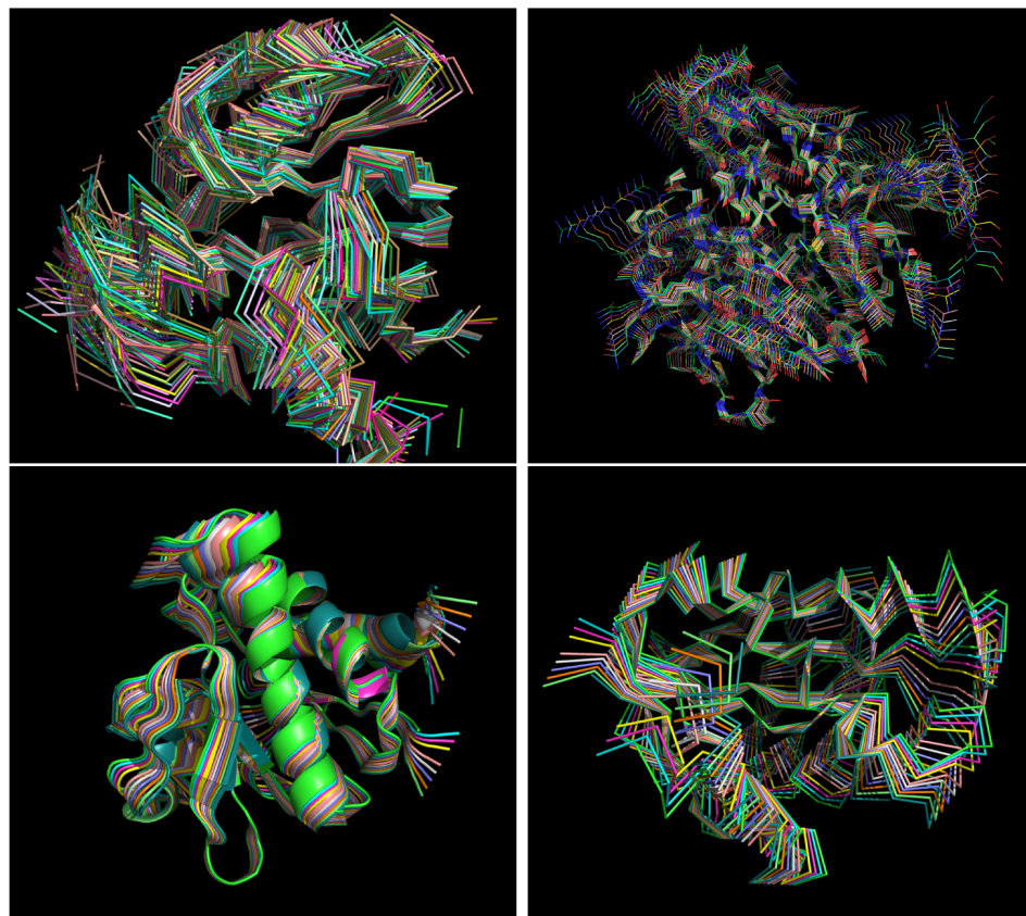
Figure 5.20: The normal mode models computed based on a mutated 3GPG model. A first model based on the chikungunya 3GPG structure is mutated to correspond to a mayaro sequence. Then normal modes 7/8/9/10/11 with perturbation amplitude between -100 and +100 (step=20) are computed using the Elnemo web server [53]. Top left images represent all the models (all modes) used for the molecular replacement search. The three others are different representations of the search ensembles giving the best score during the molecular replacement search.
