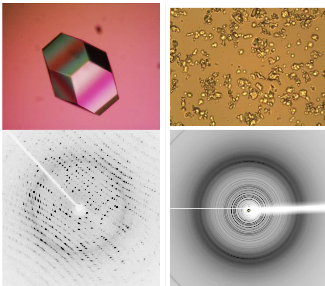
Figure 1.1: Top left is a single crystal (Photographed by Mathias Klode), top right is a crystalline protein precipitate. Bottom left are the resulting X-ray image of one single crystal at one orientation, bottom right is the rings observed when a protein powder is diffracting.
