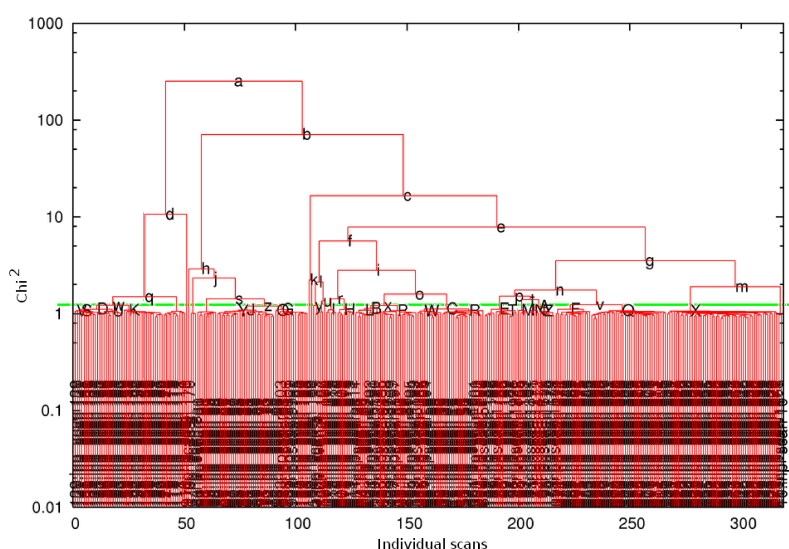
Figure 5.6: The clustering of all the patterns collected on the first attempt on ID31.
