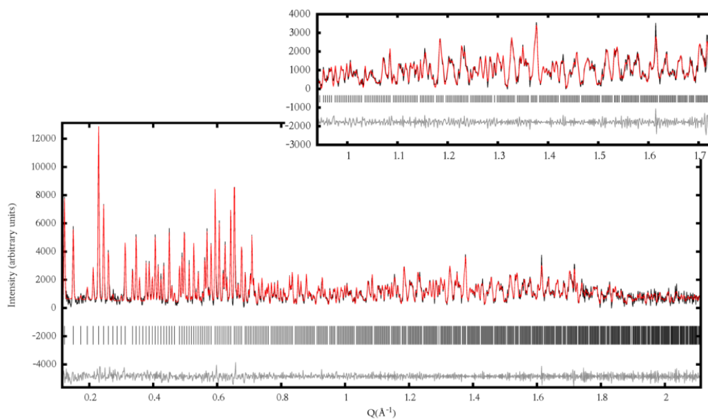
Figure 7.4: Final fit of the CpGV using the Pawley method. The data were collected at a temperature of 295 K (ID31, \lambda = 1.53985(4)\text{\AA} ), Space group is I23 lattice parameter is a=102.6108(4)\text{\AA} .
