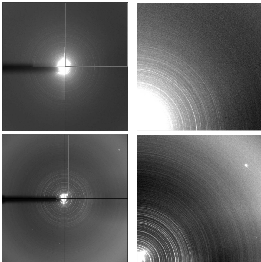
Figure 5.15: On the left, two images taken on the same urchin, at two different beam positions, with two different sample to detector distances. On the right, a zoomed region of a quarter of the detector. On some images, a clear spot of a salt single crystal is seen (and will be excluded).
