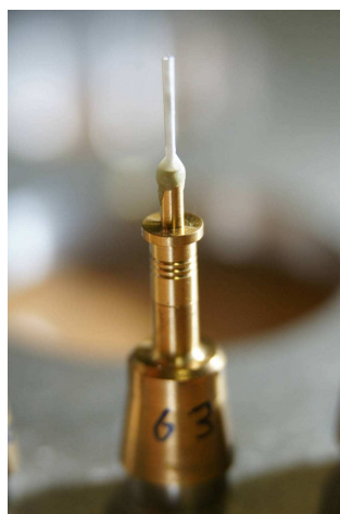
Figure 6.7: A typical sample holder for room temperature protein powder diffraction. The brass parts are made to hold the 1 mm borosilicate capillary centred in the beam while being spun at high speed (typically 1000 rpm).
