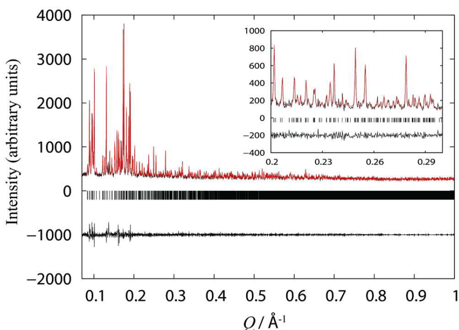
Figure 3.13: LeBail fit of ligand-free urate oxidase crystallised with (NH_4)_2SO_4 and 15 % PEG 8000 ( P2_1 ) (ID31: \lambda = 1.30000(6) Å, 295 K). The black, red, and lower black lines represent the experimental data, calculated pattern, and difference between experimental and calculated profiles respectively. The vertical bars correspond to Bragg reflections compatible with its particular space group. The inset correspond to magnification of the fit in the selected Q range..
