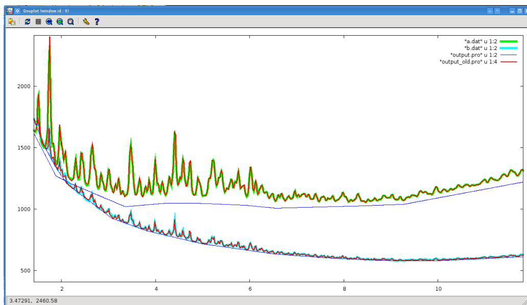
Figure G.1: Gnuplot can be used to see the fitted powder patterns refined within PRODD.
