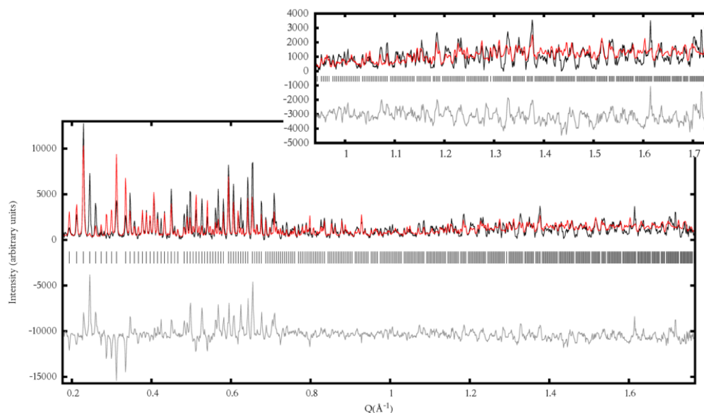
Figure 7.28: CpGV single crystal structure (current single crystal model from Peter Metcalf, unpublished) Rietveld fit compared to powder data, after a rigid body refinement. A very small improvement of the fit is seen.
