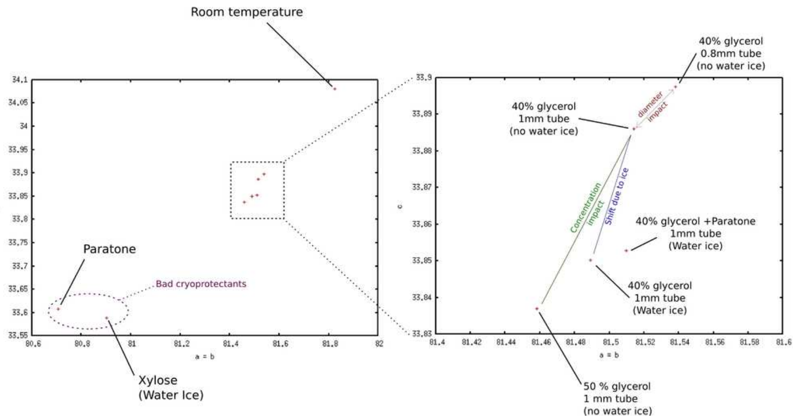
Figure 6.13: The high angular resolution of ID31 diffractometer allows us to see shifts in lattice parameters of human Insulin T6 due to cryoprotectants. The same batch of microcrystals is used in all experiment removing crystallisation variation bias. It is also interesting to see that for the same condition (40% glycerol), in one case when the sample wasn't plunged inside liquid nitrogen (but directly cooled with the cryostream) the cooling speed reached wasn't sufficient and gave crystalline ice.
