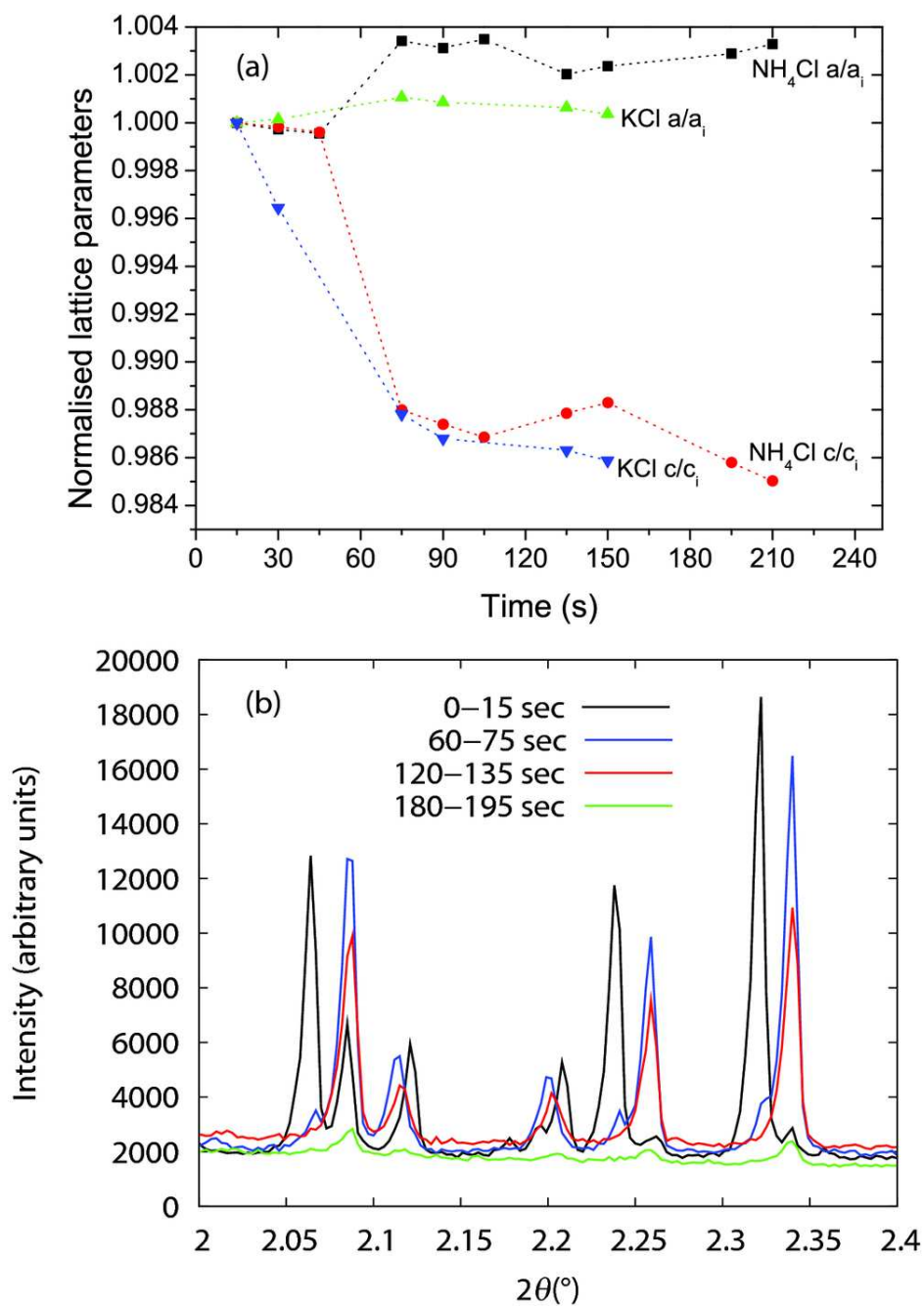
Figure 3.10: (a) Anisotropic variation of the normalised lattice dimensions of trigonal ligand free Uox crystallised with NH_4Cl or KCl at pH 8 ( P3_121 ) with increasing sample exposure time to the synchrotron beam. (b) Selected 2\theta region of powder diffraction profiles of Uox crystallised with NH_4Cl at pH 8 (ID31: \lambda = 1.30000(6) Å, 295 K) showing a gradual evolution of the peak positions and widths with increasing irradiation time. The colours correspond to different sample exposure times varying from 15 to 195 seconds.
