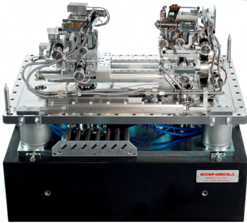
Figure 2.2: ID11 Laue/Laue monochromator
