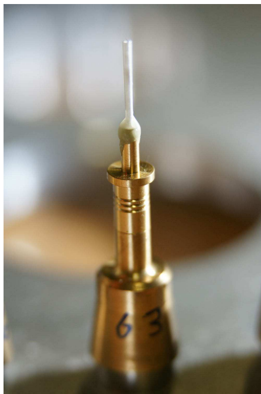
Figure A.3: A typical 1.5 mm capillary mounted on an ID31 brass holder. The brass holder allows use of the spinner mounted on the axis of the diffractometer, but also the sample changer robot.
