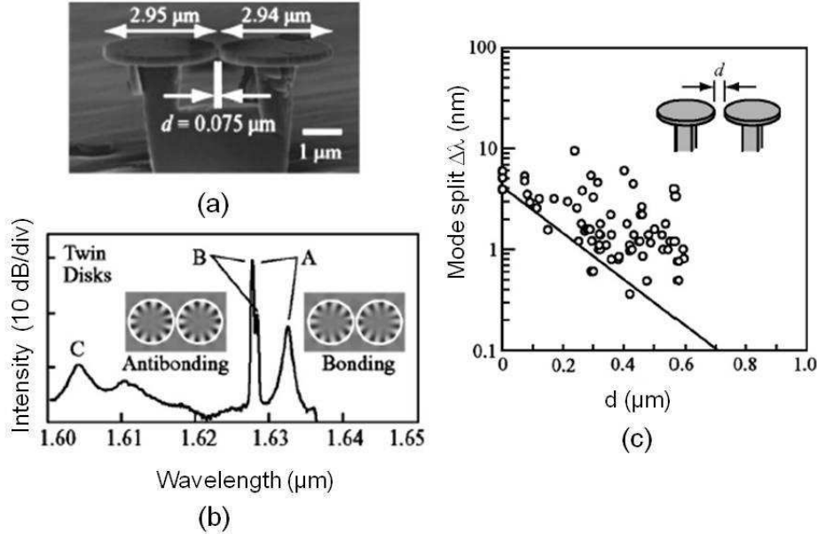
Figure 1.23: (a) Scanning electron images of twin microdisks. (b) Lasing spectra. Inset figures are magnetic field profiles of bonding and antibonding states of the eleventh order whispering gallery mode. (c) Mode split ( \Delta\lambda ) vs interdisk spacing ( d ) characteristic of twin disks. The dots and the line are measurement and calculated results, respectively. Images from [57]
