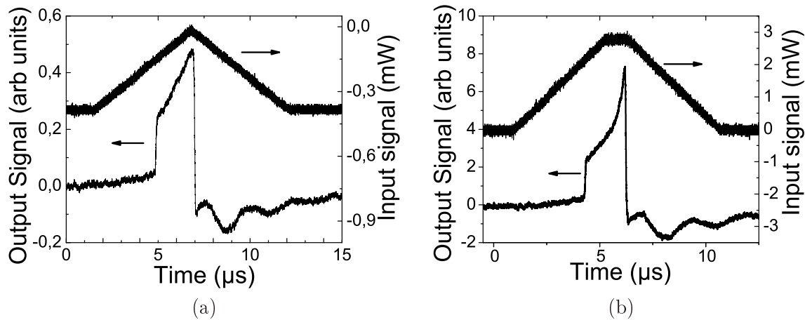
Figure 6.8: Bistability measurements for a longer signal modulation with constant injection intervals: (a) 11 \mu s and (b) 10 \mu s with 1 \mu s of time-out. Reflection signal (lower trace) and input signal (upper trace) as a function of time for a detuning of \Delta\lambda_0 = 1.6 \text{ nm} . Note the similarities between the shape of the bistable pulse and the excitable pulse (fig. 6.6) specially the curve in (b).
