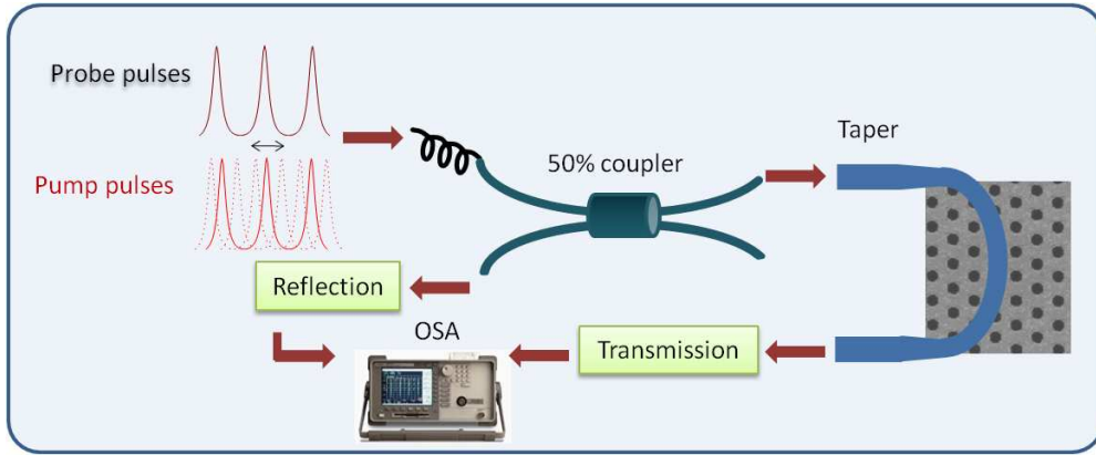
Figure 4.12: Experimental setup for fibered pump. Using a translation stage, the pump pulses are delayed with respect to the probe pulses before being sent to the tapered fiber.
