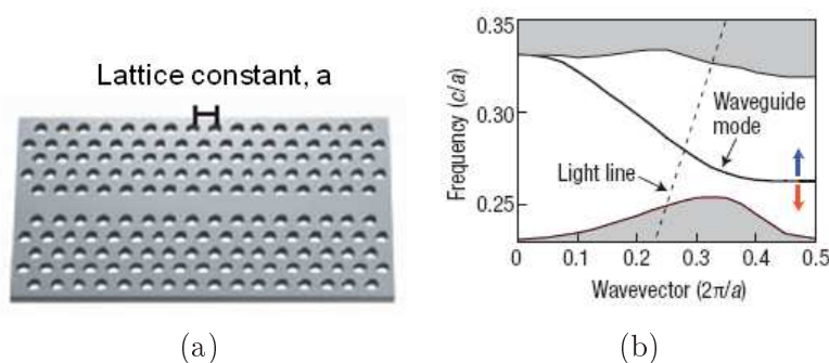
Figure 1.31: (a) Sketch of a W1 guide, i.e. a whole missing line of holes. (b) Band diagram of this structure. The PhC bandgap takes place inside the white region. Note that a band of the waveguide lies within this bandgap. Images from [70].
