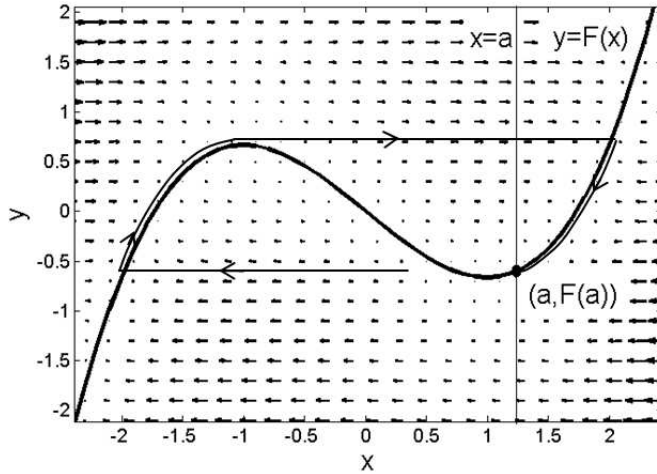
Figure 1.12: Nullclines of eq. 1.24 in the phase space. The line with the arrows represent an example of a possible excitable trajectory. The small arrows show the velocity vector direction at each point of the phase space.
