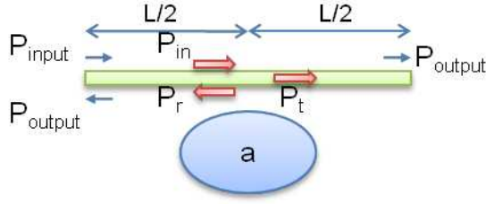
Figure 2.7: Scheme of the distributed losses in the microfiber.
