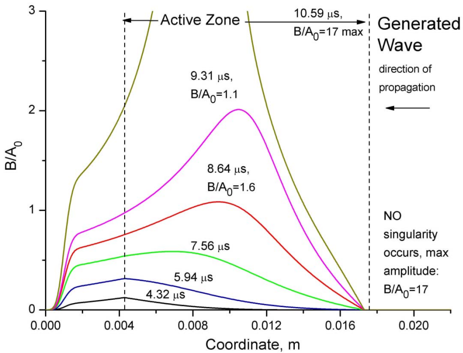
Figure 5.17. Supercritical time evolution of spatial distribution of generated wave amplitude B/A_0 during three waves coupling process under parallel pumping with nonlinear phase shift. Distributions are shown for time moments: 4.32 \mu\text{s} (black), 5.94 \mu\text{s} (blue), 7.56 \mu\text{s} (green), 8.64 \mu\text{s} (red), 9.31 \mu\text{s} (purple) and 10.59 \mu\text{s} (khaki). No singularity is observed. A_0 = 10^{-10} , h_0 = 50 \text{ Oe} , \Gamma = 1.04 .
