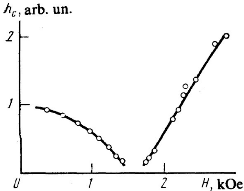
Figure 1.8. Dependence of the threshold amplitude of the parallel pumping field on the static magnetic field of the parametric quasiphonon generation in \text{FeBO}_3 at T = 77 K [105].
