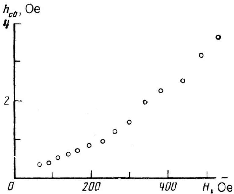
Figure 1.9. Amplitude dependence of the shear pumping threshold field h_c on the static field H of the parametric quasiphonon generation in \text{FeBO}_3 , T = 90 K, \omega_p = 35.0 GHz [109].
