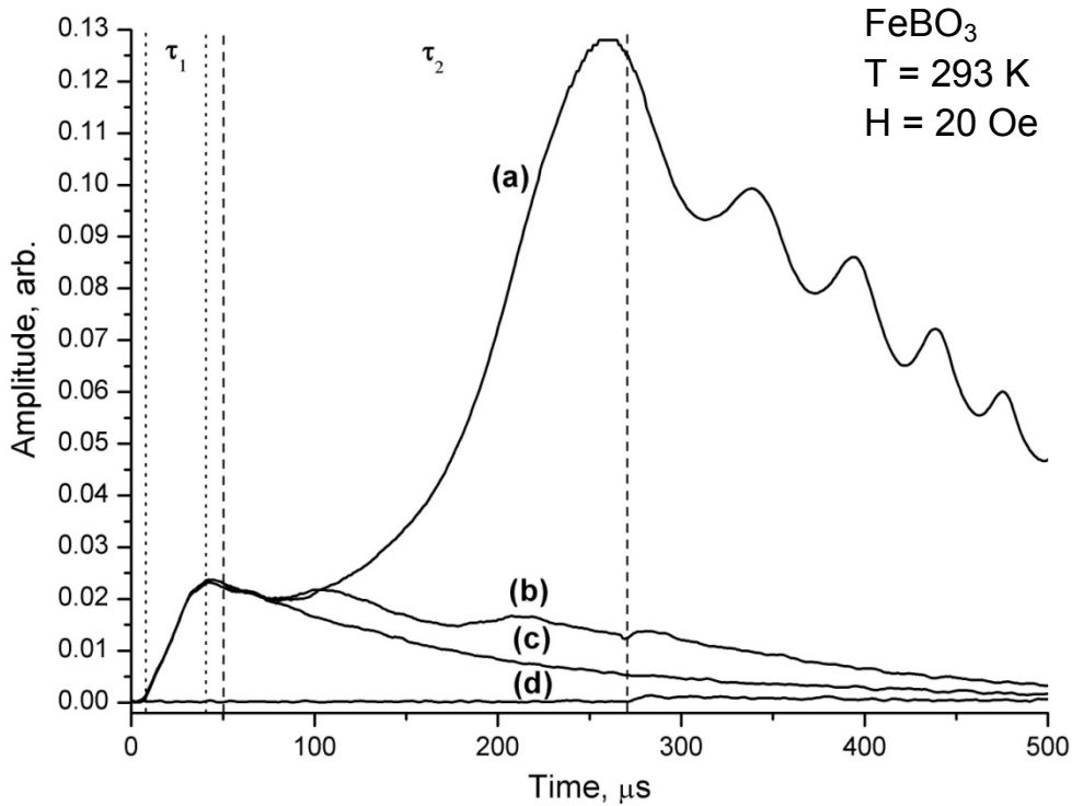
Figure 3.29. Experimental time dependences of amplitude of magneto-elastic oscillations under electromagnetic pumping in FeBO_3 crystal at 293K: (a) with pumping frequency modulation ( h_p=15 Oe) (b) without frequency modulation ( h_p=15 Oe) (c) without applied pumping ( h_p=0 ), (d) without initial pulse ( a_{n0}=0 ); \tau_1 and \tau_2 are the durations of initial exciting pulse and pumping pulse respectively.
