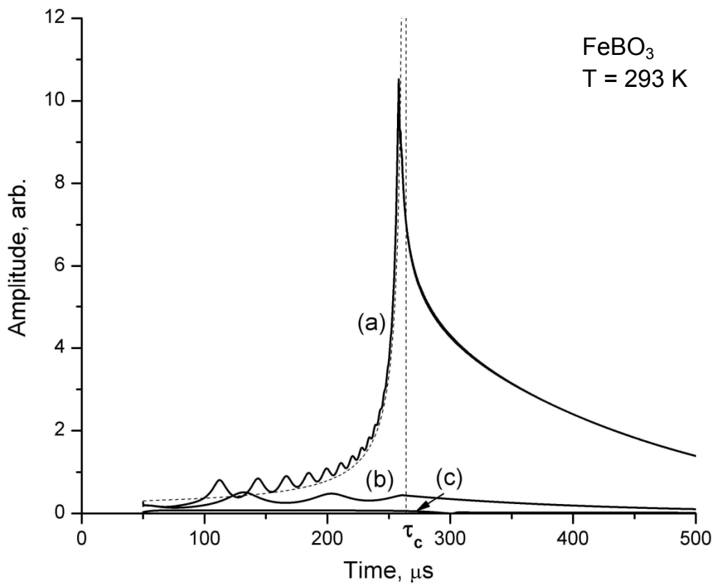
Figure 4.1. Calculated time dependencies of magnetoelastic oscillations amplitude under electromagnetic pumping in \text{FeBO}_3 resonator at 293 K (a) with proposed phase modulation law, (b) without frequency modulation, (c) without initial excitation a_{n0} = 0 ; dashed line shows theoretical explosive amplitude growth when \beta_n = 0 that reaches singularity at the time \tau_c .
