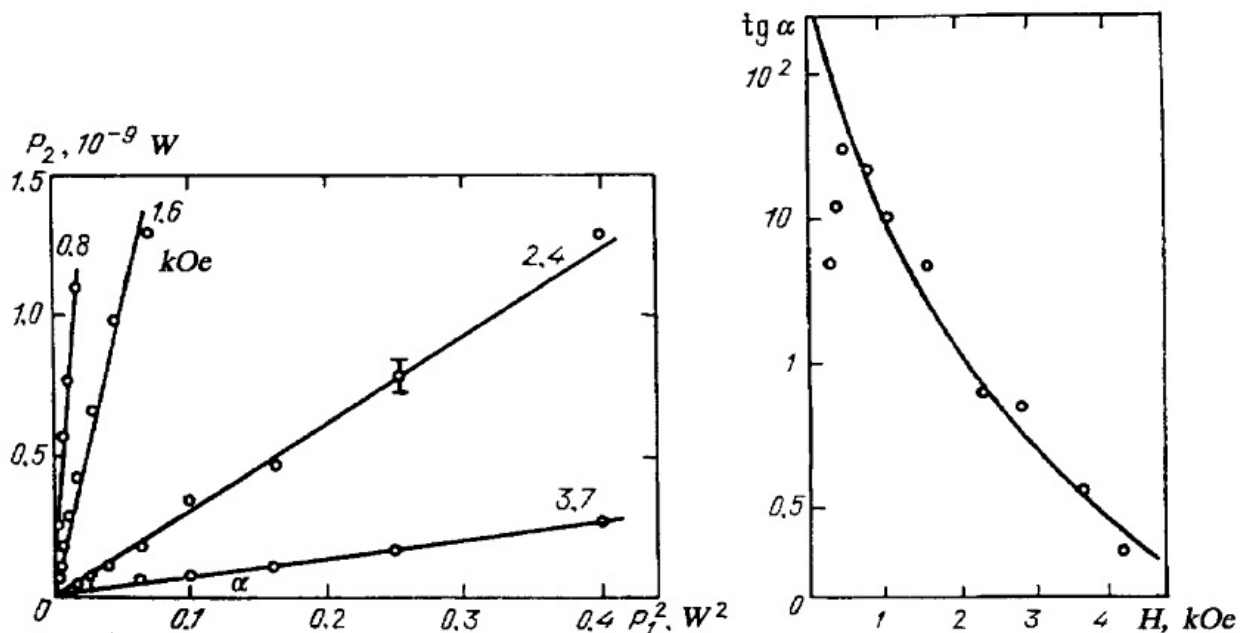
Figure 1.10. Dependencies of the second harmonic power on the square of initial wave power at different bias magnetic fields (left). Dependence of the effectiveness of sound wave transformation on the bias magnetic field (right) [115].
