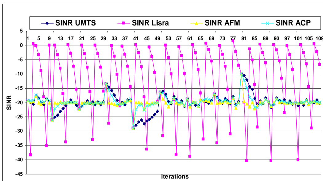
Figure 5.32. SINR variation for vehicle
