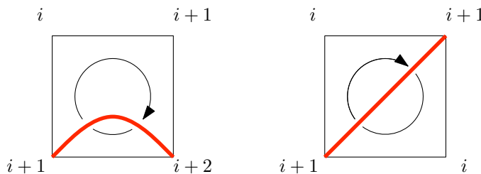
FIGURE 6.4 – Rules for the reverse Schaeffer construction.
