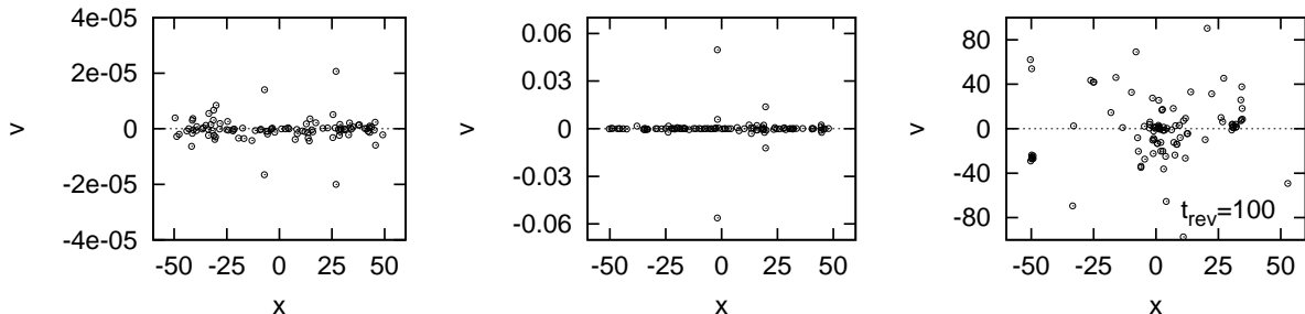
Figure 4.21: Configuration in phase space of reversibility test with t_{rev} = 1 (left), 10 (middle) and 100 (right) for N = 100 and R_0 = 0 .
