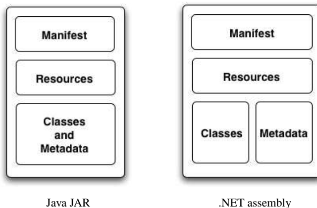
Figure 3.1: Java JARs and .NET assemblies
