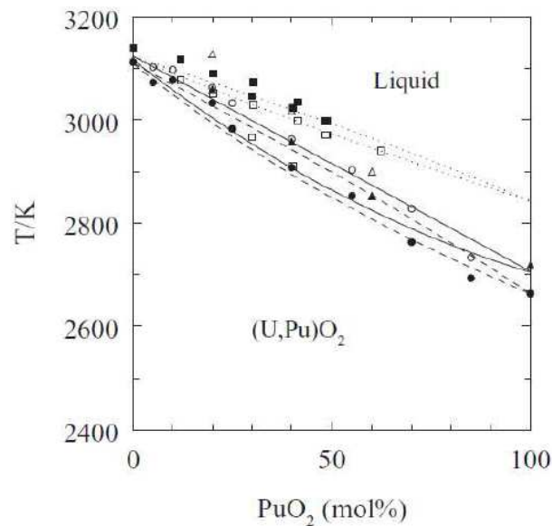
Figure 4: UO 2 -PuO 2 region; The circles correspond to the experimental data by Lyon and Bailey 10 , the triangles by Aitken and Evans 11 , and the squares by Kato et al 15 ; The solid lines represent the recommended liquidus and solidus by Adamson et al 12 , the broken line the ideal liquidus and solidus based on Lyon and Bailey 10 , and the dotted line the liquidus and solidus suggested by Kato et al.
