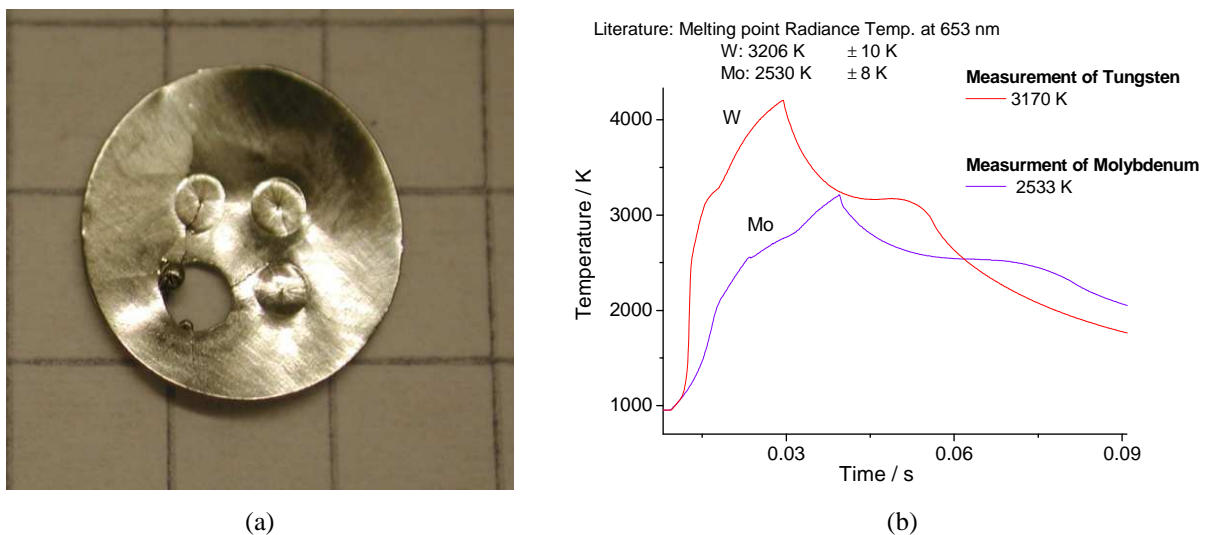
Figure 7: (a) A molybdenum foil on which four laser shots were performed. (b) Measured thermograms on molybdenum and tungsten.
