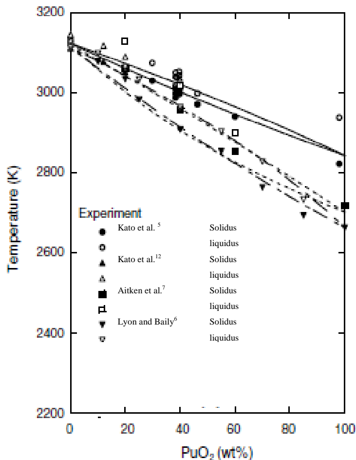
Figure 4: Solidus and liquidus temperature in the \text{UO}_2 - \text{PuO}_2 system.
