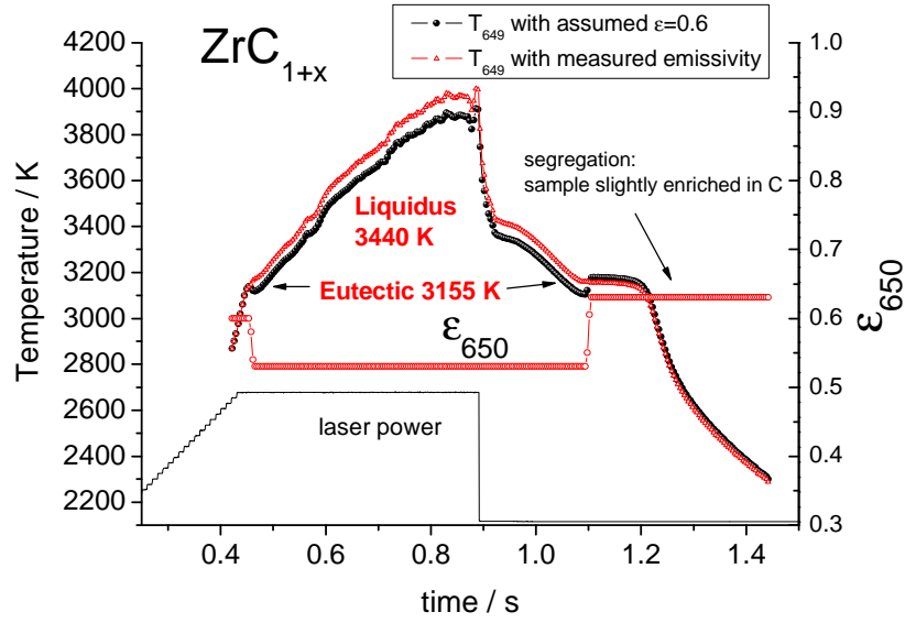
Figure 17: Thermogram of a ZrC_{1+x} sample measured at 650 nm. The thermal arrests corresponding to the eutectic have been fixed at 3155 K. Emissivity of solid and liquid ZrC_{1+x} could then be deduced accordingly. Black curve: thermogram corresponding to an assumed constant emissivity \epsilon(650)=0.6 . Red curve: thermogram corresponding to the real emissivity values.
