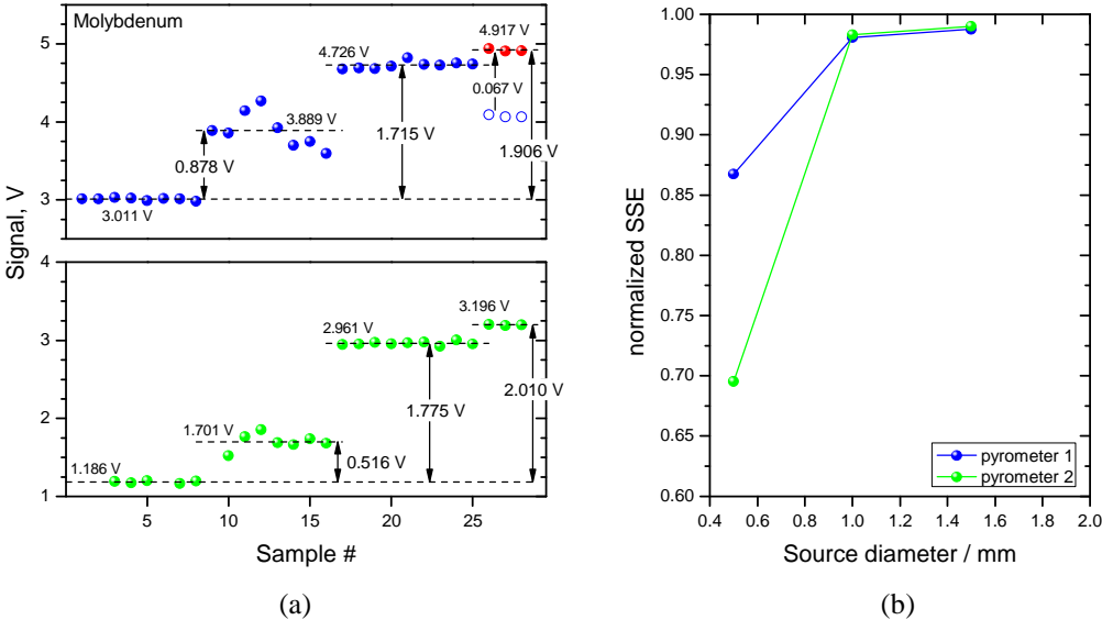
Figure 10: (a) Pyrometer signals at the freezing temperature of molybdenum recorded on intact samples and on samples with a Ø0.5, Ø1.0, and Ø1.5 mm hole. (b) Normalized SSE derived from these measurements.
