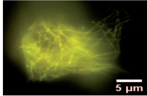
(b) Maximal displacement of microtubules is 0.15 \pm 0.06 \mu\text{m} .
