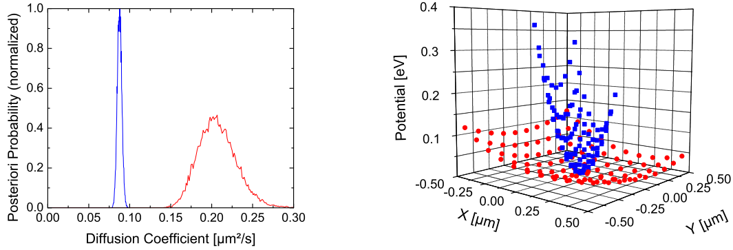
(a) Posteriori probability for the diffusion coefficient D_{Inf} before and after 10 minutes of cholesterol extraction.
