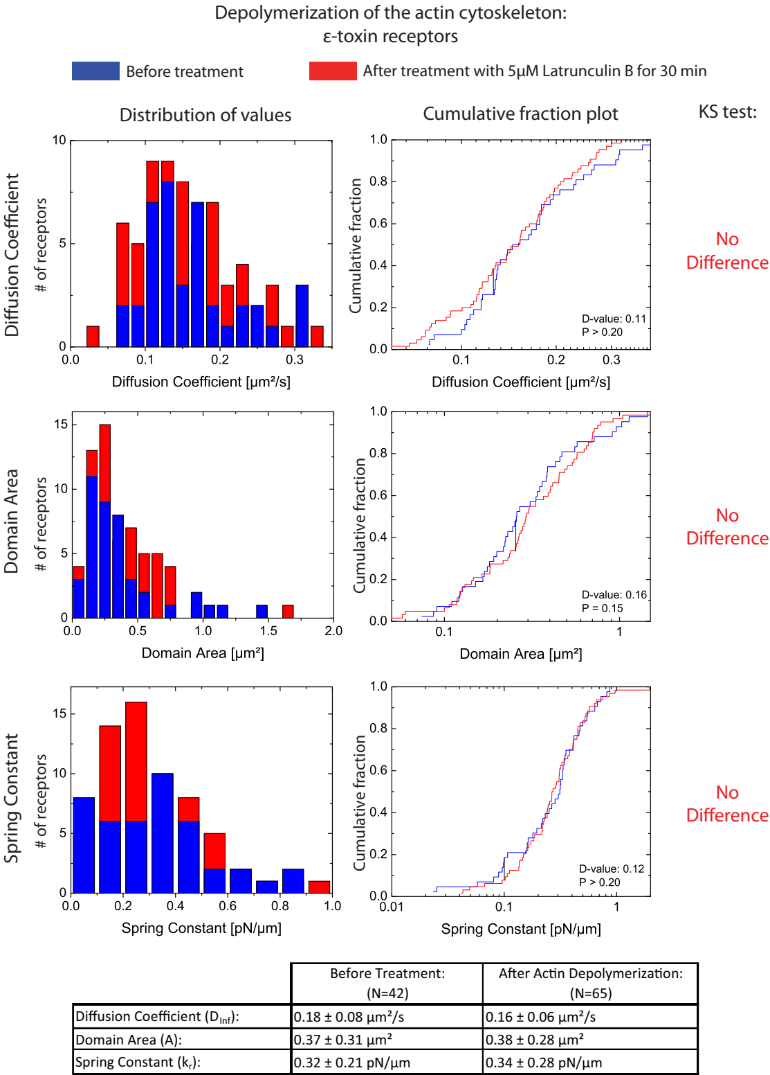
Figure 5.7: Effect of actin depolymerization on the motion of \epsilon -toxin receptors. Cells were treated with 5 \mu M Latrunculin B at 21 ^{\circ}\text{C} for 30 minutes. No significant differences are observed in diffusion coefficient, domain area and spring constant before and after treatment.
