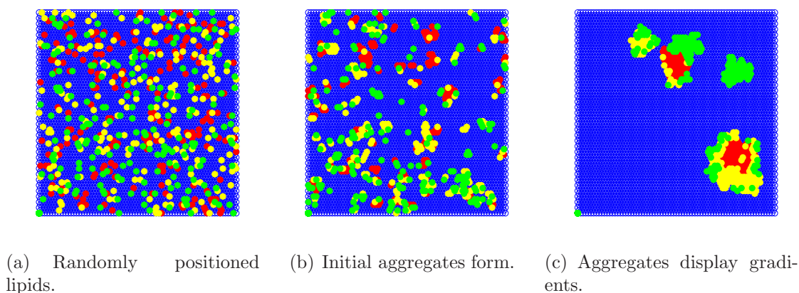
Figure 5.13: Aggregation due to hydrodynamic mismatch. The blue particles are the matrix. The hydrophobicity mismatch of the other three species is indicated by their color, from green (least) to red (highest) mismatch. When the system is allowed to lower its energy, aggregation occurs along with sorting of the particles. The sorting creates a radially decreasing profile in hydrophobicity mismatch in the aggregates.
