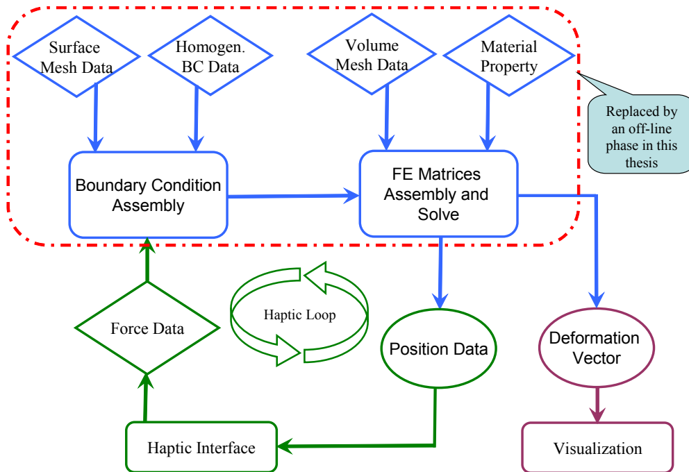
Figure 4.1 – Components and relations between them in the haptic deformation model.
