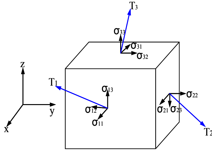
Figure 2.2 – Stress components.
