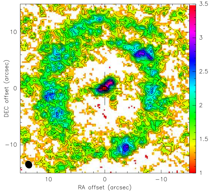
Figure 5.12: ^{12}\text{CO}(2-1) integrated intensity contours observed with the IRAM interferometer toward the center of NGC 3147. The cross marks the coordinates of the center as given in Table 5.1 with offsets in arcseconds. The rms noise level is \sigma = 0.2 Jy/beam \text{km s}^{-1} . The map, derived with 2\sigma clipping, has not been corrected for primary beam attenuation. Contour levels are from 2\sigma to 18\sigma with 1\sigma spacing. In this map the whole velocity range is used: \pm 240 \text{km s}^{-1} with 49 channels in steps of 10 \text{km s}^{-1} . The beam of 1.4'' \times 1.2'' is plotted at the bottom left.
