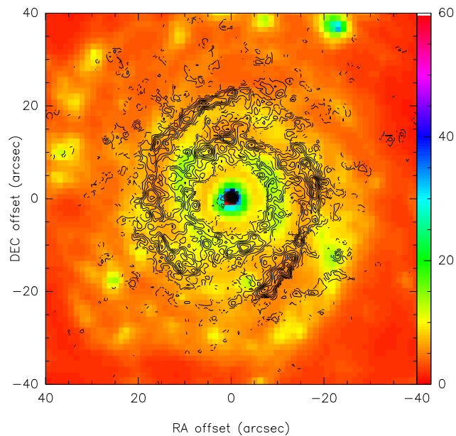
Figure 5.23: Superposition of the CO(1-0) contour levels shown in Fig. 5.10 and the 8\ \mu\text{m} Spitzer/IRAC image shown in Fig. 5.22. The central 80'' are shown. There is a good agreement between the CO(1-0) and the mid-IR emission in the inner ring, but the external CO(1-0) pseudo-ring does not correspond to the dust emission structures. The CO is found in the dust “interarm” region.
