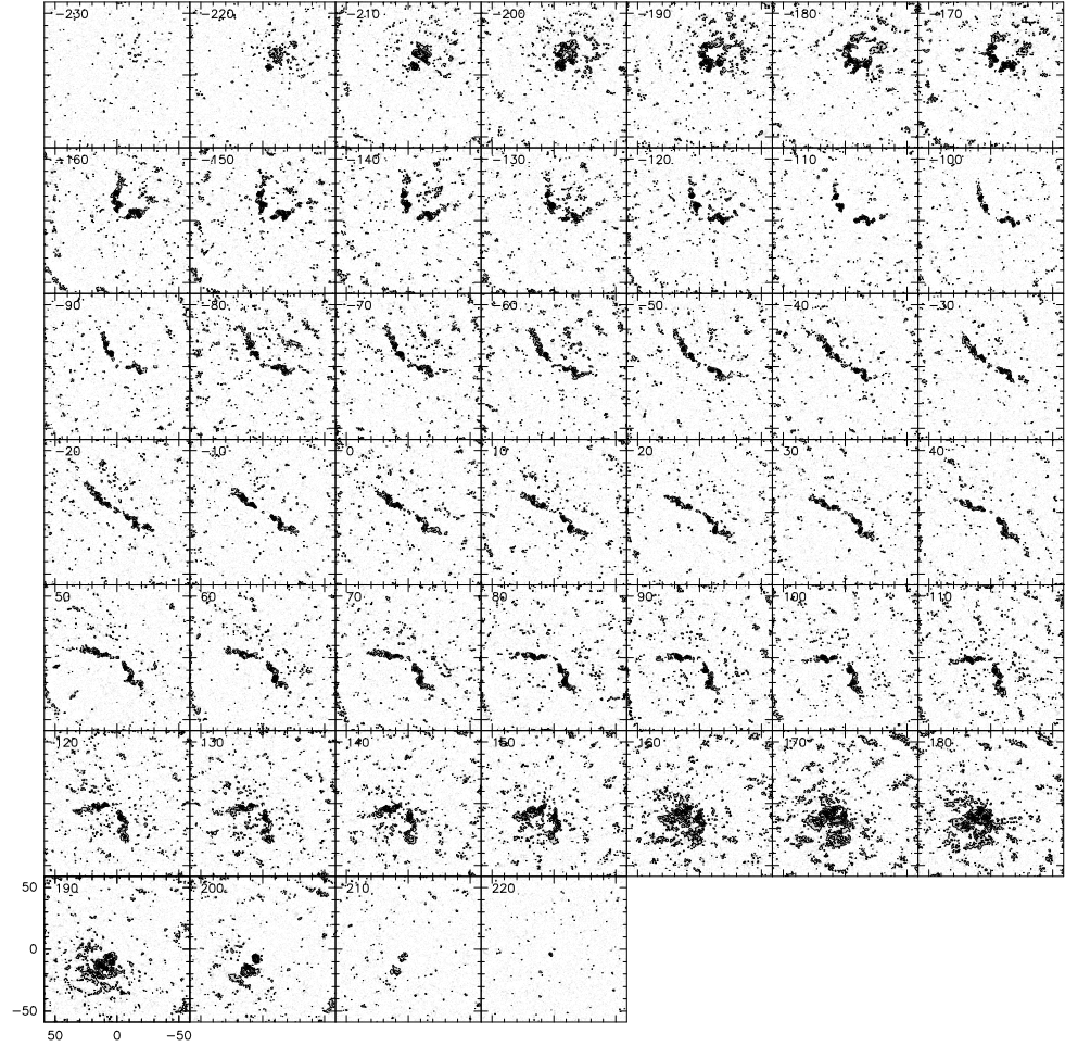
Figure 5.9: CO(1-0) velocity channel maps observed with the IRAM interferometer in the nucleus of NGC 3147 with a spatial resolution of (HPBW) 1.8'' \times 1.6'' . The center of the observations, given in Table 5.1, is \alpha_{2000} = 10^h 16^m 53.6^s , \delta_{2000} = 73^\circ 24' 03'' . Velocity-channels range from v = -230 \text{ km s}^{-1} to v = 220 \text{ km s}^{-1} in steps of 10 \text{ km s}^{-1} relative to V_{hel} = 2813 \text{ km s}^{-1} . The contours begin at 5 \text{ mJy/beam} , their spacing is 5 \text{ mJy/beam} , and the maximum is 50 \text{ mJy/beam} .
