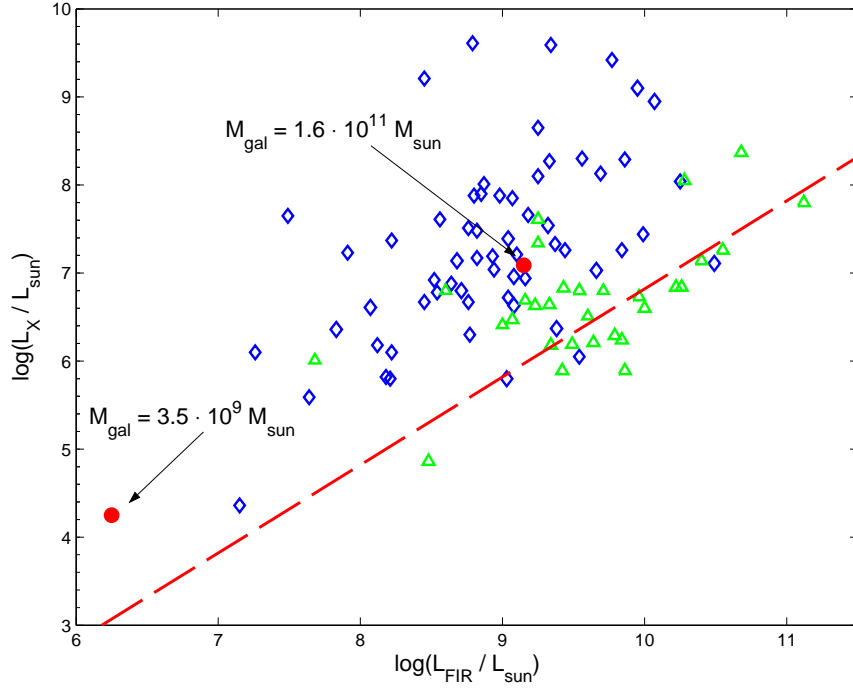
Figure 3.11: L_{FIR} versus L_X diagram as in Fig. 3.8 with the values deduced for the two template models of the early-type galaxy (filled circles). The diamonds represent the E-S0 galaxies, the triangles the S0a-Sb galaxies. The masses of the two theoretical models are also indicated. The galaxy with \log L_X / L_\odot > 10 present in Fig. 3.8 is not plotted here.
