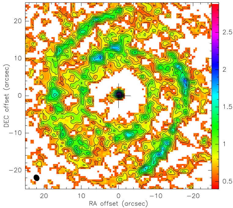
Figure 5.10: ^{12}\text{CO}(1-0) integrated intensity contours observed with the IRAM interferometer toward the center of NGC 3147. The cross marks the coordinates of the center as given in Table 5.1 with offsets in arcseconds. The rms noise level is \sigma = 0.15 Jy/beam \text{km s}^{-1} . The map, derived with 2\sigma clipping, has not been corrected for primary beam attenuation. Contour levels are from 2\sigma to 17\sigma with 1\sigma spacing. In this map the whole velocity range is used: \pm 240 \text{km s}^{-1} with 49 channels in steps of 10 \text{km s}^{-1} . The beam of 1.8'' \times 1.6'' is plotted at the bottom left.
