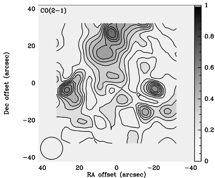
Figure 4.9: Integrated ^{12}\text{CO}(2-1) emission observed with the HERA receiver. The contour levels are between 0.410 to 4.10 K km/s in steps of 0.410 K km/s. The beam of 12'' is indicated at the bottom left.
