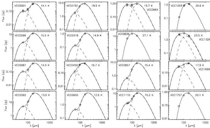
Figure 1.1: FIR SEDs for some spiral galaxies of the Virgo Cluster studied by Popescu et al. (2002). The two modified blackbody functions that fitted the data points (ISOPHOT data) are plotted with dashed lines. The temperature of the warm component is constrained to be 47 K. The fitted temperature of the cold component is marked in each plot, and the sum of the two fitting functions is plotted as the solid line. The galaxy VCC 1110 has additional measurements at 70 and 120 \mu\text{m} , and some galaxies do not show evidence for the two dust components (VCC 1757).
