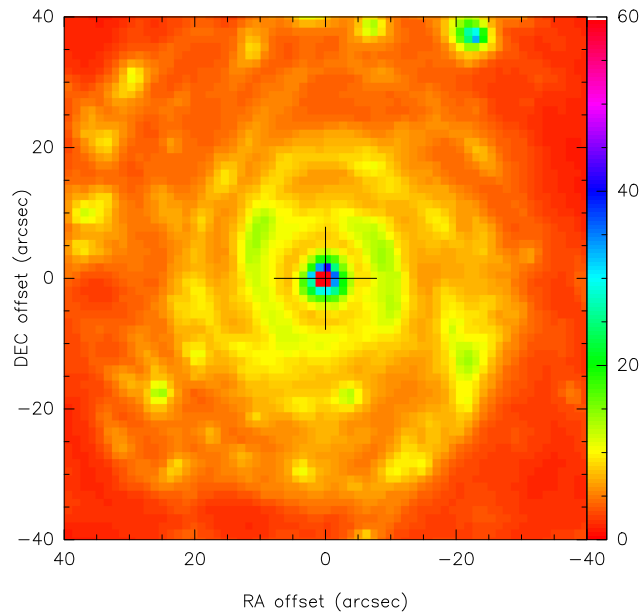
Figure 5.22: 8\ \mu\text{m} Spitzer image of NGC 3147. The central 80'' of the galaxy are shown. A ring structure around the nucleus is also apparent.
