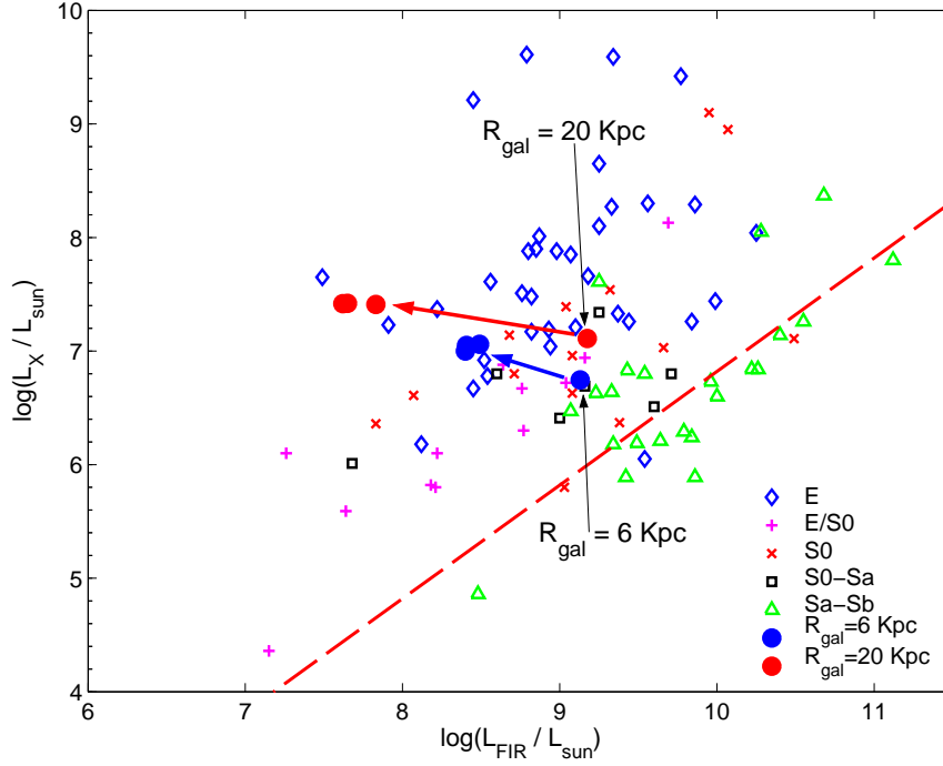
Figure 3.13: Models of the more massive galaxy of 1.6 \times 10^{11} M_{\odot} baryonic mass in the L_{FIR} vs. L_X diagram for various core radii r_c^{stars} and r_c^{gas} , plotted as filled circles. The thin arrows indicate the original model, while the thick arrows indicate the shift of the model for various core radii. We represented: E galaxies (empty diamonds), E/S0 galaxies (pluses), S0 galaxies (crosses), S0s galaxies (empty squares), Sa – Sb (empty triangles). The galaxy with \log L_X / L_{\odot} > 10 present in Fig. 3.8 is not plotted here.
