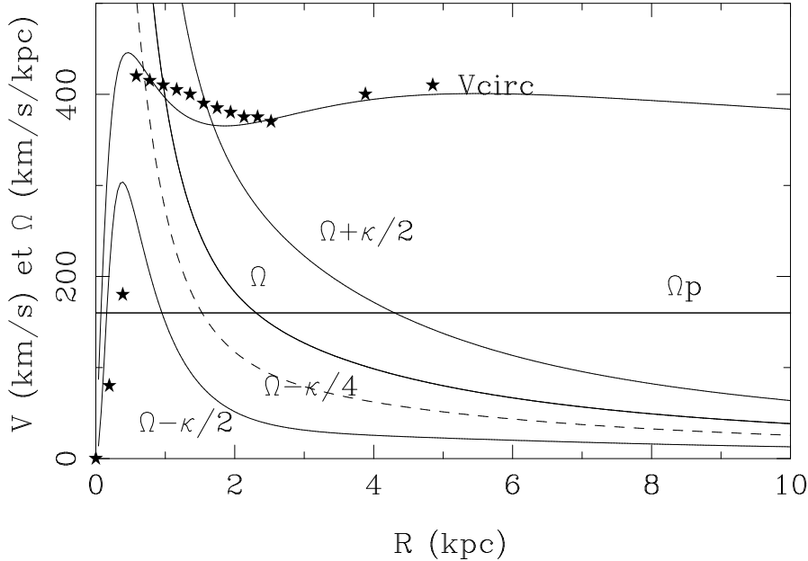
Figure 5.30: Model rotation curve and derived frequencies \Omega , \Omega - \kappa/2 and \Omega + \kappa/2 , for NGC 3147. The star symbols are the data derived from the CO kinematics, deprojected with an inclination of i = 29.5^\circ .
