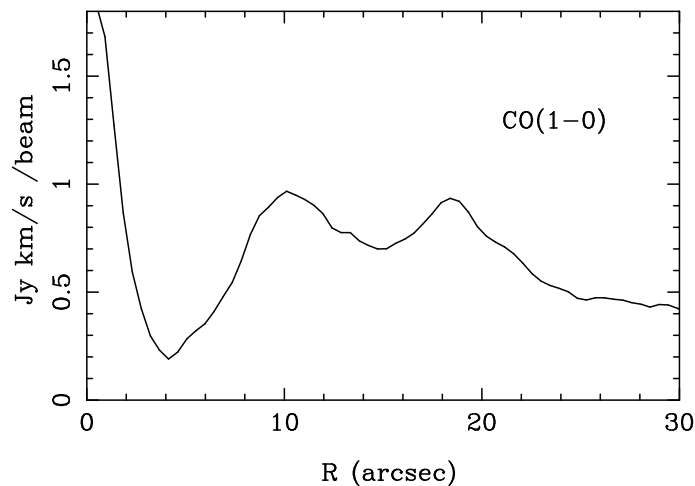
Figure 5.11: Radial distribution (azimuthal average, deprojected to face-on orientation) of the CO(1-0) intensity, shown in Fig. 5.10. This clearly shows the nuclear peak and two CO(1-0) emissions corresponding to the two rings shown in Fig. 5.10.
