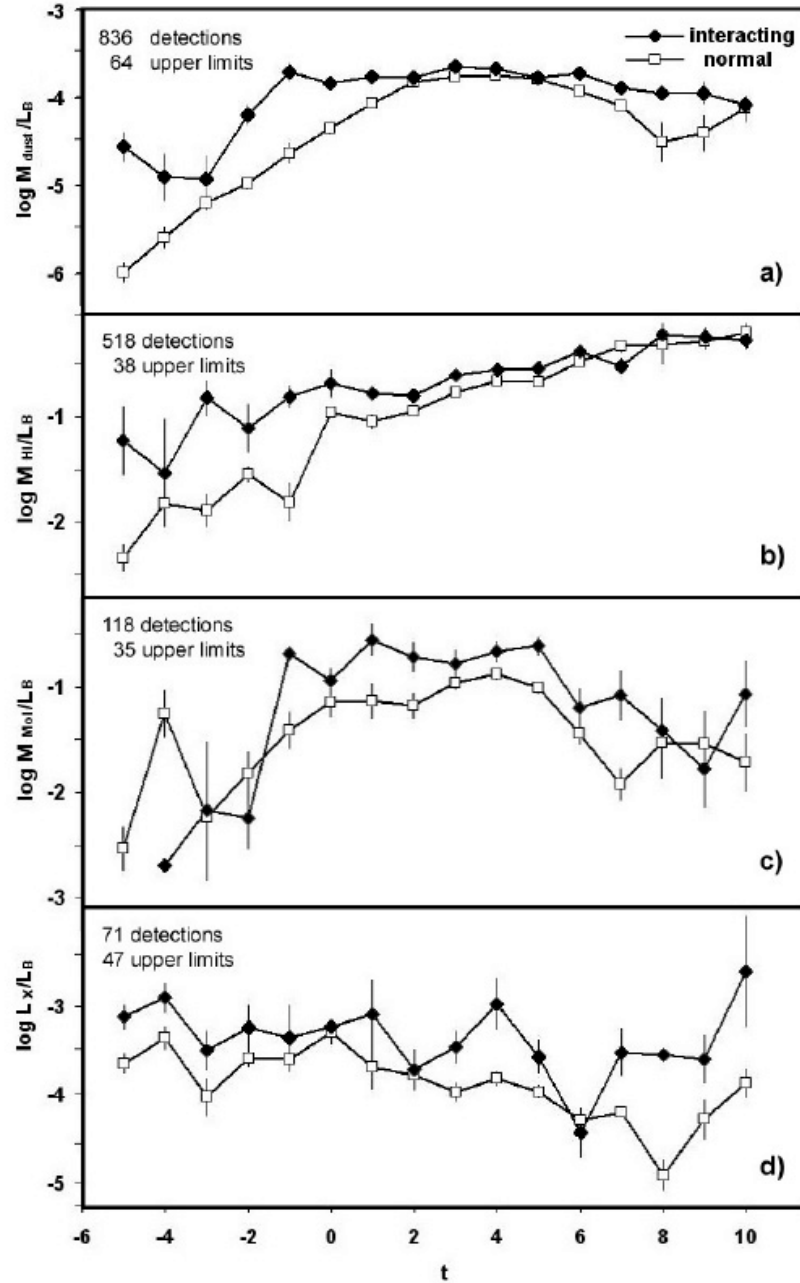
Figure 2.8: Comparison between mean values for interacting galaxies and corresponding means for normal galaxies (Bettoni et al., 2003) for dust, atomic gas, molecular gas, and hot gas component. Bars represent 1\sigma errors (by Casasola et al., 2004).
