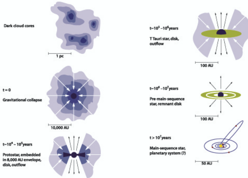
Figure 2.2: Phases of the star formation. Based on an original sketch by Frank Shu.
