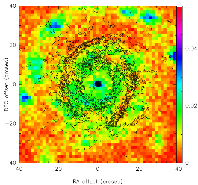
Figure 5.20: Superposition of the CO(1-0) contour levels shown in Fig. 5.10 and the FUV- GALEX image shown in Fig. 5.19. The central 80'' are shown. The CO inner ring agrees with the FUV one, the central 10'' -radius CO ring is slightly contained in the FUV circular region. But the more external ( 18'' -radius) CO pseudo-ring does not correspond at all with the FUV structures, although there is some overlap with the FUV ring (eastern part). The southwest CO emission appears to fall in the FUV interarm.
