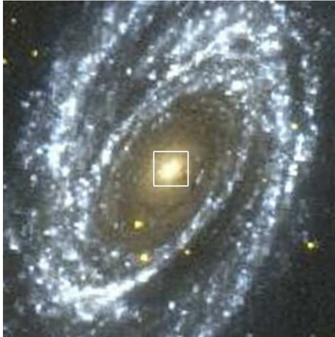
Figure 4.4: The field of our observations (white box, 80 arcsec in size) superposed on a GALEX composite image of M 81. In the figure, FUV is in the blue channel and NUV the yellow one.
