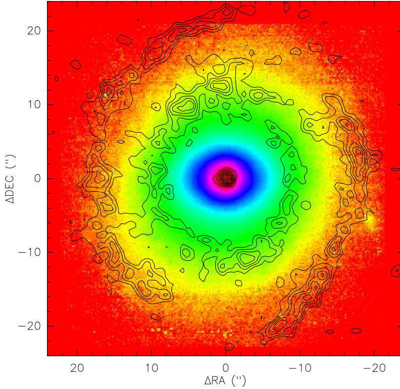
Figure 5.25: CO(1-0) linear contours (0.87 to 2.87 by 0.2 Jy km s -1 beam -1 ) superposed on the near-infrared J image, taken with the CFHT, in logarithmic levels. The nuclear bar of P.A. = 85° lies just inside the nuclear ring in the molecular gas. The major axis of the galaxy is at P.A. = 150°.
