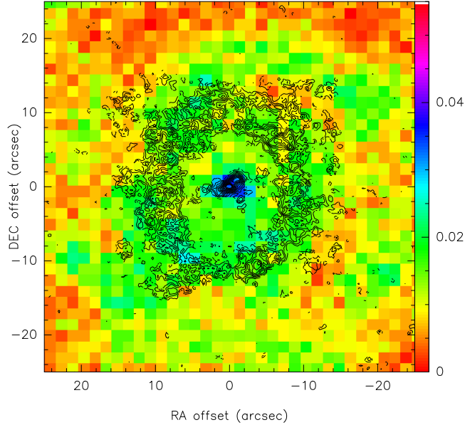
Figure 5.21: Superposition of the CO(2-1) contour levels shown in Fig. 5.12 and the FUV- GALEX image shown in Fig. 5.19. The central 50'' are shown. The CO(2-1) nuclear peak agrees with the FUV one, and the CO(2-1) ring is contained in the FUV- GALEX inner ring-like structure.
