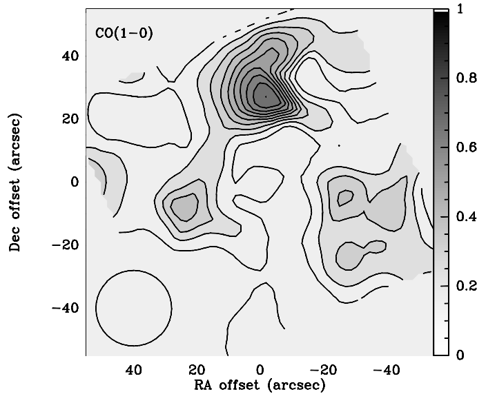
Figure 4.7: Integrated ^{12}\text{CO}(1-0) emission. The contour levels are between 0.701 to 7.01 K km/s in steps of 0.701 K km/s. The beam of 22'' is indicated at the bottom left.
