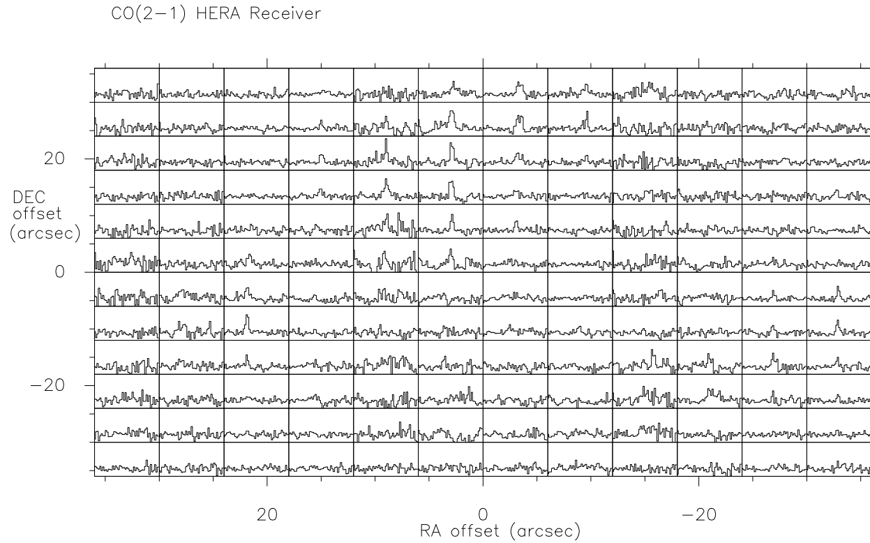
Figure 4.8: ^{12}\text{CO}(2-1) map of the M 81 central region observed with the HERA receiver. Each spectrum has a velocity scale from -600 to 600 \text{ km s}^{-1} and a temperature scale from -20 to 70 \text{ mK} . The positions are offsets relative to the M 81 nucleus assumed of coordinates \text{RA}_{J2000.0} = 09^{\text{h}} 55^{\text{m}} 33^{\text{s}} , \text{DEC}_{J2000.0} = 69^{\circ} 03' 55'' .
