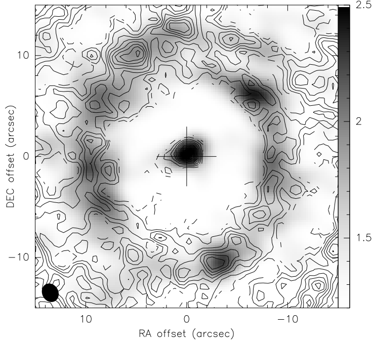
Figure 5.14: Contours of the ^{12}\text{CO}(1-0) map, same as Fig. 5.10, superposed with the grey scale ^{12}\text{CO}(2-1) map tapered and convolved to the same resolution and corrected for primary beam attenuation, in unit of \text{Jy}/\text{beam km s}^{-1} . The beam is plotted at the bottom left.
