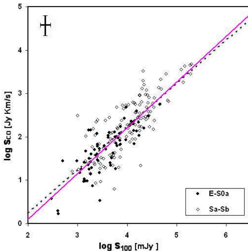
Figure 3.1: The relation between the CO(1-0) line flux and 100 \mu\text{m} one, plotted as a pink-full line, for early-type galaxies and early spirals from E to Sb. The representative points of galaxies are plotted with different symbols. The cross at the upper left of the figure represents the mean errors for the fluxes in the whole sample. For comparison, the relation found by Bregman et al. (1992) for a sample of early-type galaxies is shown as a dotted line.
