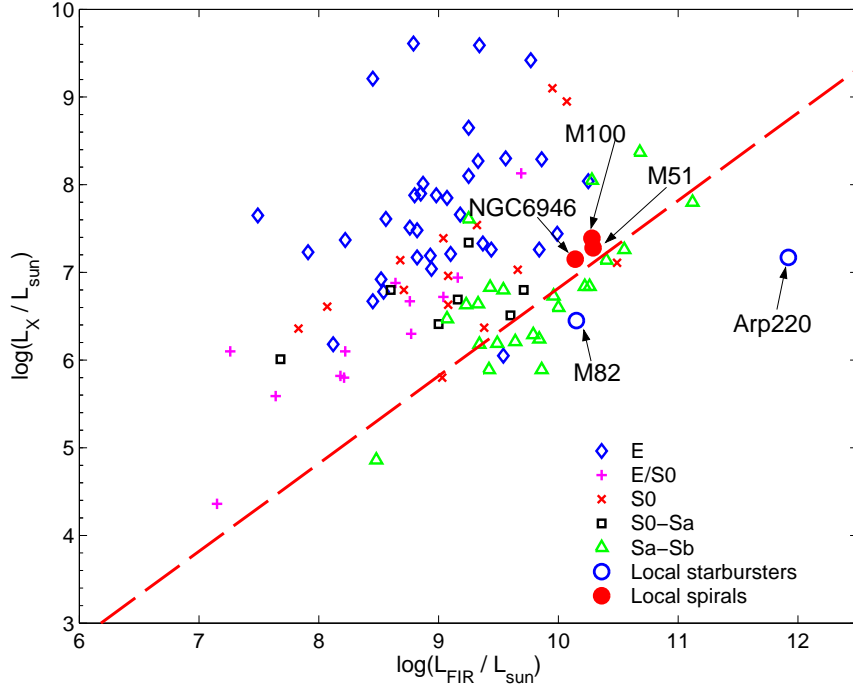
Figure 3.14: L_{FIR} versus L_X for galaxy models of spirals and starbursters. Five theoretical models, taken from Piovan et al. (2006), are represented: three spirals (M 100, M 51 and NGC 6946) and two starbursters (Arp220 and M82). Different morphological types are plotted as in Fig. 3.13. The galaxy with \log L_X / L_\odot > 10 present in Fig. 3.8 is not plotted here.
