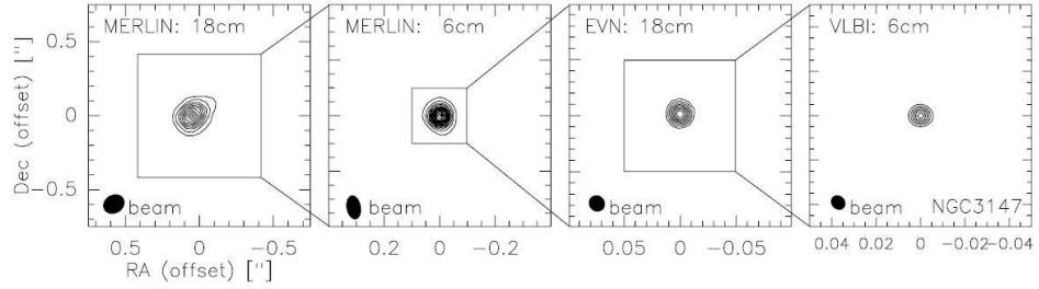
Figure 5.5: MERLIN (2 left columns) and EVN/VLBI (2 right columns) of the 18 cm and 6 cm continuum emission in NGC 3147 (Krips et al., 2007a). Contour levels are: ( 5\sigma )0.75 to 7.5 mJy/beam in steps of 5\sigma for MERLIN-18 cm (left), ( 3\sigma )0.72 to 10.1 mJy/beam in steps of 5\sigma for MERLIN-6 cm (left middle), ( 3\sigma )0.65 to 5.2 mJy/beam in steps of 5\sigma for EVN-18 cm (right middle), and ( 5\sigma )1.4 to 8.3 mJy/beam in steps of 5\sigma for EVN-6 cm (right).
