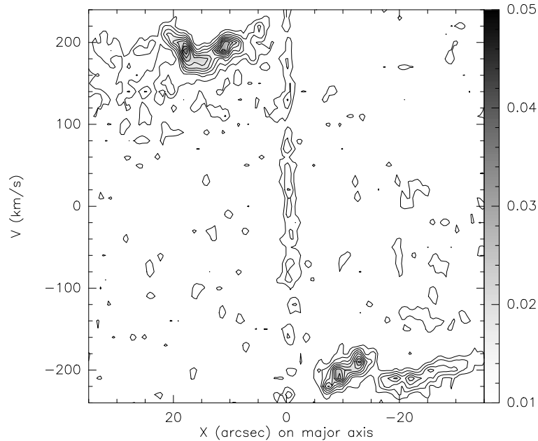
Figure 5.18: CO(1-0) position-velocity (p-v) diagram along the major axis of NGC 3147 using the whole velocity range \pm 240 \text{ km s}^{-1} with 49 channels in steps of 10 \text{ km s}^{-1} . The center (0,0), the heliocentric velocity, and P.A. used are given in Table 5.1. Contour levels are from 0.005 to 0.05 Jy/beam in steps of 0.005 Jy/beam.
