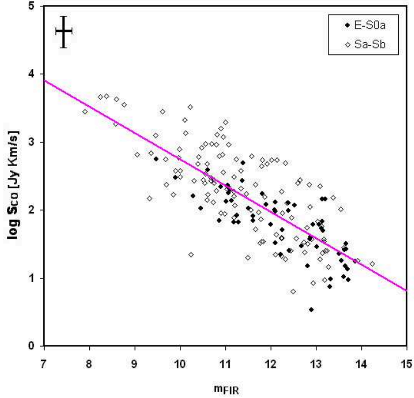
Figure 3.3: The relation between m_{FIR} and CO(1-0) flux, plotted as a pink-full line, for early-type galaxies and early spirals from E to Sb. The representative points of galaxies are plotted with different symbols. The cross at the upper left of the figure represents the mean errors for the fluxes in the whole sample.
