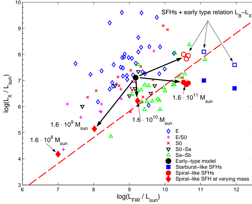
Figure 3.15: L_{FIR} versus L_X for galaxy models of fixed 1.6 \times 10^{11} M_\odot baryonic mass for various SFHs (large circles and squares) or at fixed SFH for various masses from 1.6 \times 10^8 M_\odot to 1.6 \times 10^{11} M_\odot (large filled diamonds). Large circles and squares represent, respectively, models with spiral-like SFH and starburst-like SFH. Large filled circles and squares are obtained using Eq. 3.4, while large open circles and squares depend on Eq. 3.10. Different morphological types are plotted as in Fig. 3.13. The galaxy with \log L_X/L_\odot > 10 present in Fig. 3.8 is not plotted here.
