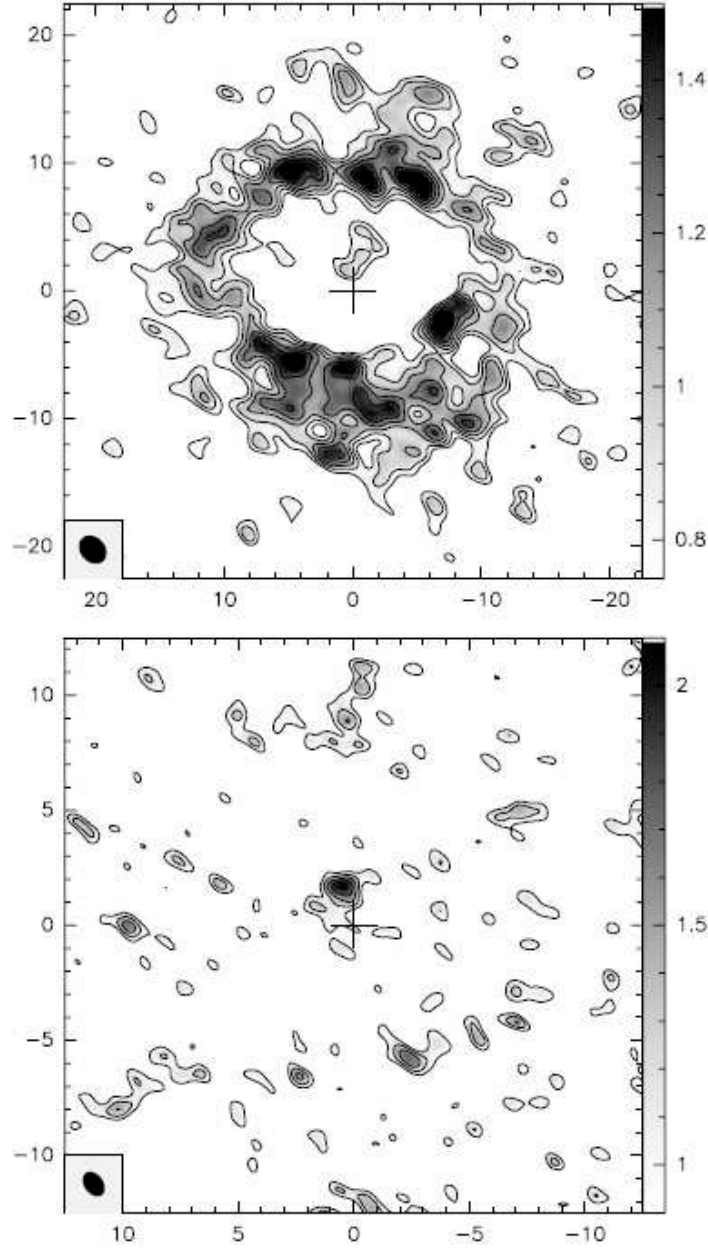
Figure 5.2: Upper panel: CO(1-0) integrated intensity contours observed with the IRAM interferometer toward the center of NGC 7217 (Combes et al., 2004). The cross marks the coordinates center. The rms noise is \sigma = 0.15 \text{ Jy km s}^{-1} \text{ beam}^{-1} . Contour levels are from 5\sigma to 10\sigma with 1\sigma spacing. The beam is plotted at the bottom left. Bottom panel: Same as Upper panel but for the CO(2-1) integrated intensity (Combes et al., 2004). The rms noise is \sigma = 0.3 \text{ Jy km s}^{-1} \text{ beam}^{-1} . Contour levels are from 3\sigma to 10\sigma with 1\sigma spacing. The beam is plotted at the bottom left.
