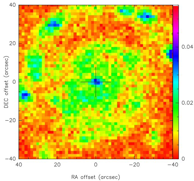
Figure 5.19: FUV- GALEX sky subtracted image of NGC 3147. The central 80'' of the galaxy are shown. A ring structure around the nucleus, even if incomplete, is evident.
