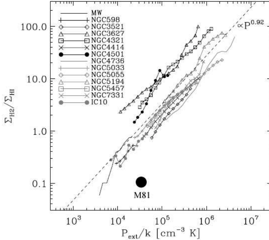
Figure 4.16: This figure, by Blitz & Rosolowsky (2006), shows that all galaxies have a similar scaling between the \text{H}_2/\text{HI} ratio and the hydrostatic pressure P_{ext} . Following the model of Blitz & Rosolowsky (2006) and assuming an \text{H}_2/\text{HI} ratio of 0.1 we found that M 81 differs by the behavior of the other galaxies with a rather high pressure.
