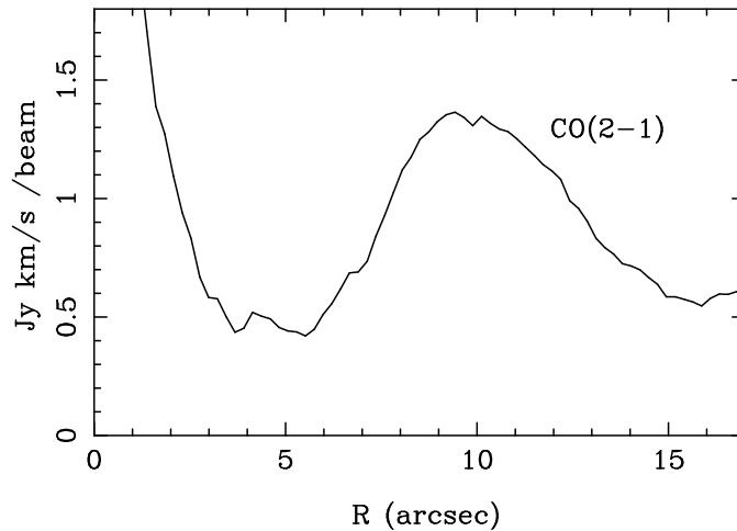
Figure 5.13: Radial distribution (azimuthal average, deprojected to face-on orientation) of the CO(2-1) integrated intensity, shown in Fig. 5.12. This figure clearly shows the central peak and the CO(2-1) emission at \sim 10'' corresponding to the inner ring of Fig. 5.12.
