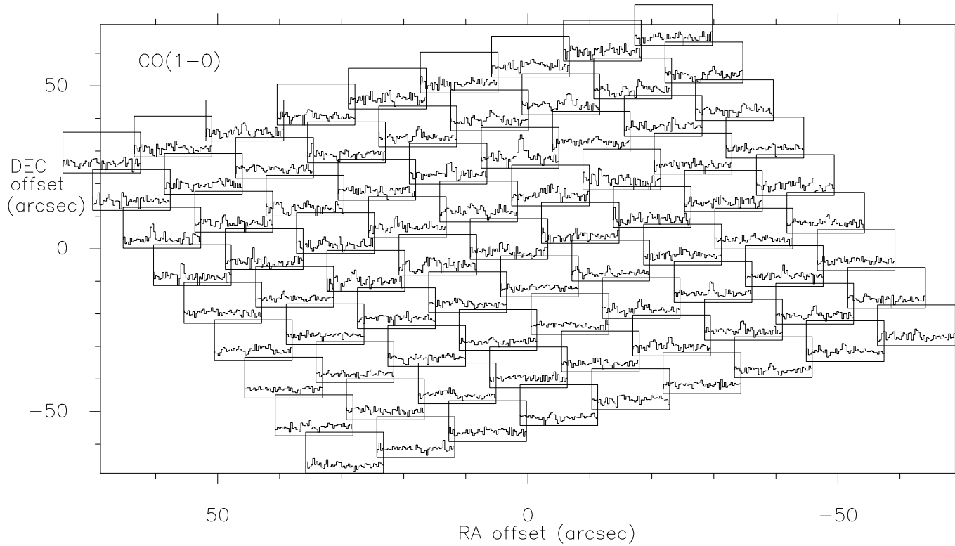
Figure 4.5: ^{12}\text{CO}(1-0) map of the observed M 81 central region. Each spectrum has a velocity scale from -600 to 600 \text{km s}^{-1} , and a temperature scale from -20 to 70 \text{mK} . The positions are offsets relative to the M 81 nucleus assumed of coordinates \text{RA}_{J2000.0} = 09^{\text{h}} 55^{\text{m}} 33^{\text{s}} , \text{DEC}_{J2000.0} = 69^{\circ} 03' 55'' .
