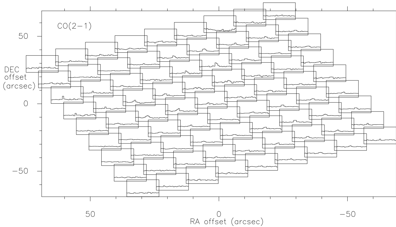
Figure 4.6: ^{12}\text{CO}(2-1) map of the observed M 81 central region. Each spectrum has a velocity scale from -600 to 600 \text{km s}^{-1} , and a temperature scale from -20 to 70 mK. The positions are offsets relative to the M 81 nucleus assumed of coordinates \text{RA}_{J2000.0} = 09^{\text{h}} 55^{\text{m}} 33^{\text{s}} , \text{DEC}_{J2000.0} = 69^{\circ} 03' 55'' . The ^{12}\text{CO}(2-1) observations are convolved to the ^{12}\text{CO}(1-0) beam resolution ( 22'' ).
