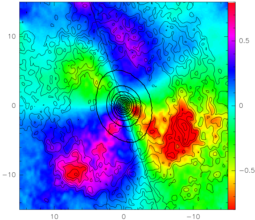
Figure 5.28: Same as Fig. 5.27 for the CO(2-1) emission taken as tracer of gas surface density.
