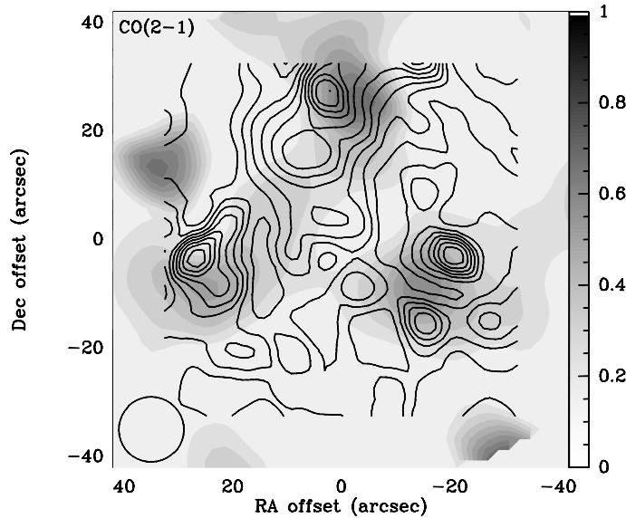
Figure 4.10: Integrated ^{12}\text{CO}(2-1) emission detected with the HERA receiver superposed on the ^{12}\text{CO}(2-1) emission found with A and B receivers. The contour levels are the same as shown in Fig. 4.9 between 0.410 to 4.10 K km/s in steps of 0.410 K km/s and the intensity levels detected with A and B receivers are in grey scale. The beam of 12'' is indicated at the bottom left. The intensity peaks detected with the two observing configurations agree quite well between them.
