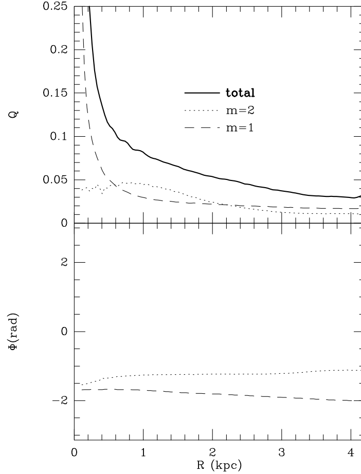
Figure 5.26: Strengths ( Q_1 , Q_2 and total Q_T ) and phases ( \phi_1 and \phi_2 ) of the m = 1 and m = 2 Fourier components of the stellar potential inside a field of 48'' in diameter ( r < 4.6 kpc). The bar strength extends up to 2 kpc in radius, and has a constant phase.
