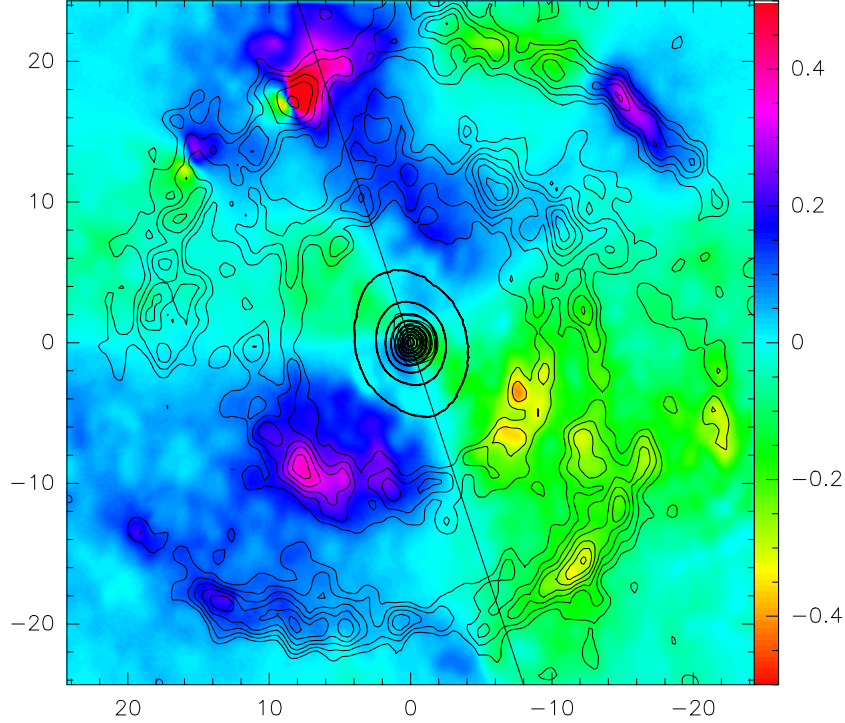
Figure 5.27: The CO(1–0) contours are overlaid onto the gravitational torque map ( t(x,y) \times \Sigma(x,y) , as defined in text) in the center of NGC 3147. The torque map (grey/color scale) is normalized to the maximum absolute value of the torques. The derived torques change sign as expected in a butterfly diagram, delineating four quadrants. The orientation of quadrants follow the bar orientation in NGC 3147. In this deprojected picture, the major axis of the galaxy is oriented parallel to the abscissa Ox . The inclined line reproduces the mean orientation of the bar (P.A. = 20^\circ on the projected image).
