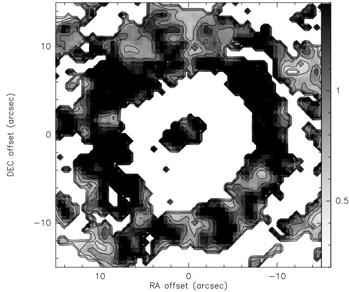
Figure 5.16: Contours and grey scale of the CO(2-1)/CO(1-0) ratio map. Contours are from 0.2 to 2 by 0.1
