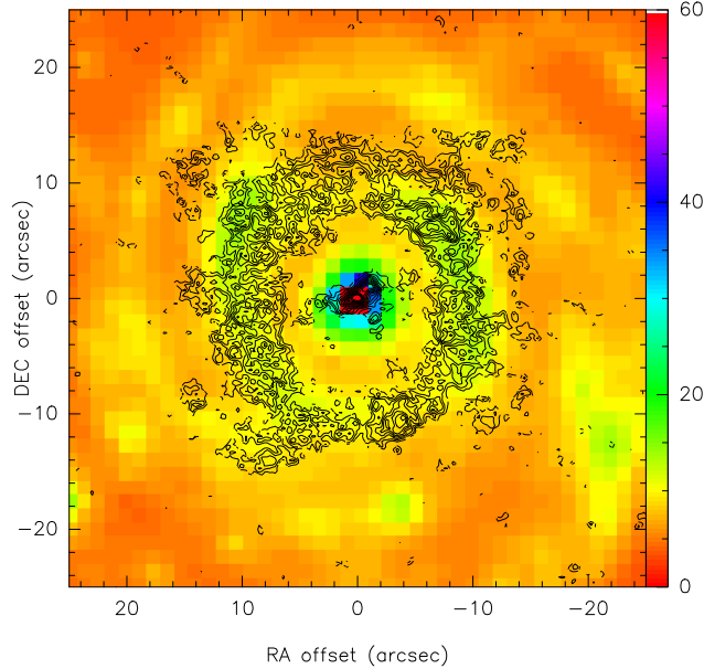
Figure 5.24: Superposition of the CO(2-1) contour levels shown in Fig. 5.12 and the 8 \mu\text{m} Spitzer/IRAC image shown in Fig. 5.22. The central 50'' are shown. There is a good agreement between the CO(2-1) ring and nuclear peak and IR ones.
