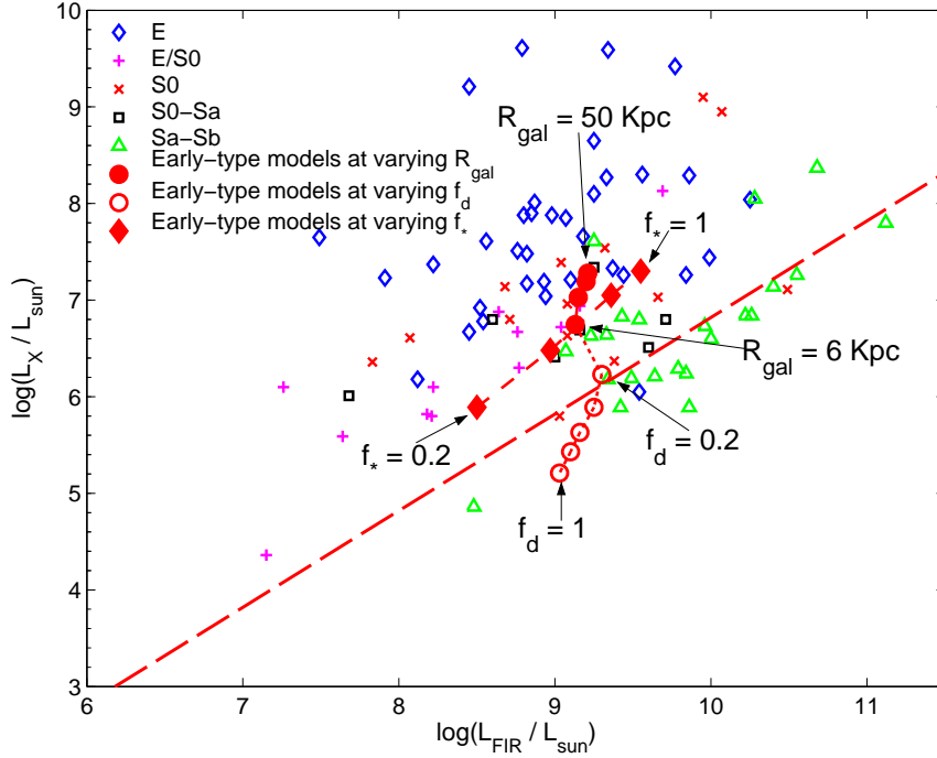
Figure 3.12: Models of the 1.6 \times 10^{11} M_{\odot} baryonic mass galaxy in the L_{FIR} vs. L_X diagram with the variation of the galactic radius (filled circles), the mass of stars (filled diamonds), and finally, the mass of gas (empty circles). We represented: E galaxies (empty diamonds), E/S0 galaxies (pluses), S0 galaxies (crosses), S0s galaxies (empty squares), Sa-Sb (empty triangles). The galaxy with \log L_X / L_{\odot} > 10 present in Fig. 3.8 is not plotted here.
