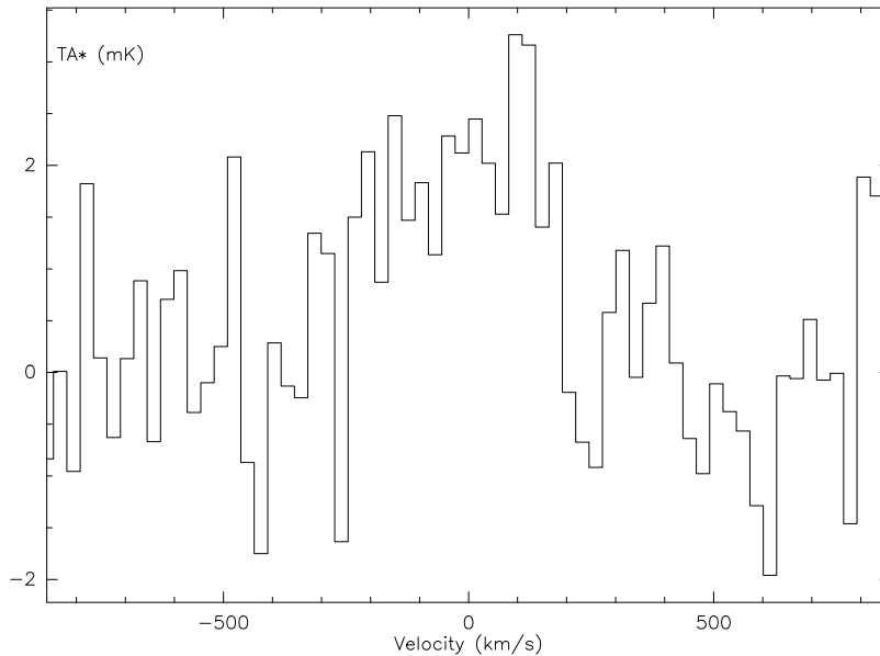
Figure 5.8: Average HCN(1-0) spectrum towards the center of NGC 3147, over the 9-point map made with the IRAM 30 m with 7'' spacing. The HCN is detected, but with a low HCN/CO ratio, of 0.05.
