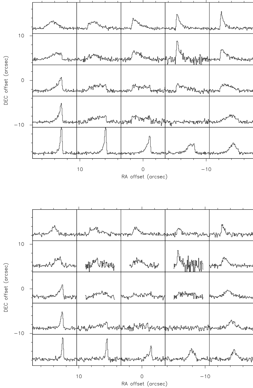
Figure 5.7: Spectra maps of NGC 3147 made with the IRAM 30 m with 7'' spacing in CO(1-0) (top) and CO(2-1) (bottom). The positions are offsets relative to the NGC 3147 center, whose coordinates are listed in Table 5.1. Each spectrum has a velocity scale from -500 to 500 \text{ km s}^{-1} , and an antenna temperature scale ( T_A^* ) from -0.05 to 0.25 \text{ K} for CO(1-0) and 0.20 \text{ K} for CO(2-1).
