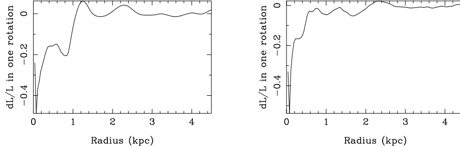
Figure 5.29: The torque, or more precisely the fraction of the angular momentum transferred from/to the gas in one rotation— dL/L —are plotted for CO(1-0) ( left ), and CO(2-1) ( right ). The curve is more noisy for the CO(2-1), because of the clumpiness of the map, but both show negative torques inside 1 kpc in radius, and positive outside.
