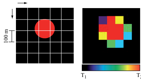
FIGURE 4.13. a) Sketch for the calculation of the number of pixels with an effective temperature above the background as a function of viewing configuration of a given thermal anomaly associated with a pit. The white grid indicates footprints of THEMIS-IR pixels. The grid is displaced in both direction to reproduce all possible configurations. b) Result of the simulation for a given offset : representation of the effective temperature at THEMIS resolution.
