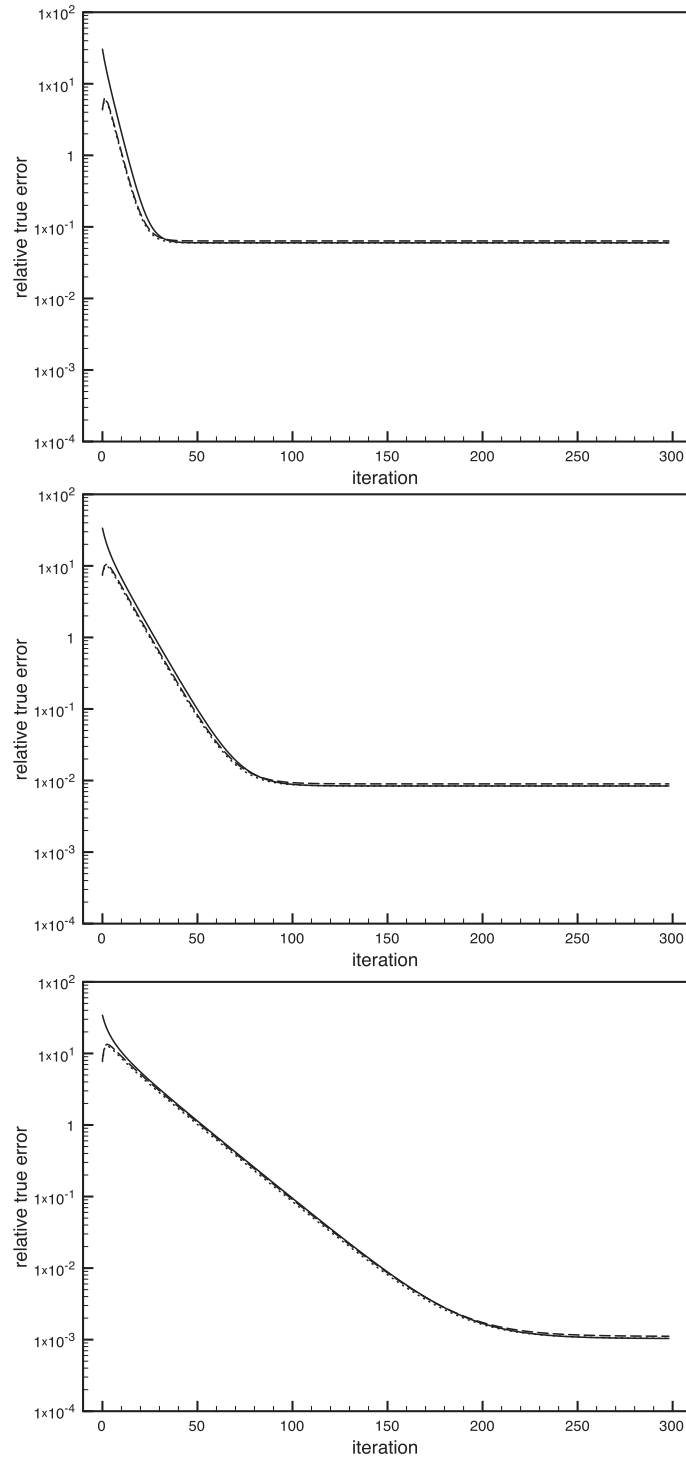
Figure 4.1: Variation of the relative true error with the iteration number of the surface value of the upper term invariants \rho^0(J = 1, J' = 1) (solid line), \rho^2(J = 1, J' = 1) (dashed line), and \rho^3(J = 1, J' = 2) (dotted line). From up to bottom, the panels show the error variation on the grids with 3, 5.9, and 11.7 PPD (see Subection 4.3.1). The plateaus in the later iterations indicate that the truncation error is reached. The convergence is slower for the grids with smaller meshes. The error of solution in the finest grid is about 0.1% and it is almost the same for both population and coherence multipoles. As an initialization of the model, I always use the LTE populations of the levels.
