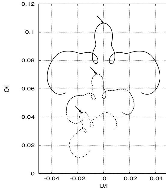
Figure 2. Hanle diagram of the emergent radiation observed at \beta = 37^\circ (right branch) and \beta = 143^\circ (left branch; see Figure 1). Solution for three different line-center optical thicknesses of the slab are plotted: T = 0 (solid line), T = 1 (dashed line), and T = 3 (dash-dotted line). The integral fractional linear polarization in Q/I and U/I are calculated for the magnetic field intensity varying between \gamma = 0 (pointed by the arrows) to \gamma = 2.8 in all plots (see Eq. (3.63) of Landi Degl’Innocenti & Landolfi (2004) for the definition of \gamma ).
