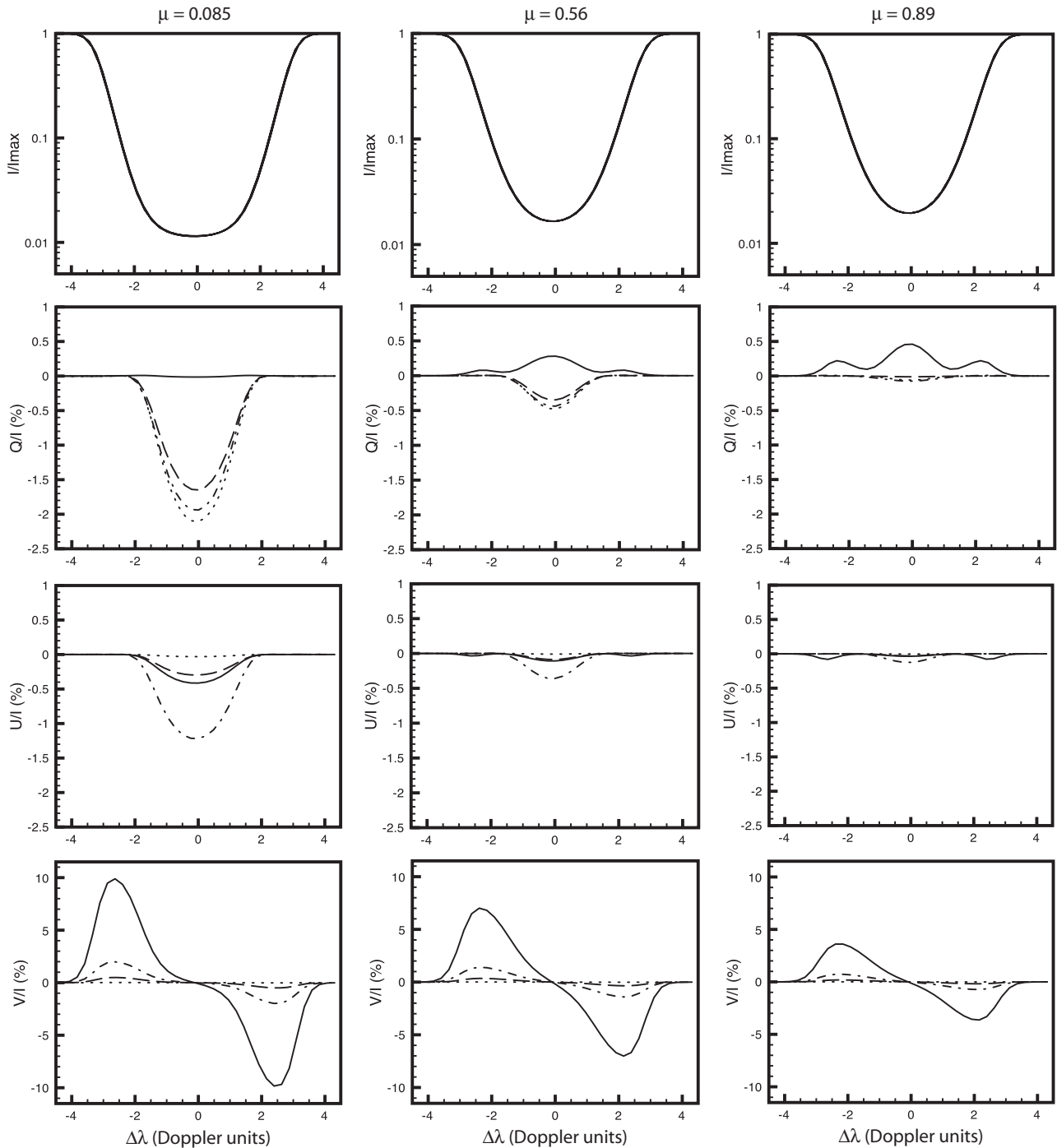
Figure 4.12: Stokes profiles of the ^3S - ^3P triplet observed at azimuth \chi - \chi_B = 0^\circ . The observation is made close to the limb ( \mu = 0.085 , left column), at \mu = 0.56 (central column), and close to the disk centre ( \mu = 0.89 , right column). The profiles have been synthesized for four different magnetic field strengths: \gamma = 0.01 (dotted line), 0.3 (dashed line), 1.2 (dash-dotted line), and 6.0 (solid line). The intensity profiles are not significantly modified by the Zeeman splitting of the strength considered. The Stokes-V profiles are not perfectly antisymmetric since there is a small contribution of symmetric component due to the alignment-to-orientation mechanism (Landi Degl’Innocenti & Landolfi 2004). However it is only small contribution in the present configuration. Note that negative Q corresponds to the linear polarization parallel with the limb.
