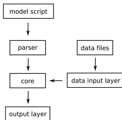
Figure A.1: Monopost code design.
