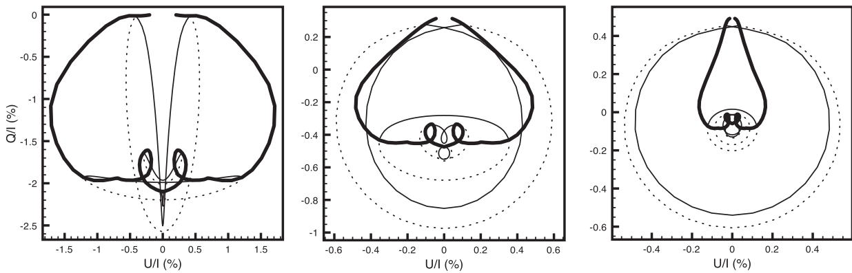
Figure 4.11: Hanle diagrams for the line centre of the {}^3S - {}^3P triplet observed at \mu = 0.085 (left panel), 0.56 (central panel), and 0.89 (right panel) and horizontal magnetic field. Thick line in each diagram corresponds to a fixed line-of-sight azimuth with respect to magnetic field vector: \chi - \chi_B = 0^\circ (left branch), and \chi - \chi_B = 180^\circ (right branch). Thin lines correspond to a fixed magnetic field strength of \gamma = 0.01, 0.3, 1.2, and 6.0 . Solid parts of the curves correspond to 0^\circ \leq \chi - \chi_B \leq 180^\circ , dotted lines correspond to the case 180^\circ \leq \chi - \chi_B \leq 360^\circ . As expected, polarization degree decreases towards the disk centre. However, a non-negligible amount of linear polarization is present even in the disk centre. Note the various scaling of the axes.
