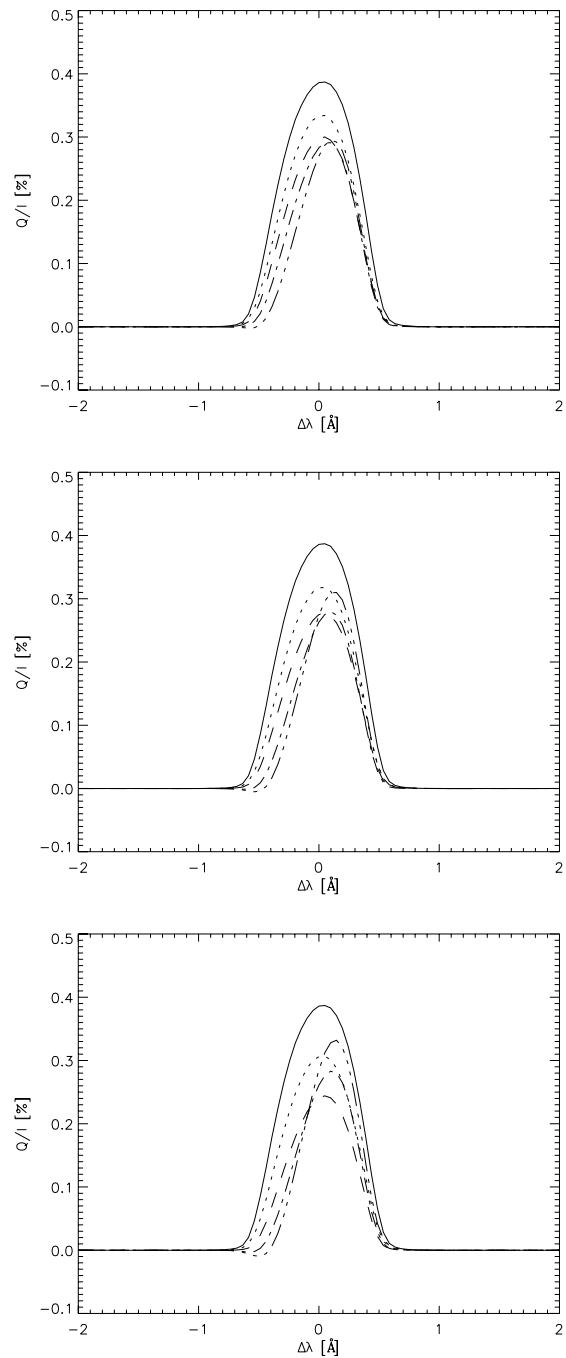
Fig. 9. Same as Fig. 8; here for the VAL F model.
