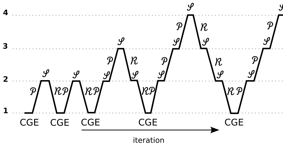
Figure 4.9: Nested MG iteration for an example of 4 grids.
