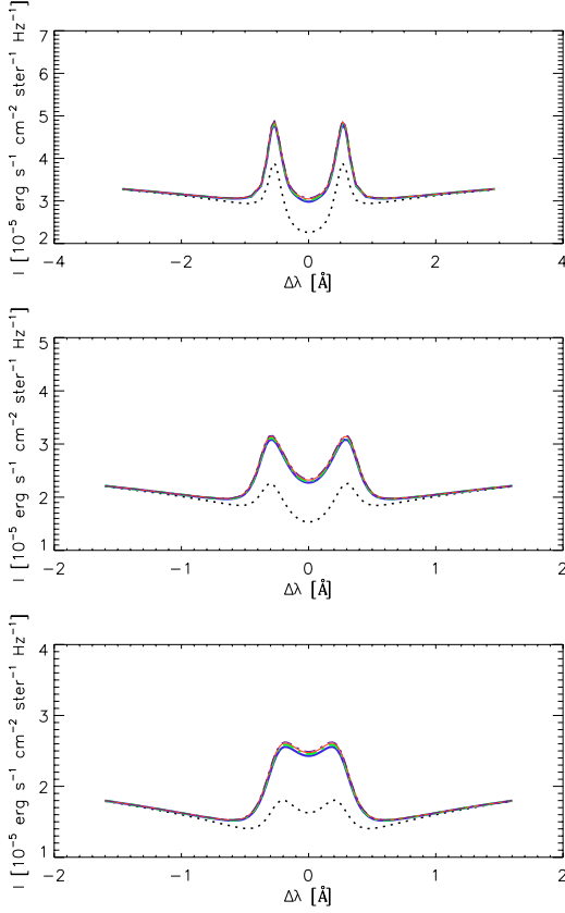
Fig. 1. From upper panel: H\alpha , H\beta , and H\gamma disk-center line profiles for \mathcal{F}_1 = 0 (dotted line, black), \mathcal{F}_1 = 4 \times 10^{11} (thick solid line, blue), 6 \times 10^{11} (thick dash-dotted line, green), 8 \times 10^{11} (thin solid line, red), and 1.0 \times 10^{12} (thin dash-dotted line, violet) \text{erg cm}^{-2} \text{s}^{-1} . No return-current effects are taken into account. Note that nonthermal profiles almost overlap in this range of beam fluxes.
