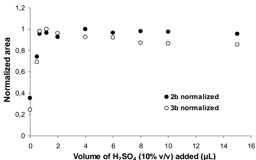
Fig. 3. Addition of variable volumes of H 2 SO 4 10% (v/v) and effect on the peak area of 2b and 3b measured after 36h reaction times. Areas were normalized to the largest peak area observed. Initial conditions : [GL] = 71 nM, [MG] = 81 nM, [1] = 2.6 \mu\text{M} .
