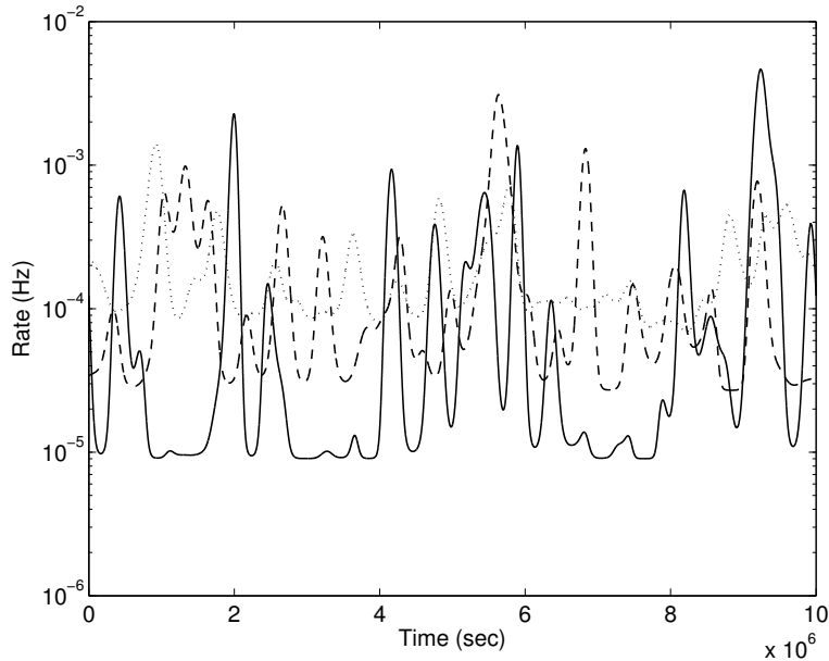
Figure 6.4: Shown are the generated rate fluctuations with time scale T_F = 10^5 sec and three amplitude factors: A = 1 for the dotted line, A = 2 for the dashed line, and A = 3 for the solid line. In all three cases the mean rate is 2 \times 10^{-4} Hz.
