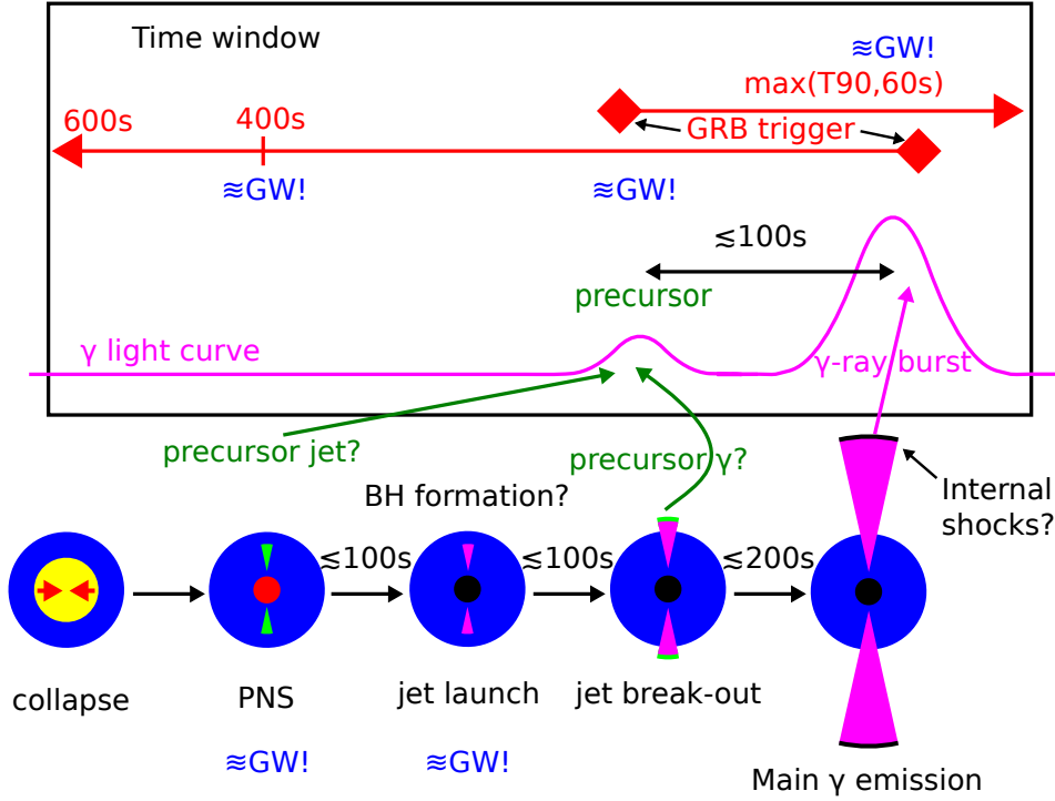
Figure 4.4: A graphical summary of the discussion in sections 4.3.2 and 4.3.3 of the gravitational wave coincidence window around the GRB trigger time for the stellar collapse model of long GRBs. The bottom part shows the stellar evolution with the formation of a relativistic jet and the possible emission times of \gamma -rays and gravitational waves. The middle part shows a fiducial \gamma -ray light curve where the \gamma -ray detector may trigger either on a precursor or on the main emission peak. The top part shows the discussed time window choice and the gravitational wave emission times compared to the \gamma -ray light curve.
