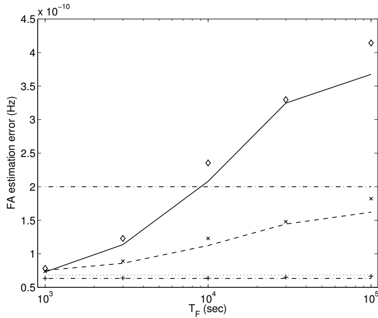
Figure 6.5: The dotted, dashed and solid lines are the theoretical predictions of the standard deviation (6.30) for respectively A = 1 , A = 2 , and A = 3 as a function of the rate fluctuation time scale T_F . The plus, cross and diamond markers denote the Monte Carlo standard deviation (6.29) for respectively A = 1 , A = 2 , and A = 3 . The upper dot-dashed line is the desired false alarm rate \alpha = 2 \times 10^{-10} Hz, and the lower dot-dashed line is the contribution of Poisson error (6.11) only for R = 10^4 time slides. The parameters used are: \alpha_1 = 2 \times 10^{-4} Hz, \alpha_2 = 5 \times 10^{-5} Hz, \Delta t = 20 ms, and a T = 10^7 s. The maximization over P is done on a discrete grid from 20 to 10000 with logarithmic steps. 1000 trials are used for the Monte Carlo simulations.
