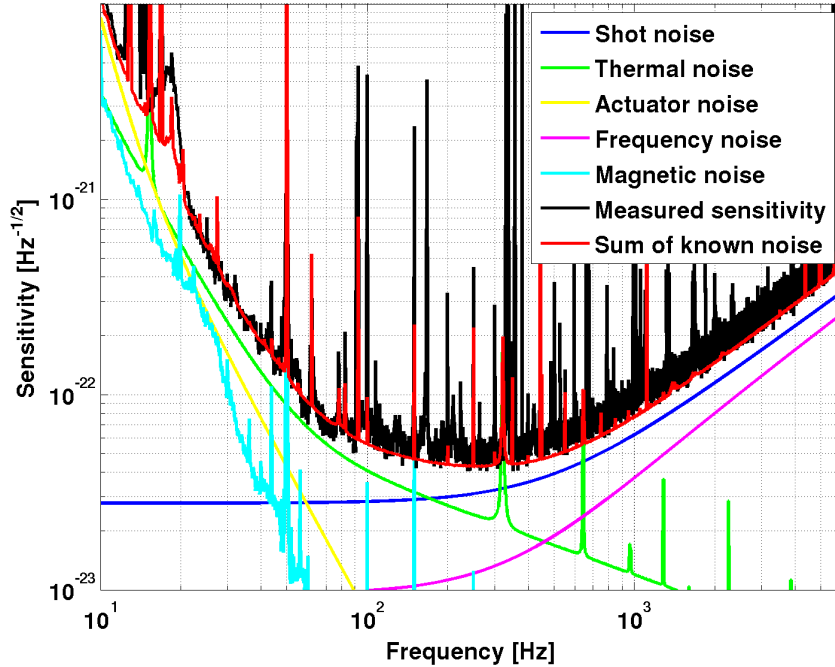
Figure 2.7: Real noise budget for Virgo during VSR2. Only the main contribution to the noise are shown. As shown by the difference between the measured sensitivity and sum of known noises, most of the noise in the interferometer is understood and well modeled.
