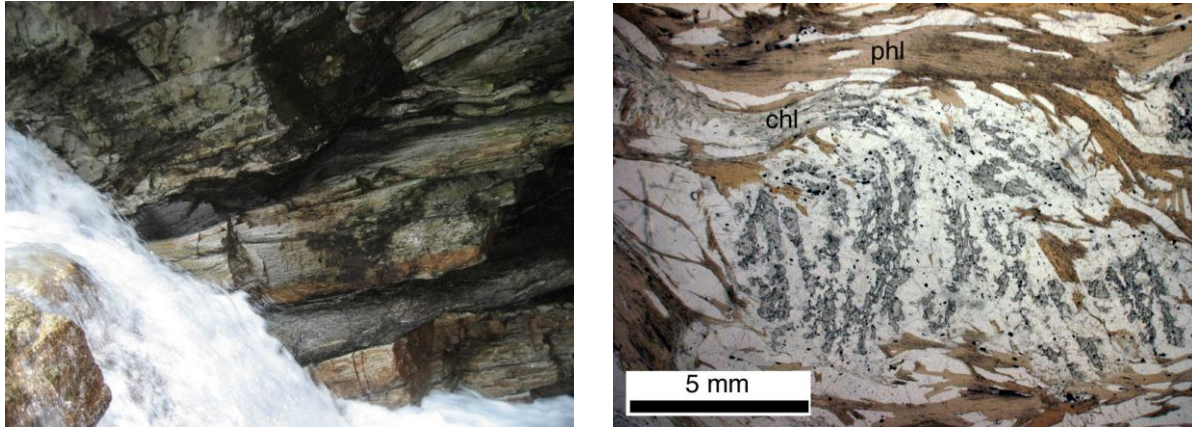
Fig. 4 : (a) Shear zones within granitoid orthogneisses in Val d'Ambra (Val Leventina, Ticino, Switzerland). (b) An example of a Mg-rich rock from one of the shear zones on (a), collected during the 2009 mission. A syntectonic kyanite porphyroblast (with numerous inclusions of rutile), partly replaced by cordierite a wrapped by a phlogopite+Mg-chlorite-bearing foliation.
