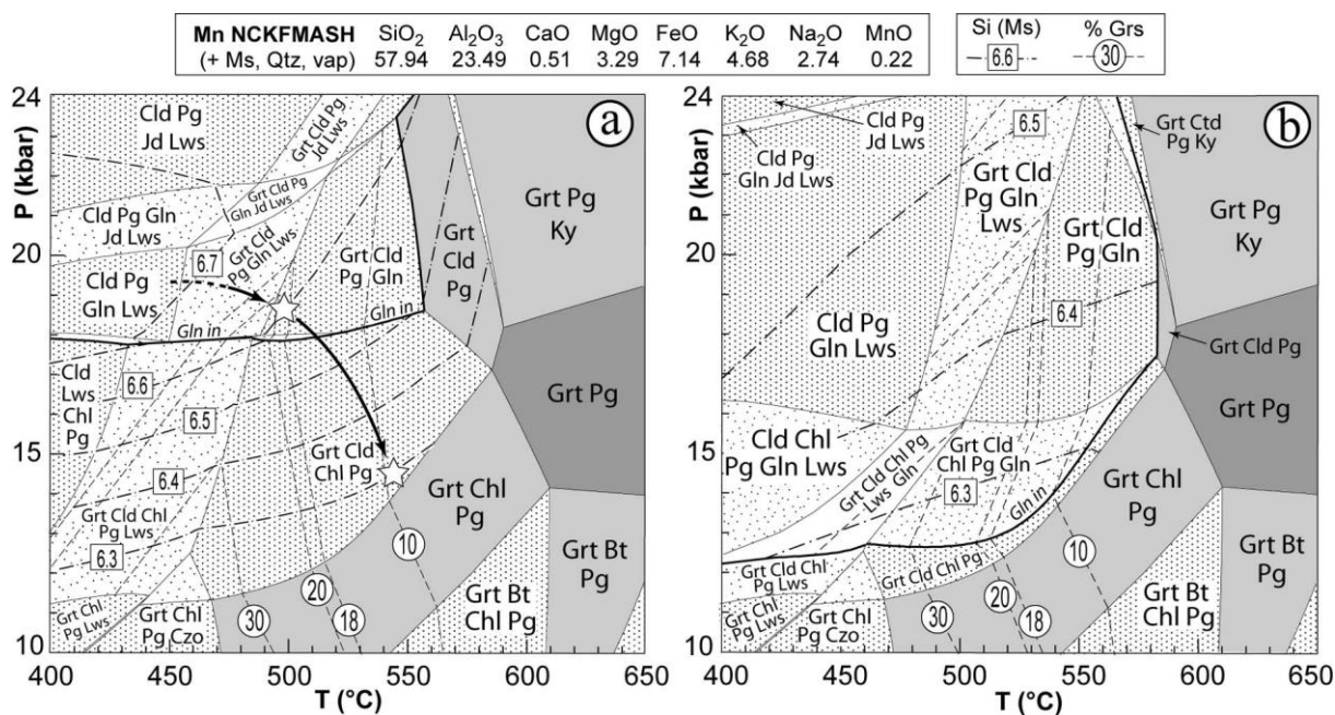
Fig. 18: P-T pseudosections calculated for a garnet+chloritoid+paragonite±chlorite -bearing metapelite from the Gran Paradiso massif (Le Bayon et al. 2006) (cf. Fig. 2; 7) using the glaucophane mixing model of (a) Wei et al. (2003) and (b) Dale et al. (2005) and contoured with compositional isopleths. Using the model of Wei et al. (2003) allows to account for the observations and propose a P-T evolution for the sample (a). On the other hand, the new model strongly extends the glaucophane stability field and results in a topology and position of the compositional isopleths incompatible with the observations (b).
