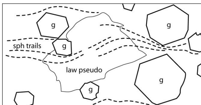
Fig. 11: Microphotograph and an interpretative drawing of a fine-grained blueschist from Ile de Groix (described in Ballèvre et al., 2003). The matrix foliation is defined by glaucophane, epidote and titanite ('sph trails'). It wraps gently around lozenge-shaped white aggregates (cf. Fig. 10) that are irregularly dispersed in the rock, do not show a preferential shape orientation, and are interpreted as pseudomorphs after lawsonite ('law pseudo'). This indicates that some ductile deformation took place during or after the growth of lawsonite. The pseudomorphs consist of an aggregate of paragonite, chlorite and epidote. They also contain glaucophane, garnet (g) and titanite (sph). Glaucophane crystals, titanite and some of the epidote grains are aligned parallel to each other, and define an internal schistosity ('sph trails'), interpreted as a relic foliation that has been overgrown by the pseudomorphed porphyroblasts (cf. Fig. 10). This internal foliation is slightly curved and continuous with the matrix foliation, suggesting that lawsonite grew syn-kinematically in a foliated matrix containing glaucophane, epidote and garnet.
