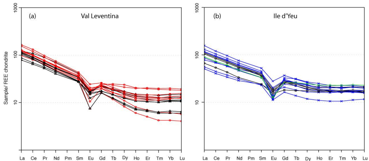
Fig. 5 : Chondrite-normalized (Boynton 1984) REE patterns of the granitoid orthogneisses (black) and Mg-rich shear zone rocks (red and blue) from (a) Val Leventina and (b) Ile d'Yeu. The similarities between the patterns of the shear zones and the orthogneisses and between the two distant localities are striking.
