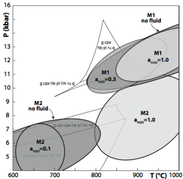
Fig. 26: Results of average P-T calculations (multi-equilibrium geothermobarometry) performed at different activities of H 2 O. Uncertainty ellipses are drawn at the 2σ level. For comparison, contours of the stability fields of the primary (M1) and secondary (M2) assemblages, based on Figs. 24 and 25, are also represented. In spite of the large uncertainties, the diagram shows a good coherence of this approach with that based on phase diagrams, if the absence of fluids (low H 2 O activity), suggested by the symplectitic character of the secondary textures, is taken into account.
