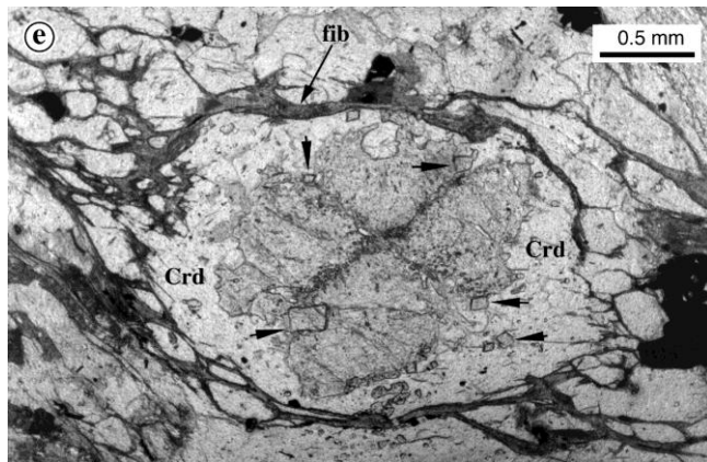
Fig. 1: Subhedral crystal of chiastolitic andalusite, surrounded by cordierite and wrapped by a fibrolitic sillimanite (fib)-bearing foliation (Marble Hall, Transvaal, Pitra and de Waal 2001). It contains relatively coarse inclusions of prismatic sillimanite, pointed by black arrows (besides the tiny inclusions of quartz and graphite defining the chiastolite cross). A straightforward interpretation of the crystallisation sequence would be: prismatic sillimanite → andalusite → cordierite → fibrolitic sillimanite. This would imply a complex P–T path involving
