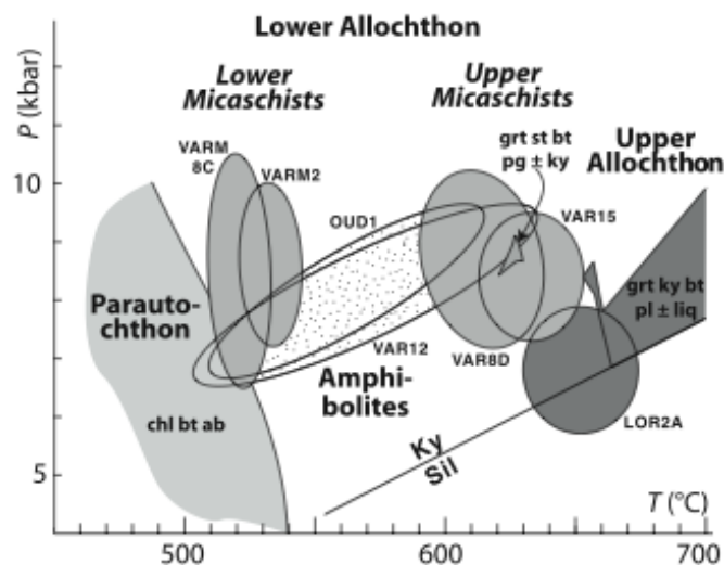
Fig. 23: Graphical representation of the results of the PT estimation. The ellipses correspond to the 1\sigma uncertainties on 'average PT' results as calculated by THERMOCALC. Other fields refer to the stability domains of the pertinent assemblages as deduced from the PT pseudosections (Pitra et al. 2010a).
