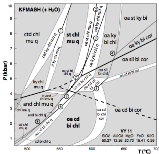
Fig. 28: P–T pseudosection for the analysed composition of the cordierite+gedrite (oa) gneiss. Both, the primary and the secondary assemblages are highlighted. The secondary assemblage (oa-cd-bi-chl) testifies to a post-deformational equilibration at <4 kbar, \approx 550^\circ\text{C} . Conversely, the primary, staurolite-bearing assemblage, contemporaneous with the formation of the shear zone, crystallised at higher pressures, indicating a barrovian-type metamorphism, characteristic of continental collision.
