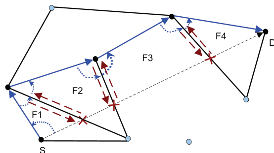
Figure 2.4: In blue the right hand rule and in red the face changes, two principles composing the face traversal on a planar graph used in GFG and GPSR algorithms strategies
