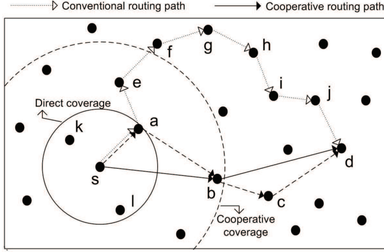
Figure 5.2: Multihop sensor network with cooperative geographic routing.
