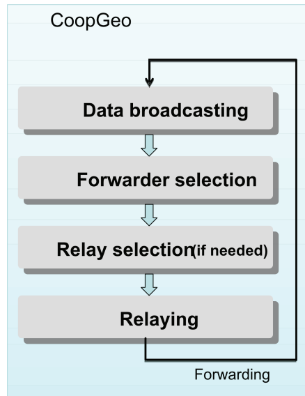
Figure 4.3: CoopGeo architecture
