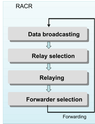
Figure 5.3: RACR Architecture.
