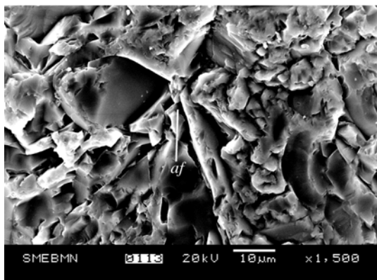
e - Aeolian feature ( af )
