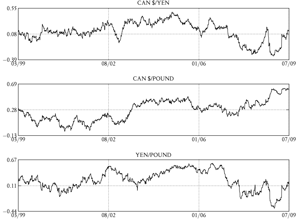
FIGURE 3.4 – Estimated correlations of diagonal DCC.
