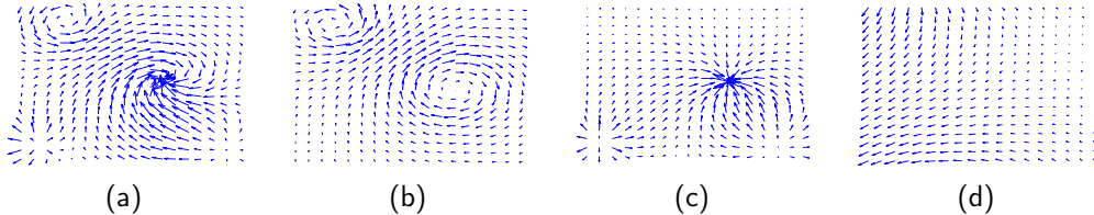
FIGURE 1.1 – Helmholtz decomposition (a) : a motion field ; (b) its solenoidal part ; (c) its irrotational part ; (d) its harmonic part
