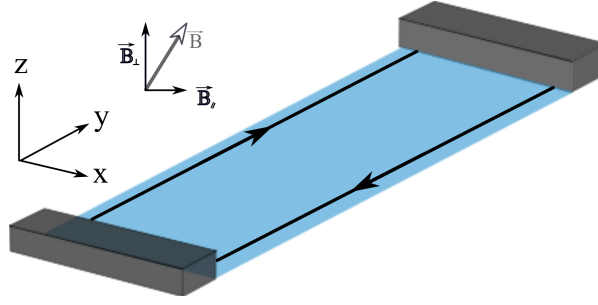
Figure B.1: The different contributions to the total magnetic field. In the absence of the component parallel to the 2DEG plane, the admittance and plasmon scattering matrices are symmetric.
