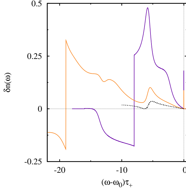
Figure 5.11: Excess occupation number for the closed channel model, at increasing injection energy, for strong coupling \theta = \pi/2 and \gamma = 0.2 . The dashed line indicates the fourier transform of the total decoherence coefficient.
