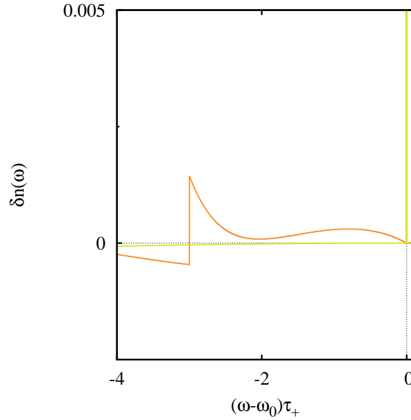
Figure 5.8: Excess occupation number for the closed channel model at low injection energy. At low ( \theta = 0.1 ) and strong ( \theta = \pi/2 ) coupling. \gamma = 0.2 in both cases
