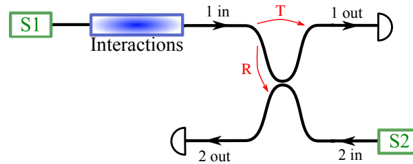
Figure 6.10: Sketch of a Hong Ou Mandel setup in the presence of an interacting region. The two single shot sources S1 and S2 feed the two branches of the interferometer. An interacting region is present in the first incoming channel, and a controlled time delay \Delta\tau is introduced on the second branch. Current correlations are measured on output of the interferometer.
