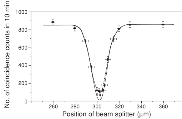
Figure 6.9: Hong Ou Mandel correlation dip for photons at zero delay time (taken from [71]).
