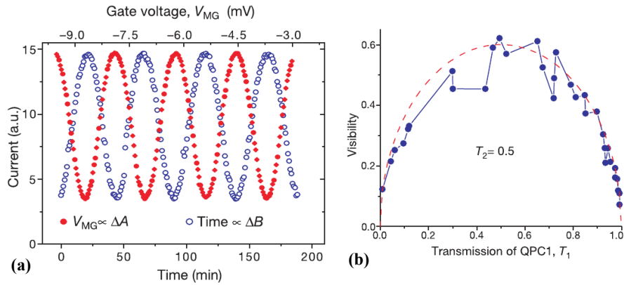
Figure 1.8: Figures taken from [74]. (a) Oscillations in the output current are manifestations of quantum coherence. (b) Visibility of the interference pattern. The reduction of the visibility is a manifestation of the decoherence of electronic excitations, and have motivated a significative amount of theoretical propositions.
