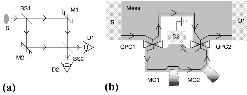
Figure 1.7: Figures taken from [74]. (a) Optical Mach-Zehnder interferometer. (b) Electronic analogue : the quantum point contacts are beamsplitters, in which the electron beams, namely the edge channels, split up and recombine.
