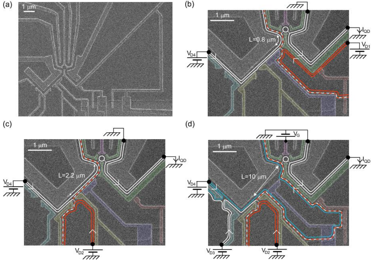
Figure 4.3: (from [145]) (a) : Overview of the setup for relaxation studies. Here, the different paths having different propagation lengths are represented in (b), (c) and (d).
