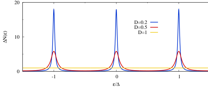
Figure 3.6: Density of states of the quantum dot as a function of \epsilon/\Delta (in units of \Delta ), for different values of the transparency D of the tunnel barrier.
