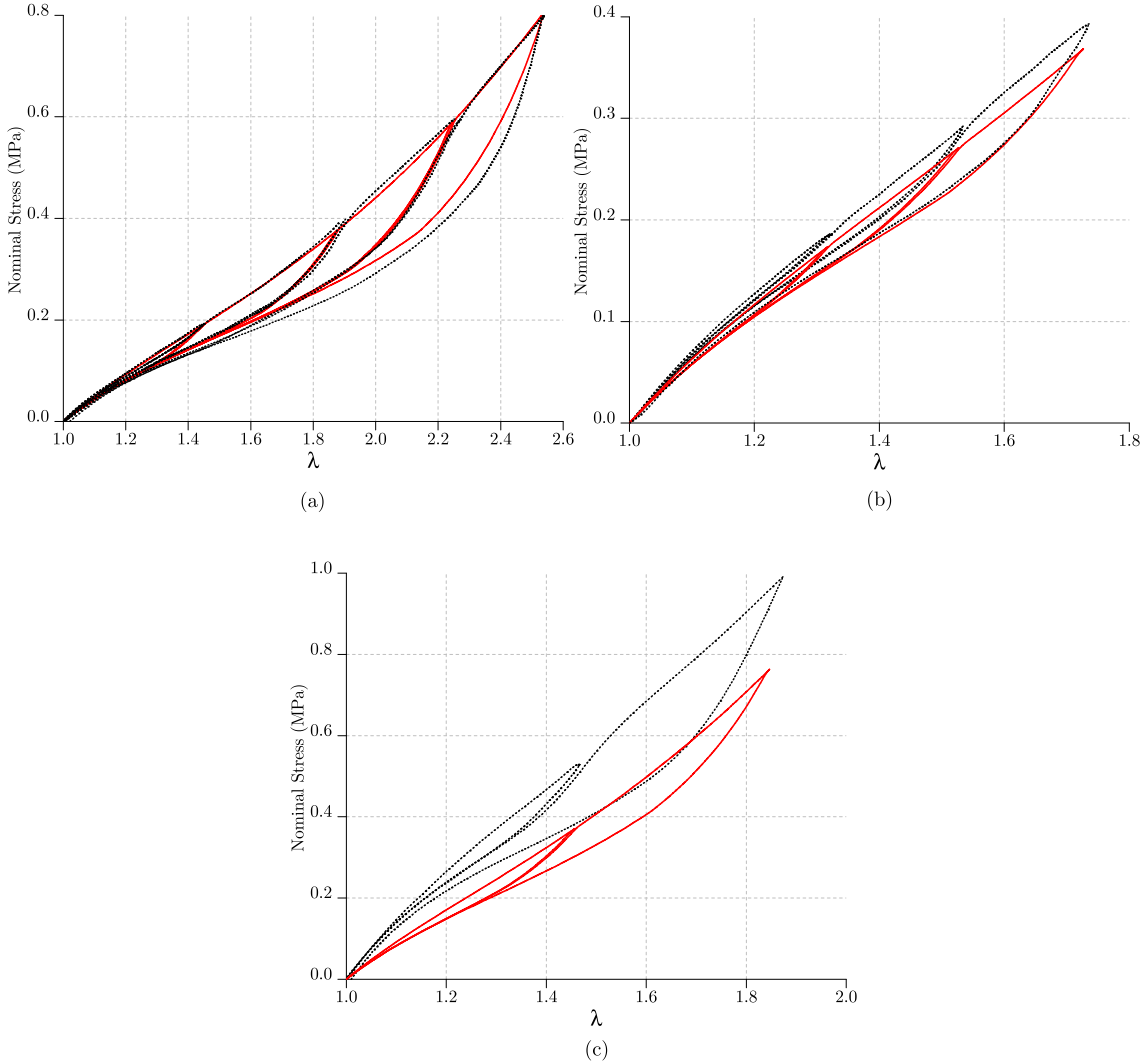
Figure 4.2: Comparison of the model (solid lines) with experimental data from Machado et al. (2010) (dotted lines) for: (a) cyclic uniaxial tensile test, (b) cyclic pure shear test and (c) cyclic equibiaxial test.
