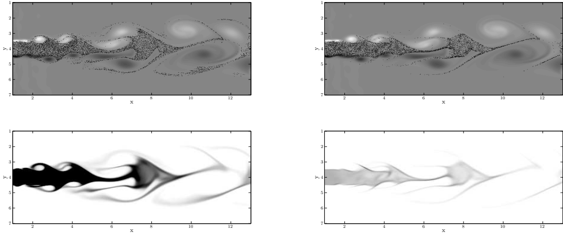
Figure 3.8: Evaporating polydisperse spray at time t = 20 . (Left) Low-inertia droplets with Stokes 0.011 to 0.12, corresponding to diameters from 9 to 30 \mu\text{m} . (Right) High-inertia droplets with Stokes 0.48 to 1.1, corresponding to diameters from 60 to 90 \mu\text{m} . (Top) Lagrangian particle positions with 40,000 particles over gas vorticity. (Bottom) Eulerian number density on a 400 \times 200 \times 5 grid.
