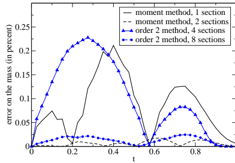
Figure 5.4: Evolution of the error on the mass density relative to its initial value, calculated with the moment method with one or two sections and the multi-fluid method of order 2 with 4 or 8 sections.
