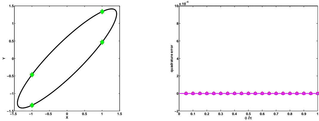
Figure C.2: Quadrature method and associated error for a distribution with r = 0.9 , m_{30} = 0 . Left: set of all velocity abscissas for quadrature in [0, \pi] ; All the nodes are equivalent. Right: reconstructed centered third order moments and error made by the quadrature on these moments: all the centered third order moments stay null, as well as the error made.
