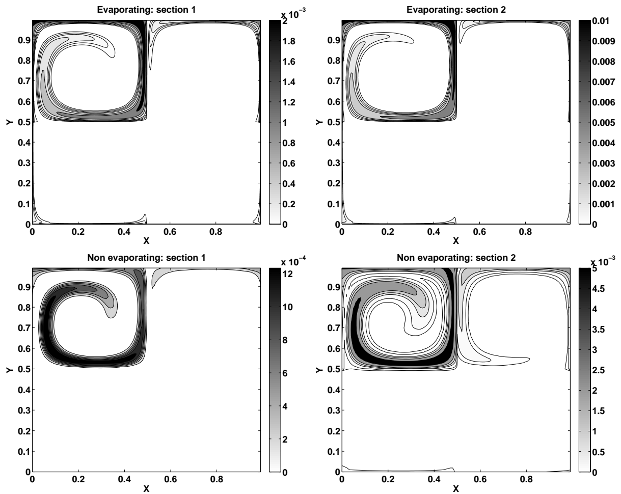
Figure 3.16: Multi-fluid model with ten sections, at time t = 2 . Comparison of the final mass in the first and second section between evaporating and non evaporating case. (Top) Evaporating test case; (left): section one, (right): section two. (Bottom) Non evaporating test case; (left): section one, (right): section two.
