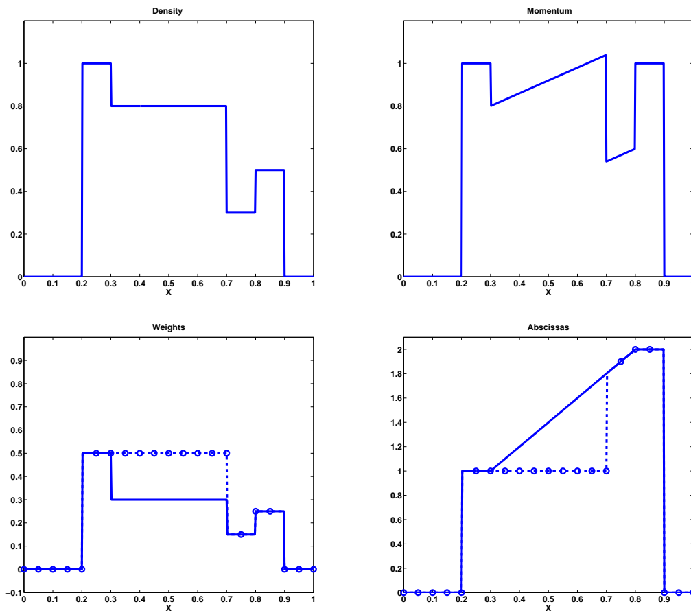
Figure 9.2: Moment dynamics in the context of a smooth transition between areas of null and non null dispersion. Solution at t = 0.2 . Top-left: M_0 . Top-right: M_1 . Bottom-left: weights. Bottom-right: abscissas. The solid line corresponds to (n_1, U_1) , the dashed line with circles corresponds to (n_2, U_2) .
