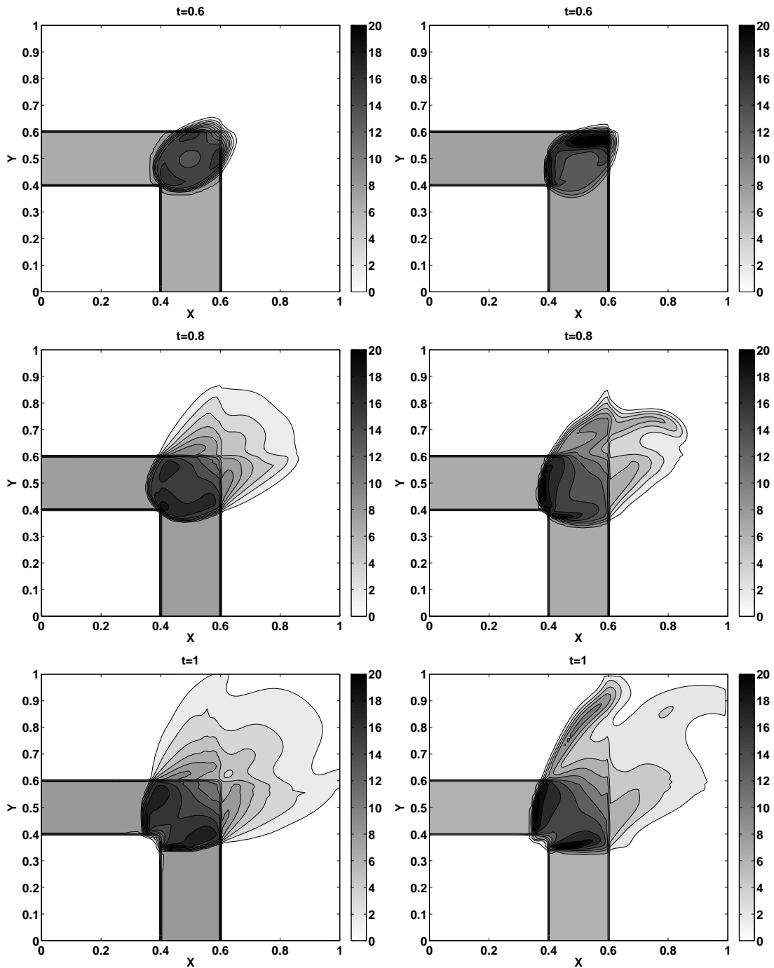
Figure 9.18: Results for collision with \text{Kn} = 1 . (Top) t = 0.6 . (Medium) t = 0.8 . (Bottom) t = 1
