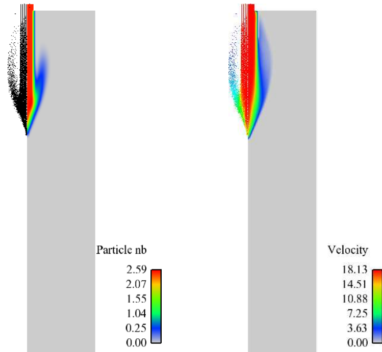
Figure 14.26: Comparison of Lagrangian and Eulerian results for a polydisperse flow made of droplets of D = 20 \mu\text{m} , at time t = 5.10^{-3} \text{ s} . In each figure, the Lagrangian particles are displayed on the left side on the domain, and the Eulerian field on the right side. Left : particle number ( m_0 ); Right : particle velocity.
