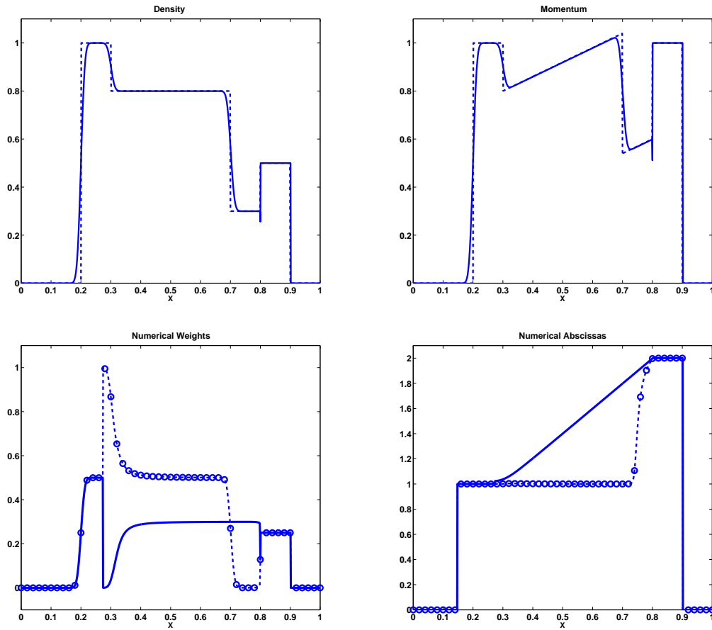
Figure 9.11: Moment dynamics in the context of a smooth transition between areas of null and non null dispersion, at time t = 0.2 . Top-left: M_0 . Top-right: M_1 . The straight lines represent the analytical entropic solution, whereas the dashed lines represent the numerical solution. Bottom-left: weights. Bottom-right: abscissas. The solid line corresponds to the set (n_1, U_1) , and the dashed line with circles to the set (n_2, U_2) .
