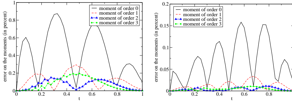
Figure 5.3: Evolution of the error on the moments calculated with the moment method with one section (left) or two sections (right) relative to their initial value.
