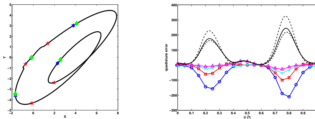
Figure C.4: Quadrature method and associated error for a distribution with r = 0.9 , m_{30} = 1 . Left: set of all velocity abscissas for quadrature in [0, \pi] ; the blue squares are the set of nodes which minimizes err1 , the red stars are the set of nodes which minimizes err2 , and the green diamonds are the set of nodes which minimizes err3 . Right: reconstructed centered third order moments: m_{30} (blue curve with circles), m_{21} (red curve with squares), m_{12} (cyan curve with crosses), m_{03} (magenta curve with triangles); error made by the quadrature on these moments: err1 (solid black line), err2 (dashed dotted black line), err3 (dashed black line).
