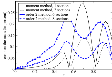
Figure 5.7: Evolution of the error on the mass density relatively to its initial value, calculated with the moment method with one or two sections and the multi-fluid method of order 2 with 6 or 8 sections.
