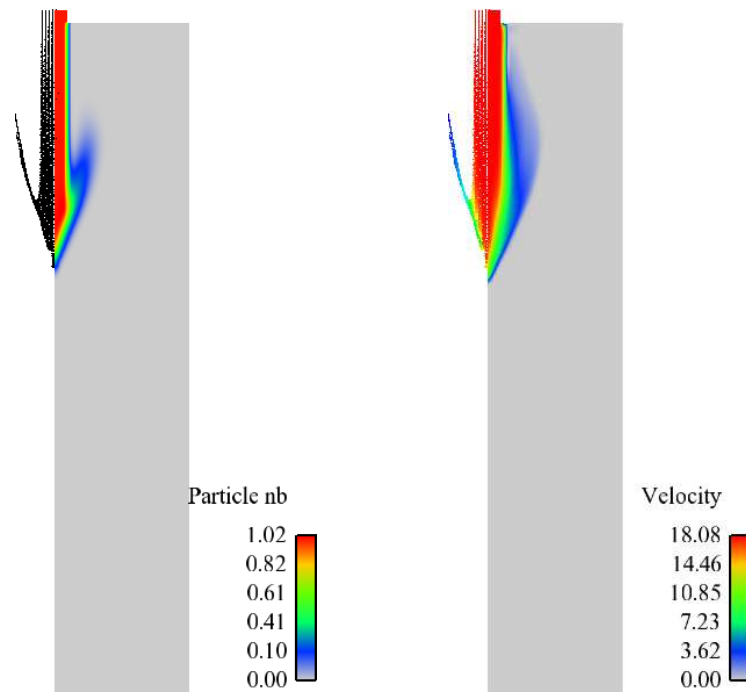
Figure 14.23: Comparison of Lagrangian and Eulerian results for a monodisperse flow made of droplets of D = 20 \mu m , at time t = 5 \cdot 10^{-3} s . In each figure, the Lagrangian particles are displayed on the left side on the domain, and the Eulerian field on the right side. Left : particle number ( m_0 ); Right : particle velocity.
