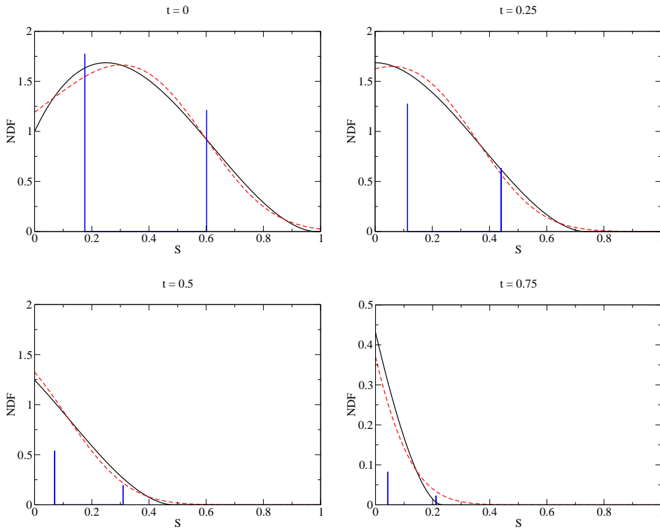
Figure 5.2: Smooth NDF (solid), ME reconstructed NDF obtained with the moments computed with the moment method with 1 section and 4 moments (dashed line) and corresponding peaks, at times t = 0 , t = 0.25 , t = 0.5 and t = 0.75 .
