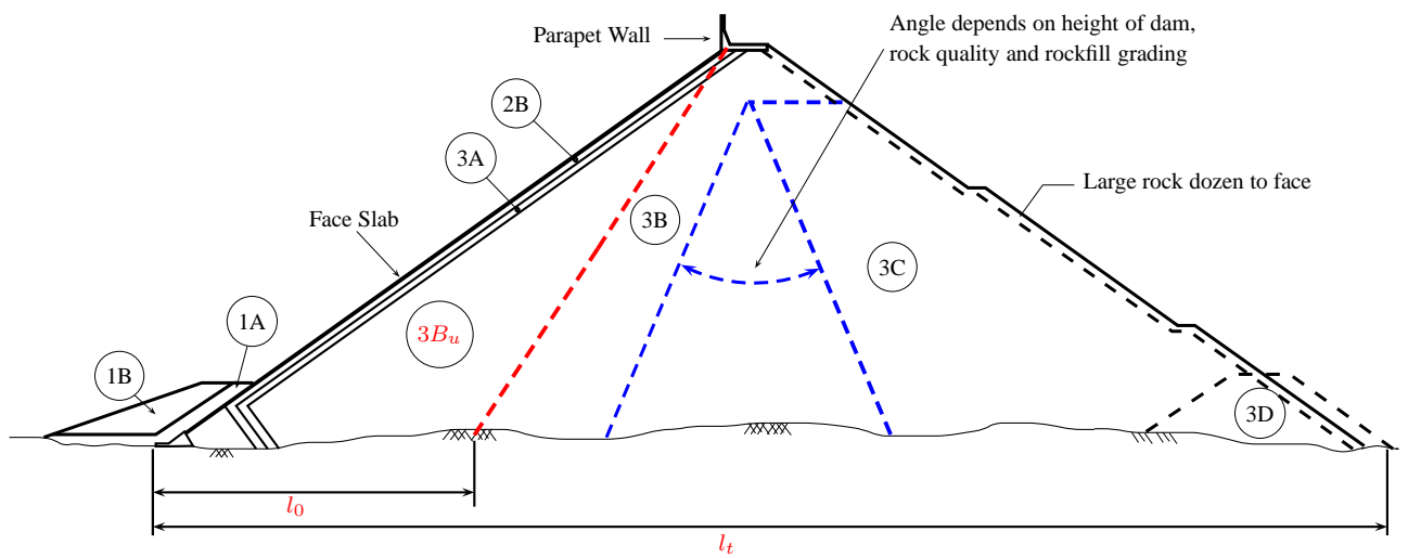
Figure 7.10: Proposition for a variation of the CFRD zoning.
