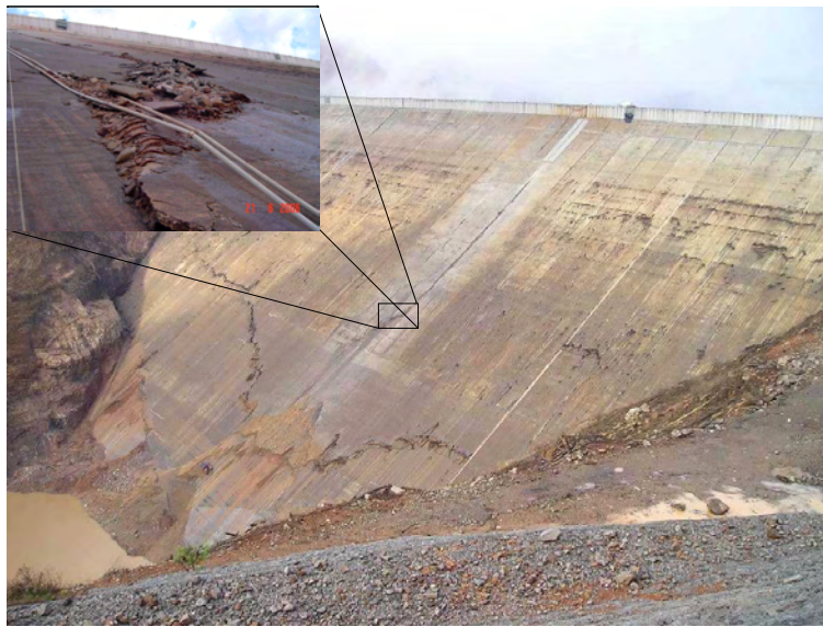
Figure 1.5: Failure of concrete slabs in Campos Novos rockfill dam, after Pritchard (2008).
