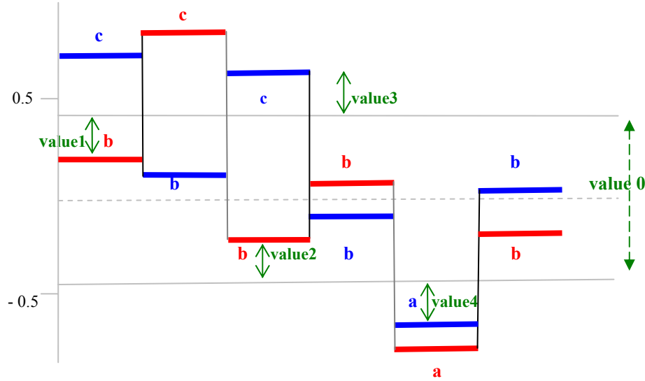
Fig. 5.3. The PAA representation of two time series: S1 = cbc bab (boldface, blue) and S2 = bcb bab (boldface, red). The solid arrows show the ignored distances and the dashed arrow shows the only distance considered by MINDIST : dist(a, c) = value0 (0.86)
