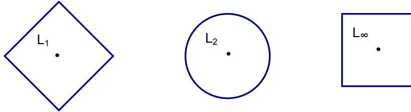
Fig. 2.1. Minkowski distance for L_1 , L_2 , and L_\infty
