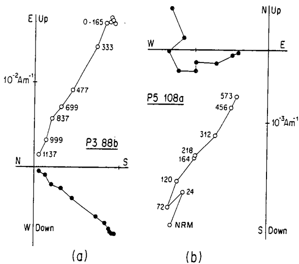
Fig. 6. Chemical demagnetization curves. Cumulative time of leaching is indicated in hours. Same conventions as in Fig. 5.
