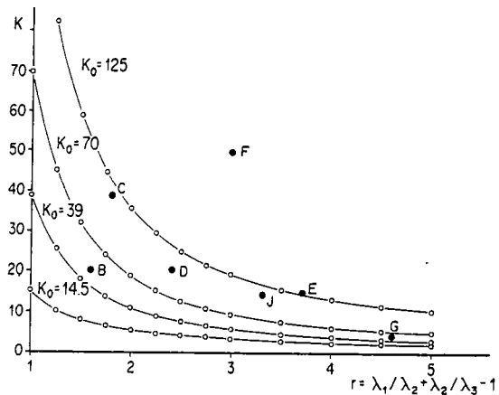
Fig. 8. Curves of modeled behaviour of Fisher's k parameter as a function of strain intensity r [41]. Black dots are real parameters of the group I sites.
