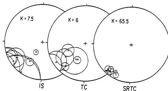
Fig. 13. Group II: site-mean directions with their circles of confidence. Same abbreviations and conventions as in Fig. 12.
