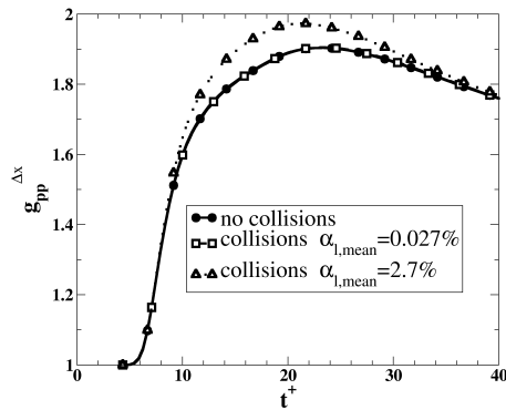
Figure 6. Preferential particle concentration time evolution of MEF simulations: without collisions (circle), with collisions at \alpha_{l,mean}=0.027\% (square), with collisions at \alpha_{l,mean}=2.7\% (triangle up).
