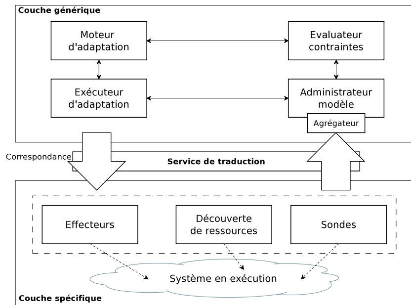
FIGURE 3.6 – Le canevas de Rainbow
