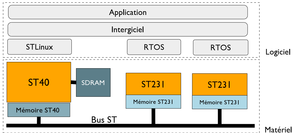
FIGURE 7.1 – Plate-forme IDTV
