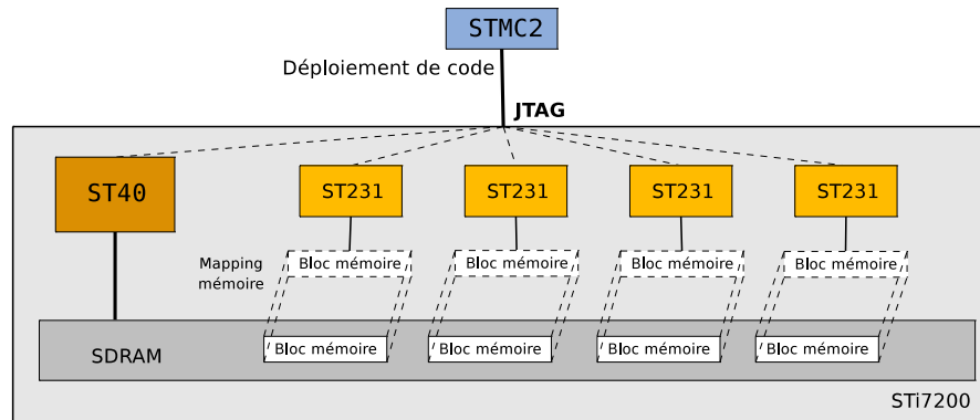
FIGURE 6.1 – Plate-forme STi7200
