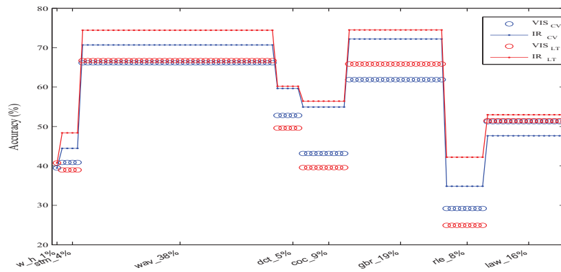
(b) Accuracy obtained for different FVs (comprising only families of features) from visible (circle) and infrared (line) domains, evaluated by 1-NN using 10f-CV (blue) and LT (red) for the classification problem with 8 classes of objects
