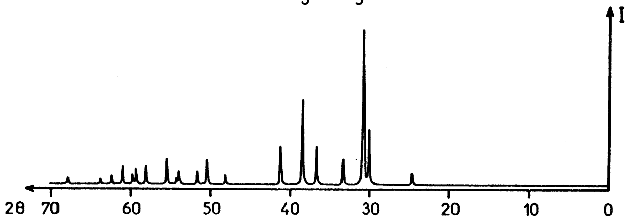
(c) \text{Sr}_3\text{SiO}_5
