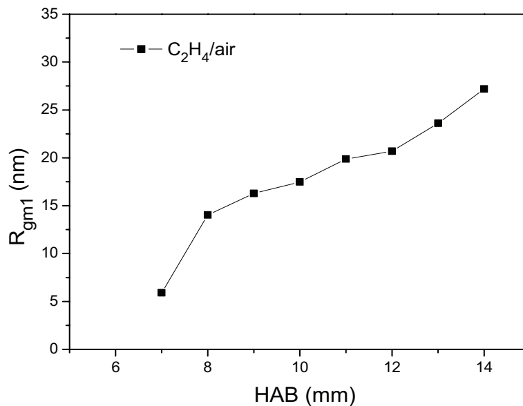
Fig. III.2.9: Radius of gyration versus the height above the burner for C_2H_4/air flame at an equivalence ratio of 2.34 ( T_{ini} = 300\text{ K} , P_{ini} = 101.3\text{ kPa} ).
