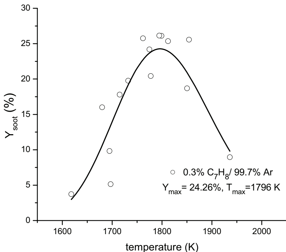
Fig. IV.1.17: Dependence of the soot yield from the temperature. 0.3% toluene in Argon
