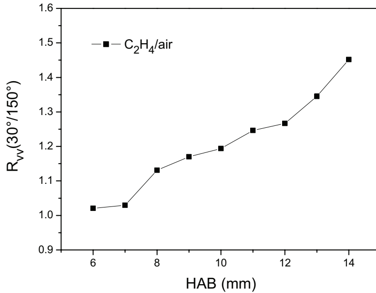
Fig. III.2.8: Dissymmetry ratio versus the height above the burner for C_2H_4/air flame at an equivalence ratio of 2.34 ( T_{ini} = 300\text{ K} , P_{ini} = 101.3\text{ kPa} ).
