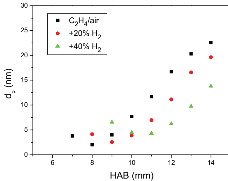
Fig. III.2.20: Soot particle diameter versus the height above the burner for the three flames ( C_2H_4/air , C_2H_4/20\%H_2/air and C_2H_4/40\%H_2/air ; see Table II.2.1).
