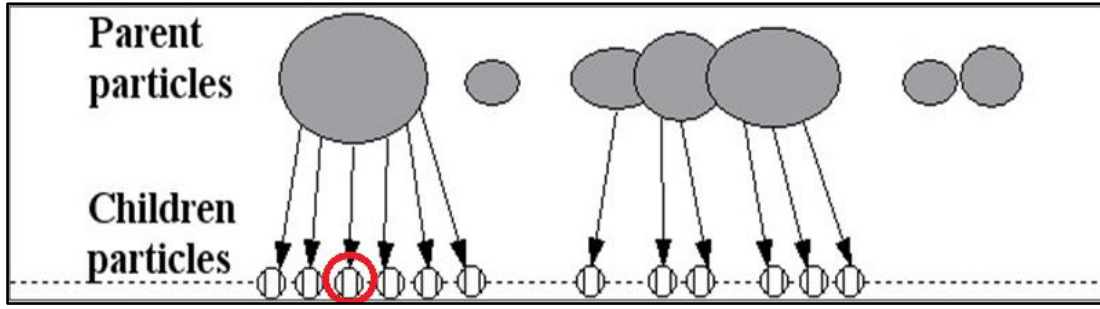
Figure 4-10: Weight-based deterministic resampling. Parent particles (gray circles) give birth to a number of children particles (white circles) proportional to their weights (size of particle). A child of the highest weight parent particle will not be diffused randomly in the prediction step in order to avoid losing the currently best estimation in case of sample depletion.
