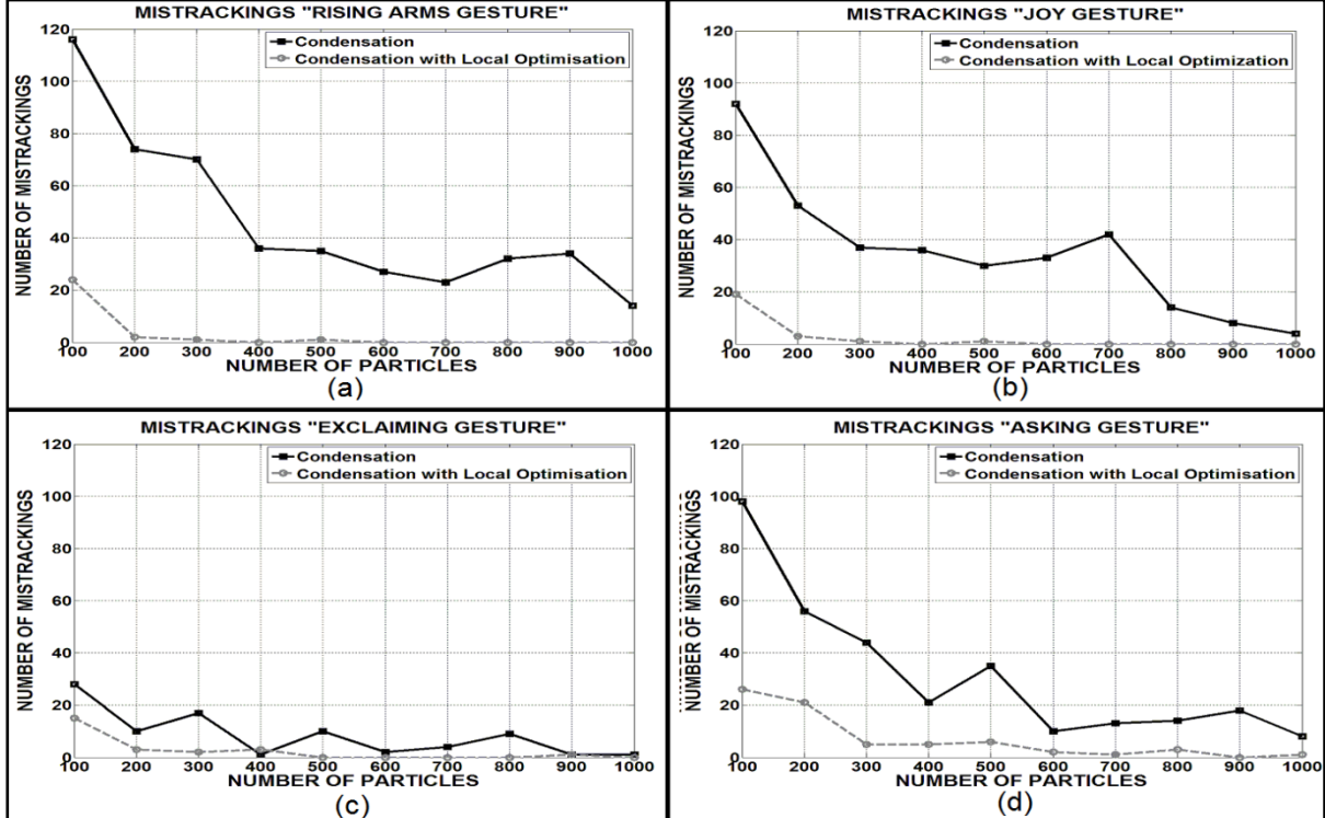
Figure 4-17: Experimental results showing the robustness contribution of the proposed local optimization (dashed gray line) with respect to the particle filter algorithm (black line). The abscissas are the number of particles and ordinates is the number of mistrackings obtained for all frames of the video sequence.
