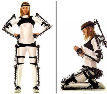
Figure 2-2: A mechanical exoskeleton suit for motion capture (Gypsy7, 2010).
