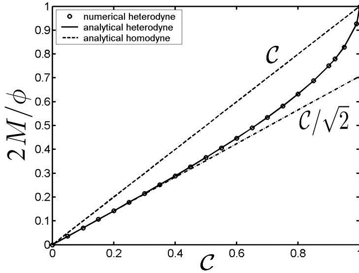
Figure 5.20: Comparison of the Mach Zehnder interferometer and the heterodyne detection. Measurement strength as a function of contrast C for the lossy Mach-Zehnder interferometer and for the heterodyne measurement.
