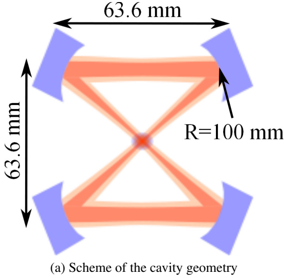
Figure 3.4: The crossed cavity configuration
