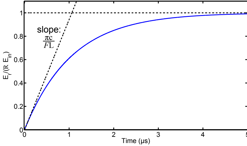
Figure 3.27: The cavity as a low pass frequency filter
