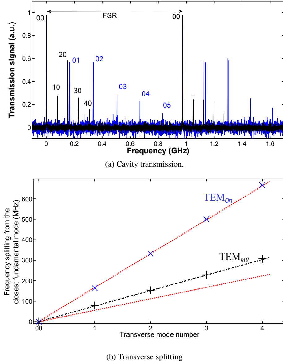
Figure 3.15: Transverse mode splitting
