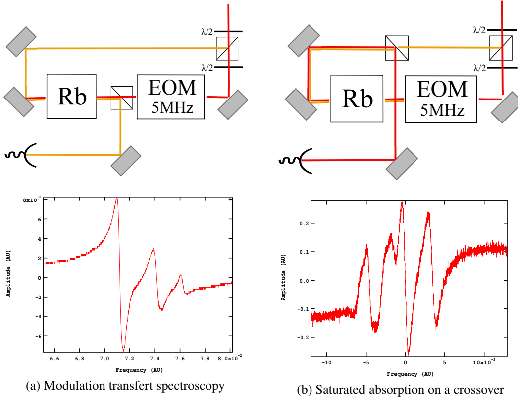
Figure 2.5: Saturated absorption
