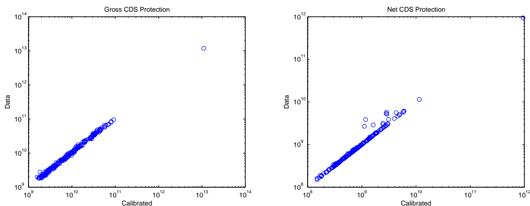
Figure V.7: Calibration to DTCC Data [130]
