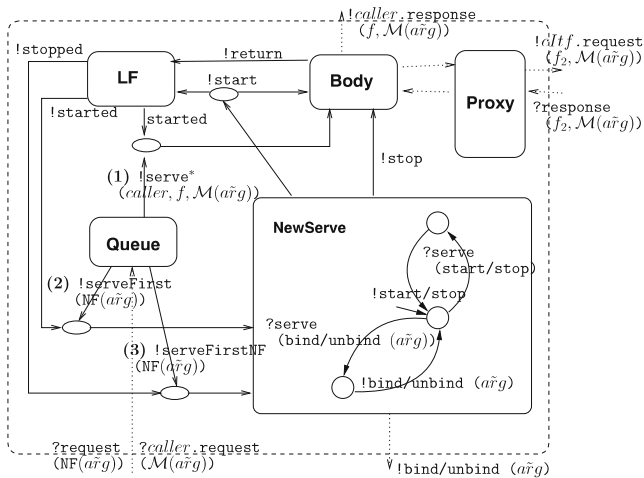
Fig. 8 Behaviour model for a GCM/ProActive primitive
