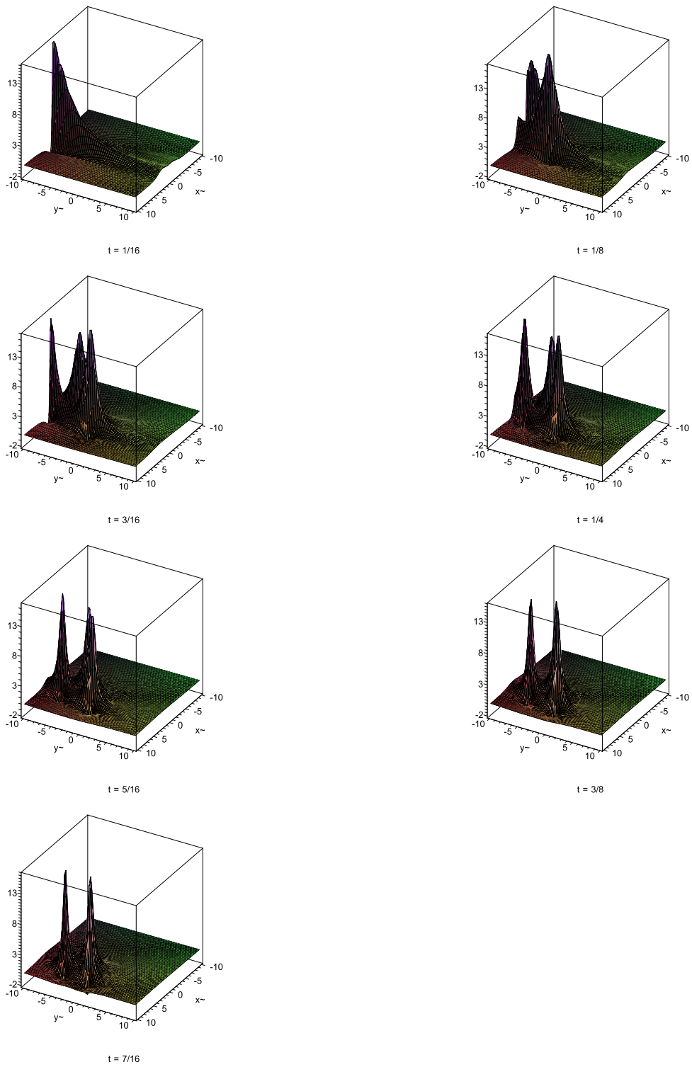
Figure 12: Solution of CKP with \varphi_4 = \frac{5+\sqrt{5}}{96} \sqrt{10 - 2\sqrt{5}}
