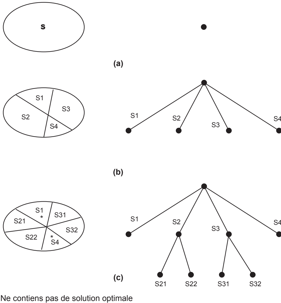
Figure 5.7 – Principe de la Méthode du branch and bound.
