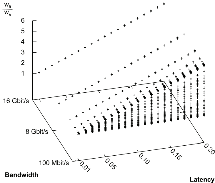
Figure 6.10: GTNetS throughput of flow A over flow B \left(\frac{\rho_A}{\rho_B} = \frac{w_B}{w_A}\right) . Observing GTNetS we conclude that the problem with the model is bad instantiation.
