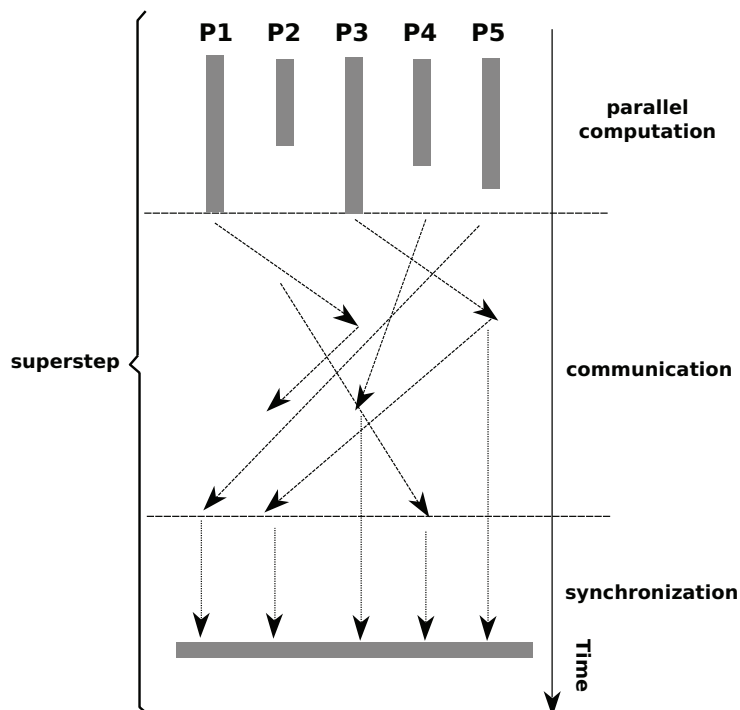
Figure 3.4: A superstep for the BSP model is a set of parallel computation followed by one communication and one synchronization phase.
