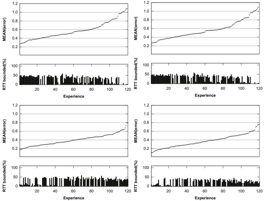
Figure 6.27: Mean error when \cong 50\% of flows are limited by latency.
