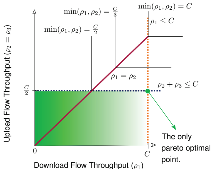
Figure 6.18: Ignoring control traffic the Max-Min algorithm finds the only available Pareto optimal point.
