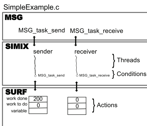
Figure 4.8: Internal simulation workflow. Actual process are trapped by simulation actions (fake computation or communication). At this point, the simulation kernel must decide based on a model which action finishes first.
