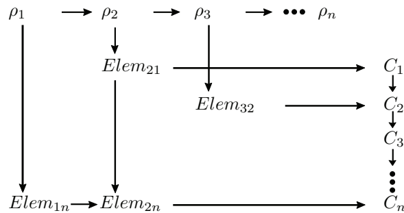
Figure 5.2: Data structure used to store the Max-Min system. Besides the list of constraints and variables there are several elements connecting the constraints used by one specific variable.
