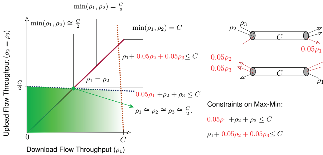
Figure 6.19: Adding control traffic in opposite direction Max-Min is able to improve TCP modeling. When adding control traffic each point on the edge of the validity zone is a Pareto optimal point, i.e., a possible solution. So, with the full-duplex model Max-Min is capable of correct modeling ack compression, i.e., \rho_1 \cong \rho_2 \cong \rho_3 \cong \frac{C}{2} .
