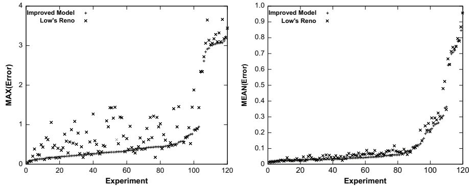
Figure 6.30: Max error (left) and mean error (right) compared to Low's Reno model with non-modified test set.
