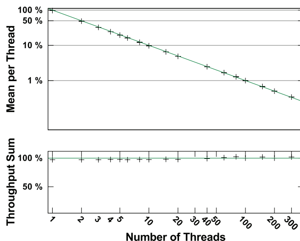
Figure 6.1: CPU model (continuous line) in comparison with real experiments (crosses) when varying the number of concurrent threads. The simple CPU model is accurate to model processing time even when the host is shared by several independent threads.
