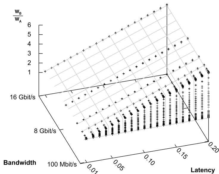
Figure 6.11: GTNetS sharing \frac{\rho_A}{\rho_B} (crosses) and the approximated Max-Min weight (surface) when \gamma fits GTNetS behavior, i.e., \gamma = 20537.14 .
