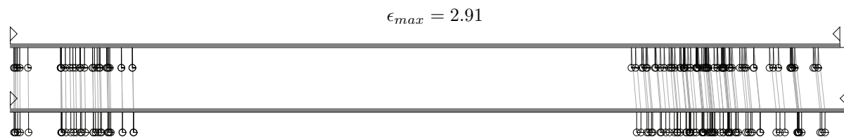
Figure 6.28: Simulation timeline indicating the moment when each flow finishes. The top timeline was obtained with GTNetS while the bottom one with SimGrid improved model. We draw a line corresponding flows in the model and GTNetS. In this case the maximum error is seen at the very beginning due to small finish time of the first finishing flow.
