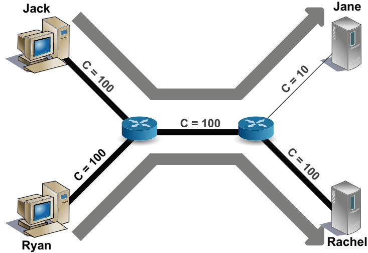
Figure 5.1: Example of how the simple sharing model used in OptorSim [11] is incapable of capturing the network behavior. In this example the top flow gets a working rate of 10 while the bottom flow gets a working rate of 50. At the end we have that only 60% of the central link is used.
