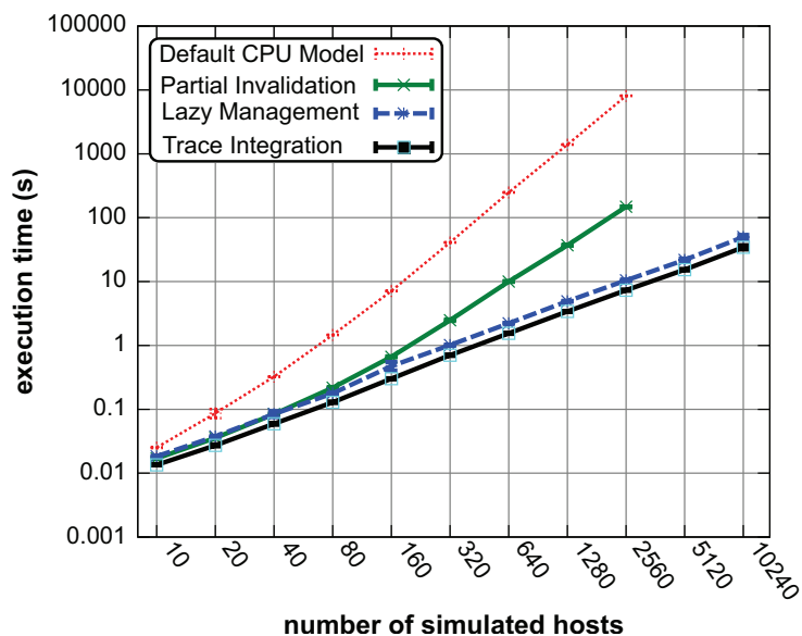
Figure 7.3: Simulation time as a function of number of hosts in logarithmic scale without using trace files . Lazy action management improves the simulator speed significantly and trace integration does not affect the system performance without availability traces.
