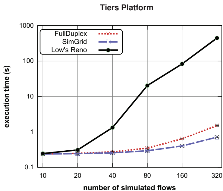
Figure 7.8: Performance of SimGrid original model versus full-duplex model and Low's Reno model performances for a 50-node's Tiers platform . The performance with full-duplex model is very close to the original model while Reno's performance is the worst one.
