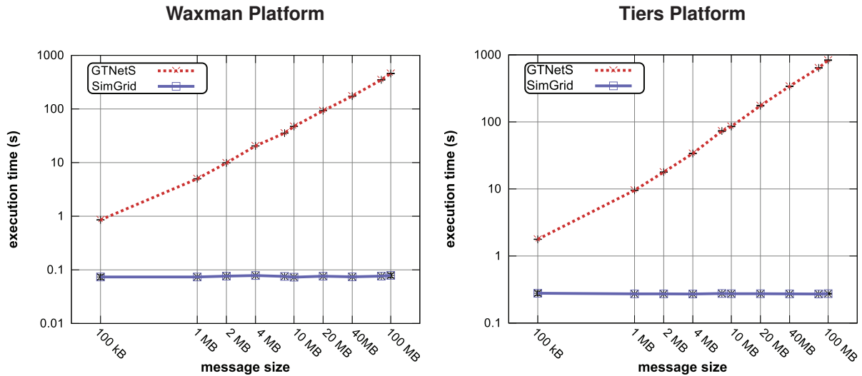
Figure 7.6: SimGrid versus GTNetS response time when varying the size of messages for two 50-node platforms Waxman (left) and Tiers (Right). Notice that GTNetS performance depends on the size of message while SimGrid performance, as expected, is independent of message sizes.
