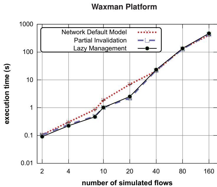
Figure 7.9: Performance of SimGrid default network model versus partial invalidation and lazy management with a 50-node's Waxman platform . With lazy management and partial invalidation the execution time is improved for small contention scenarios.
