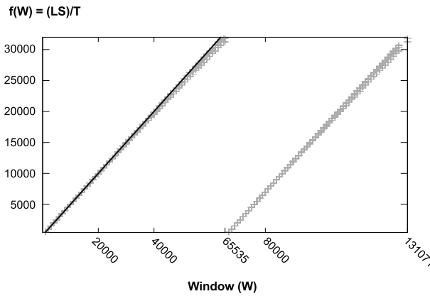
Figure 6.3: Transmission throughput as function of TCP window for GTNetS values (crosses) in comparison to SimGrid model (continuous line). This results reinforces that connection throughput is often limited by the round trip time. Moreover, this figure points out that two times the latency ( 2L ) is a good approximation for RTT.
