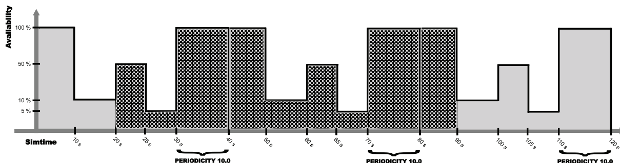
Figure 7.2: Integrating availability trace histograms one is able to advance the simulation to useful actions.
