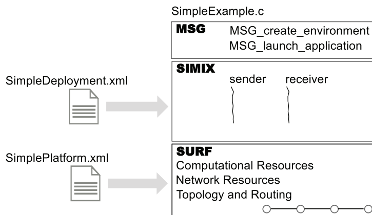
Figure 4.7: SimGrid internals after initialization. One actual thread is created in SIMIX for each user process. A representation of the network topology is created inside the simulation kernel.
