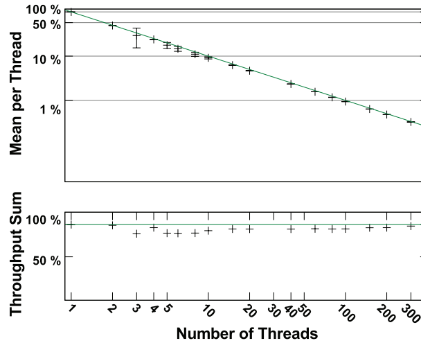
Figure 6.2: CPU model (continuous line) in comparison with real experiments (crosses) when threads are sharing the same memory space . The simple CPU model is accurate, however, it is yet slightly less accurate than with independent threads.
