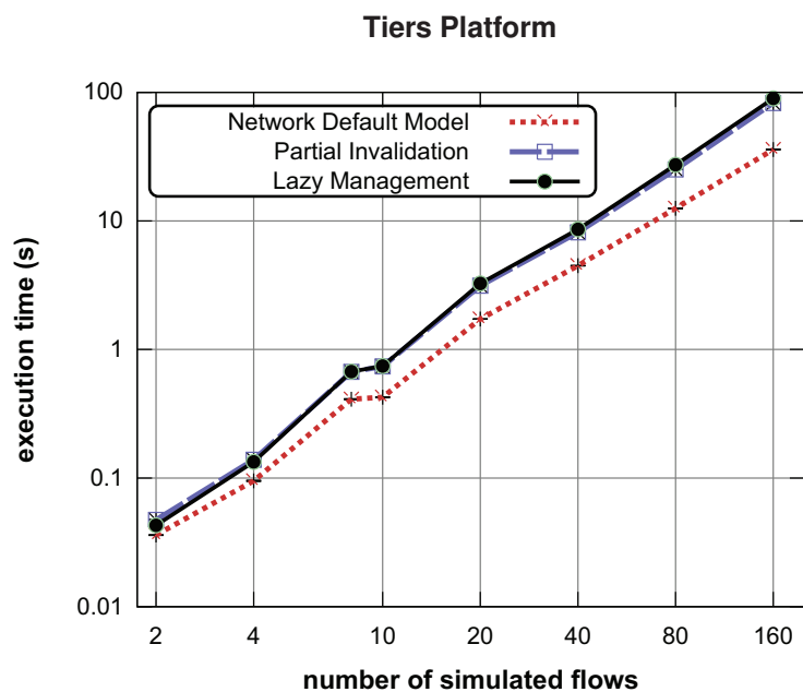
Figure 7.10: Performance of SimGrid default network model versus partial invalidation and lazy management with a 50-node's Tiers platform . With lazy management and partial invalidation the execution time follows the same complexity .
