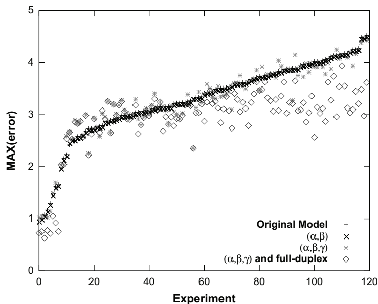
Figure 6.24: Maximum error when avoiding latency limited flows.
