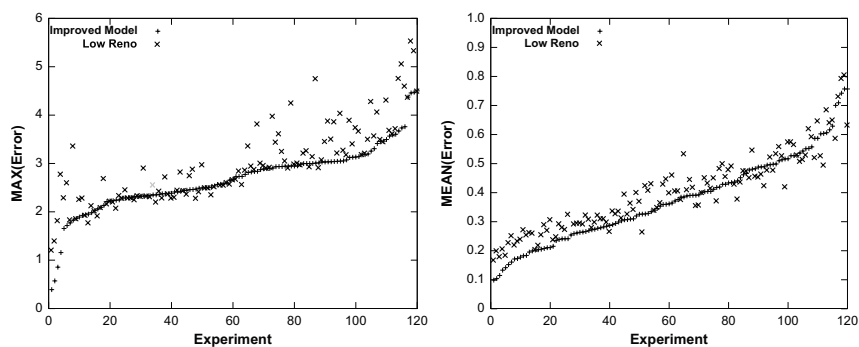
Figure 6.32: Max error (left) and mean error (right) compared to Low's Reno model when \cong 50\% of flows are limited by round trip time.
