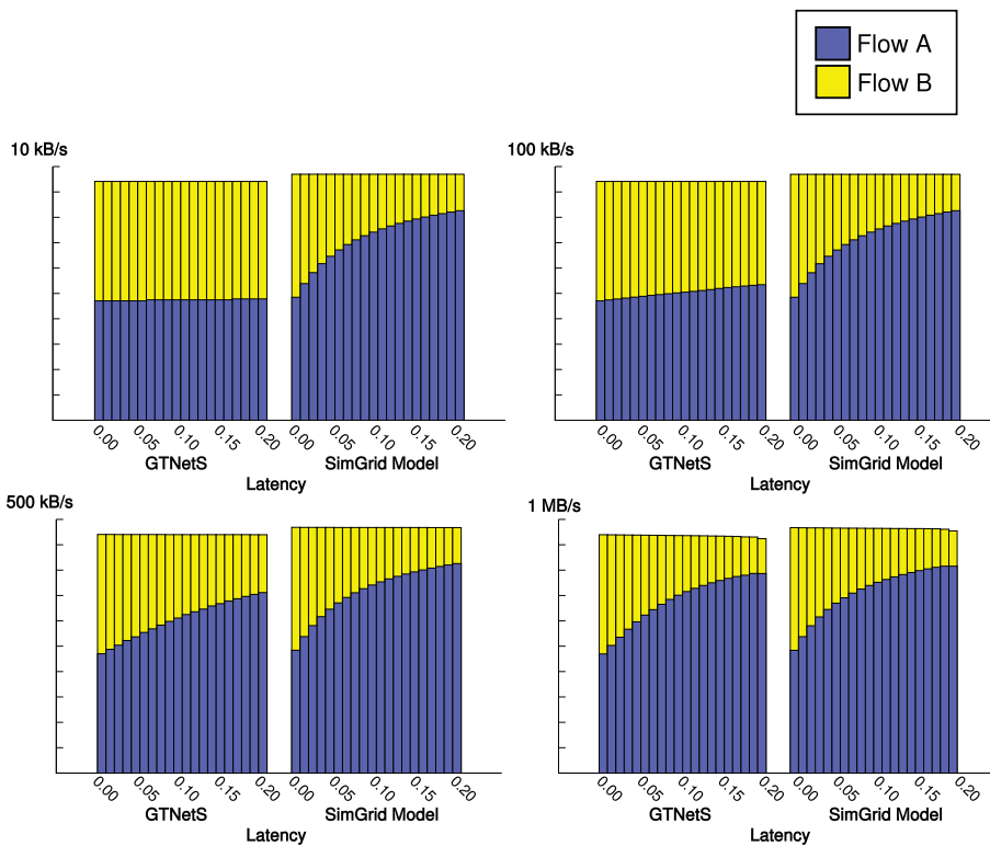
Figure 6.9: GTNetS throughput sharing result in comparison with SimGrid sharing model. SimGrid models is inaccurate when bandwidth for small bandwidth values.
