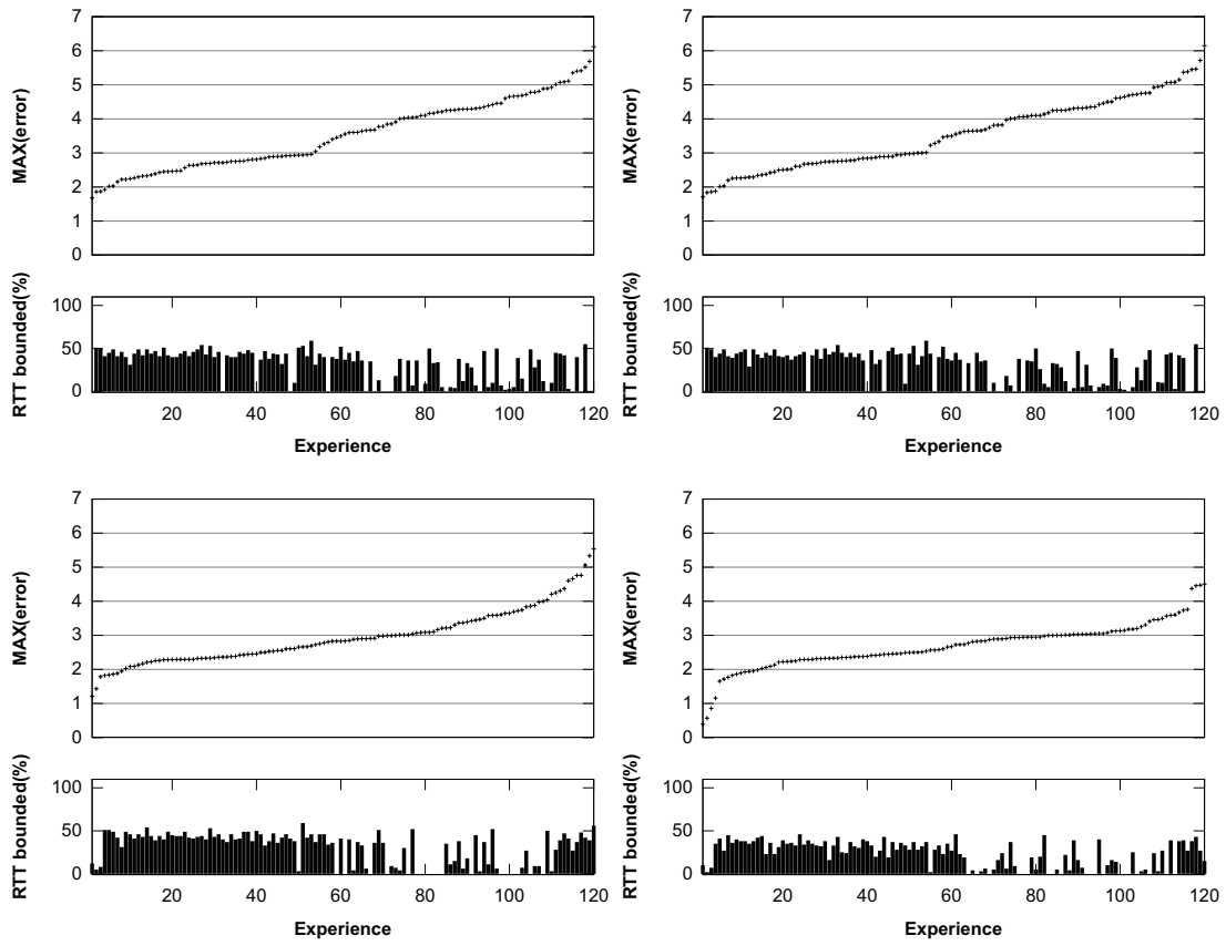
Figure 6.26: Max error when \cong 50\% of flows are limited by latency.
