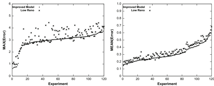
Figure 6.31: Max error (left) and mean error (right) compared to Low's Reno model when bounded by bandwidth.
