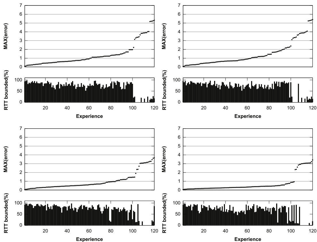
Figure 6.22: The maximum error after several improvements using random topologies. The model after improvements, bottom-right, has improved accuracy.
