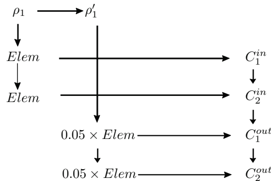
Figure 6.17: Sparse Max-Min representation when using the full-duplex model. One smaller data flow \rho'_1 is created in opposite direction of the main flow \rho_1 . The constraints are also doubled to reflect the possibility of using full power in both directions.
