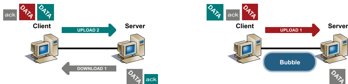
Figure 6.16: In TCP ack compression is a common phenomenon. When this phenomenon happens ack packets get stuck (or compressed) in the client sending queue forcing the download flow to use only 50% of available bandwidth.
