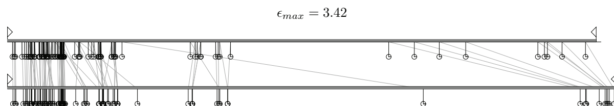
Figure 6.29: Flow termination (marks) timeline obtained with the GTNetS (top) and SimGrid improved model (bottom). Yet, in this case the maximum error is representative as measure.
