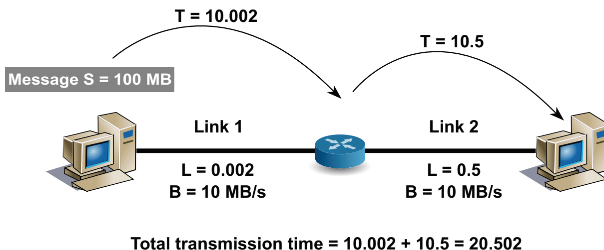
Figure 3.2: Store & forward approaches does not reflect the behavior of TCP for multiple links even when contention is neglected.
