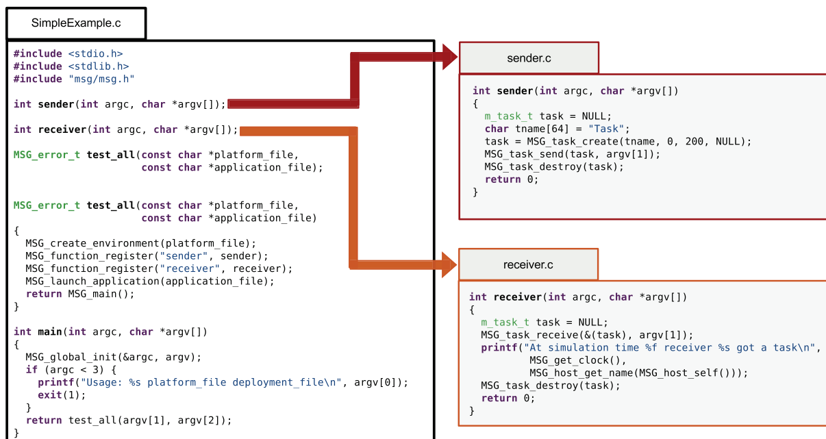
Figure 4.2: A simple SimGrid application model.
