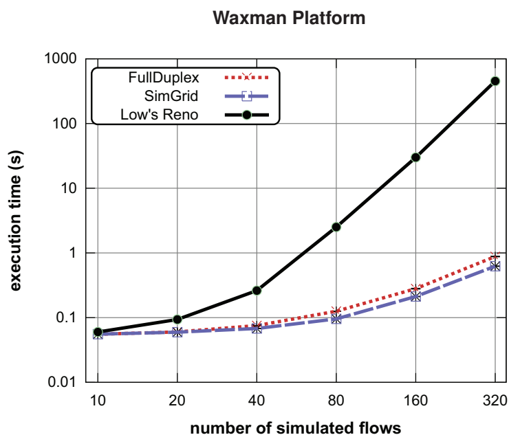
Figure 7.7: Performance of SimGrid original model versus full-duplex model and Low's Reno model performances for a 50-node's waxman platform . The performance with full-duplex model is very close to the original model while Reno's performance is the worst one.
