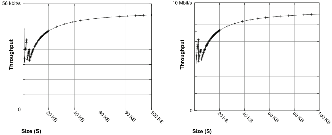
Figure 6.6: Throughput of short flows as a function of size for two network links, 56 kbit/s (left) and 10 Mbit/s (right). The slow start phase affects throughput of small messages but stabilizes for messages over 100 KB.
