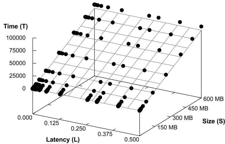
Figure 6.4: SimGrid model transmission time (surface) in comparison with GTNetS (points) in a 56 Kbit/s link. Time can be well estimated as a linear function of size, bandwidth and latency when limited by link bandwidth.
