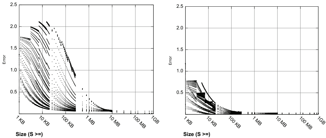
Figure 6.7: Error \epsilon of original model (left) and error after fitting GNetS results (right). Errors are significantly reduced after improvements.
