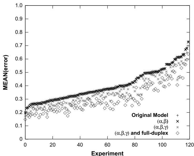
Figure 6.25: Mean error when avoiding latency limited flows.
