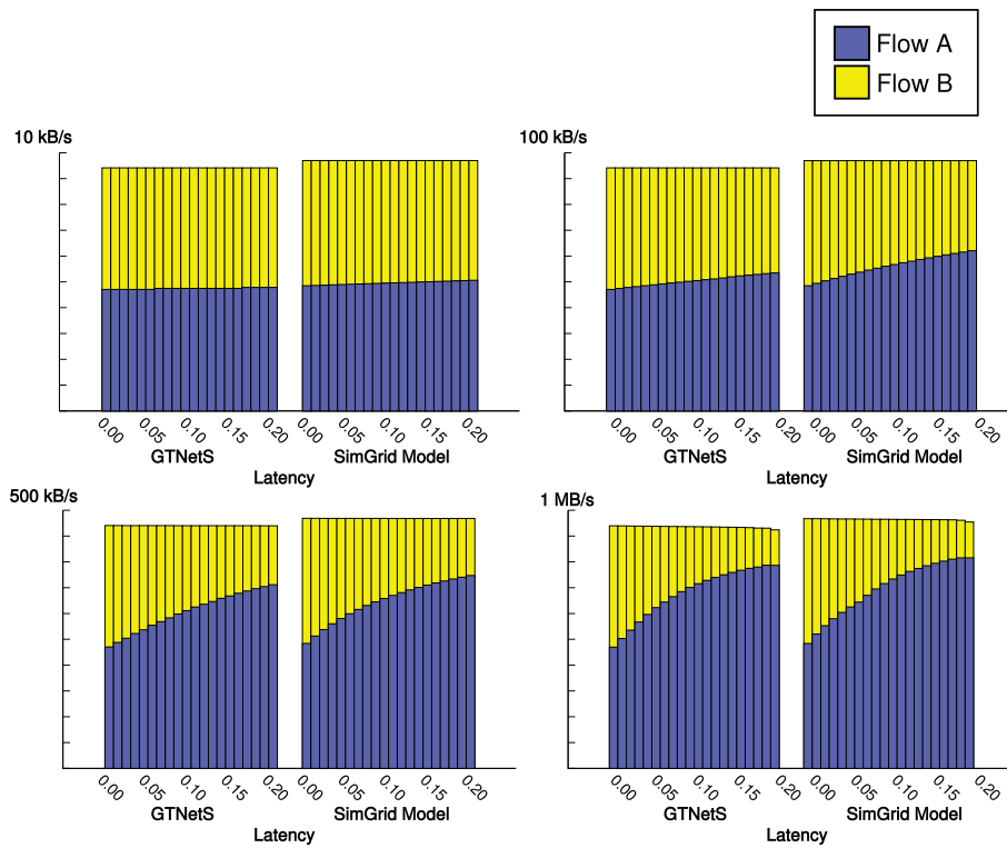
Figure 6.12: GTNetS bandwidth share in comparison with SimGrid model after fitting GTNetS. Resulting share is improved when flows are limited by bandwidth.
