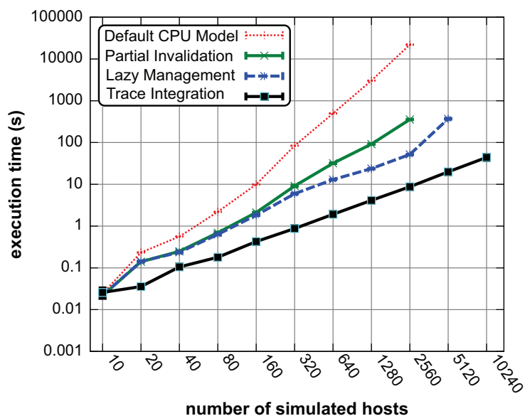
Figure 7.4: Simulation time as a function of number of hosts in logarithmic scale using trace files . Trace integration can significantly improve simulation speed in this case.
