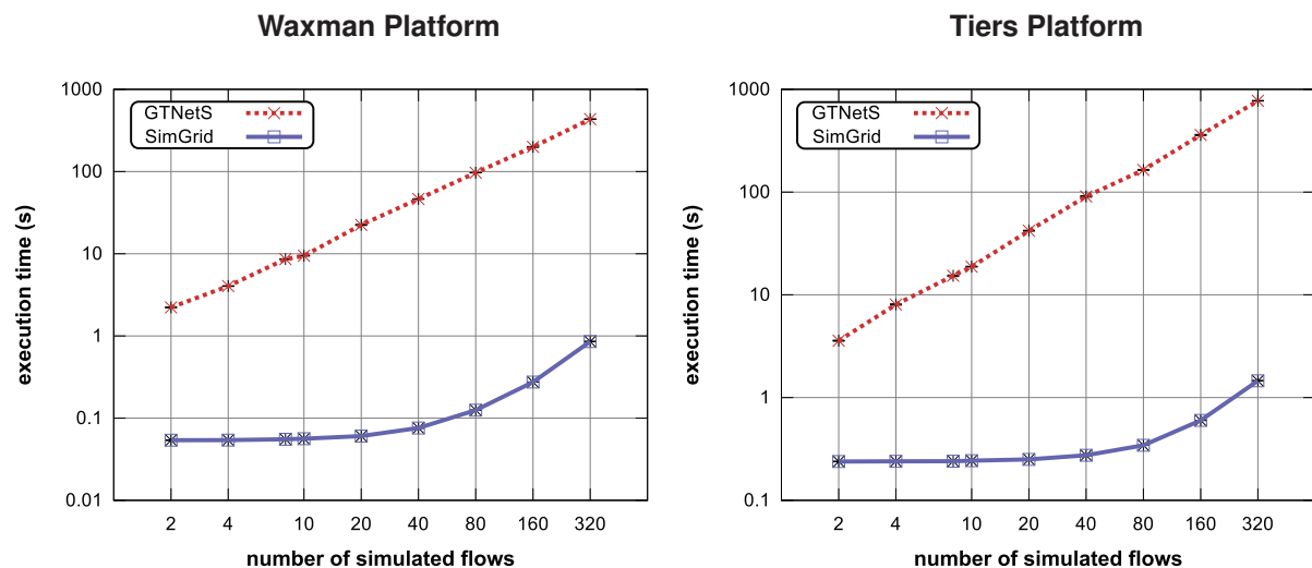
Figure 7.5: SimGrid versus GTNetS response time when varying the number of simulated flows for two 50-node platforms Waxman (left) and Tiers (Right). Notice that GTNetS is much slower than SimGrid in spite of results being very close as shown in Table 7.1.
