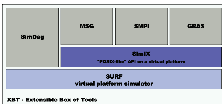
Figure 4.5: SimGrid architecture.
