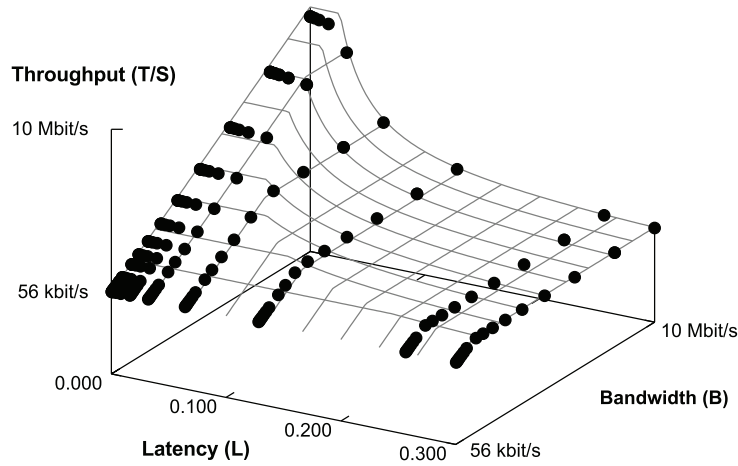
Figure 6.5: Transmission throughput of SimGrid model (surface) in comparison with GTNetS' throughput (points). When bandwidth is high flows become eventually limited by latency.
