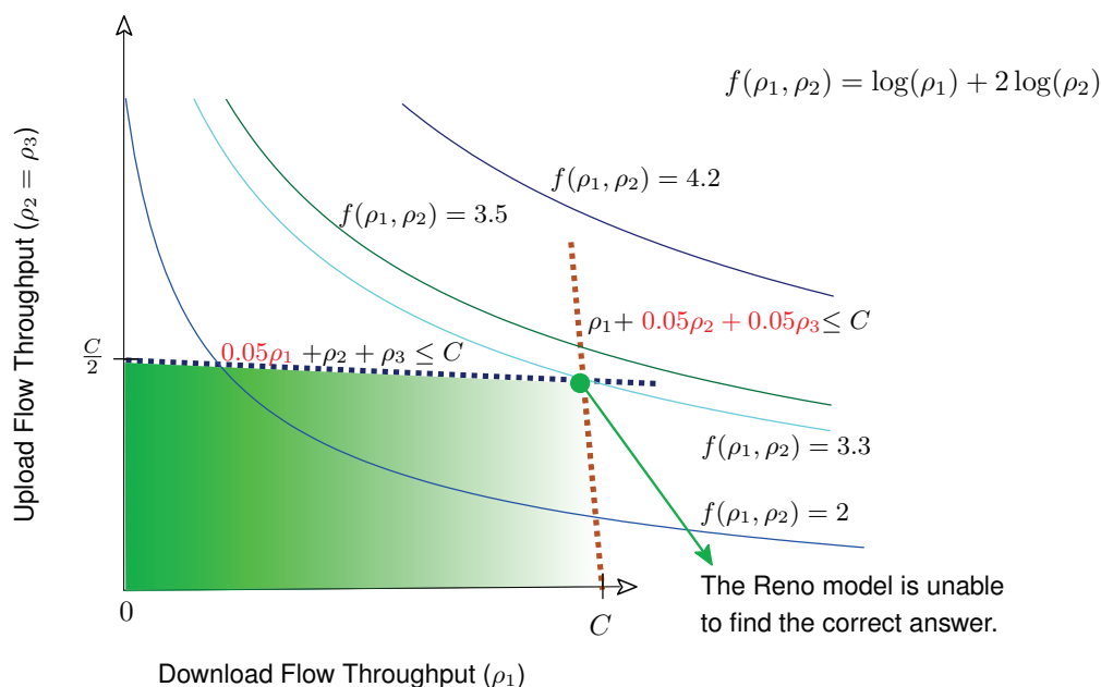
Figure 6.33: Representation of Reno model for a simple full-duplex scenario of one download and two uploads. Adding control traffic is helpless to Reno model since it still choose the Pareto optimal point in the corner.
