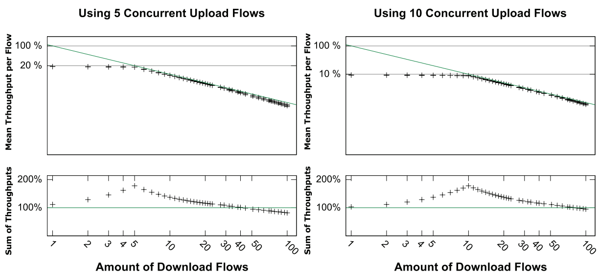
Figure 6.15: Throughput with concurrent download and upload flows.
