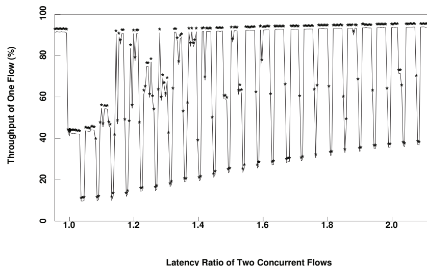
Figure 8.1: Phase effect example. The throughput of one flow, when two concurrent flows present slightly different latencies, may be significantly penalized. This happens because DropTail may privilege flows depending on the frequency that packets arrive.
