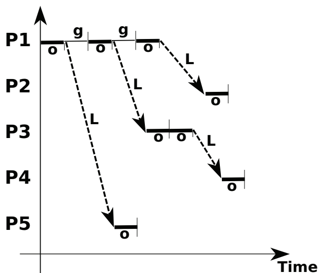
Figure 3.1: In the LogP model communication is more detailed. Before sending or receiving a message one waits for the overhead ( o ), the time taken to transmit is dictated by the latency ( L ) and between consecutive transmissions a gap ( g ) is respected.
