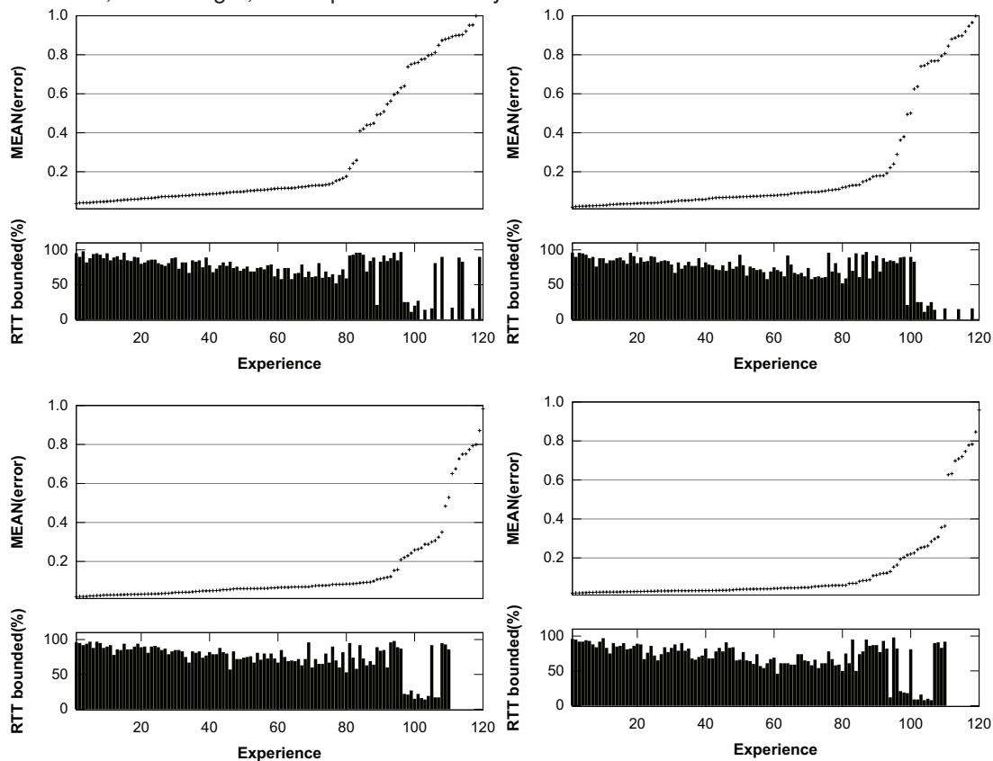
Figure 6.23: Mean error using after several improvements using random topologies. Although the mean error is improved, the mean error improvements are less significant.
